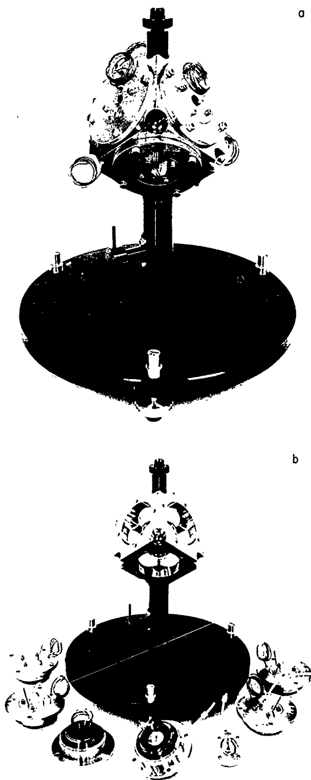
Figure 11. Six-pad spinning sphere, assembled and disassembled
