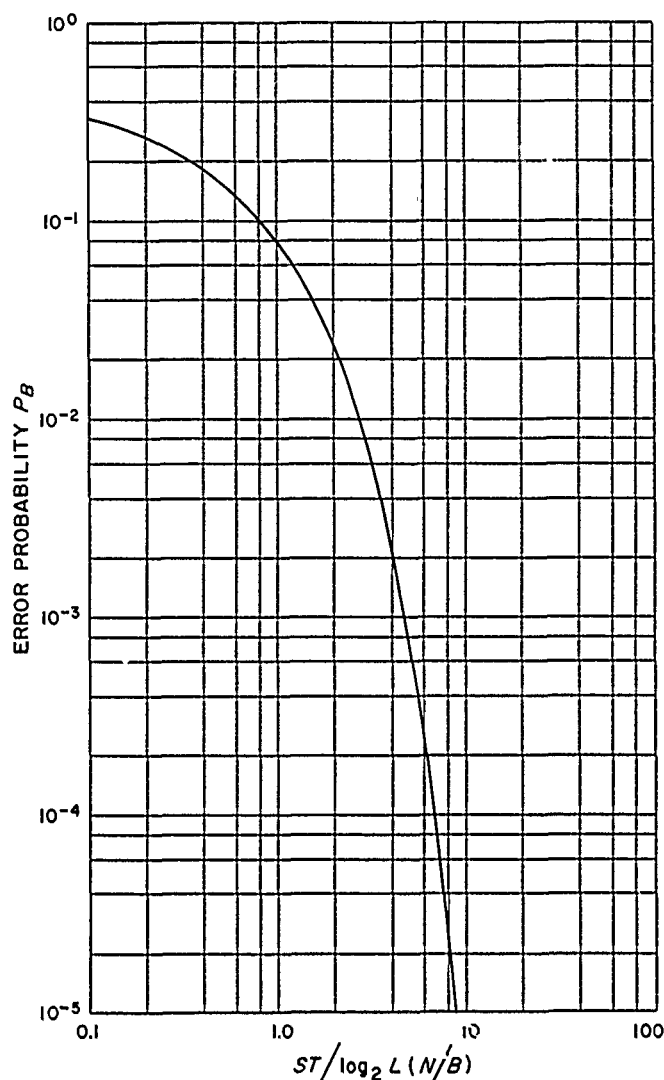
Figure 60. Bit detection error probability for PCM, nonredundant codes
