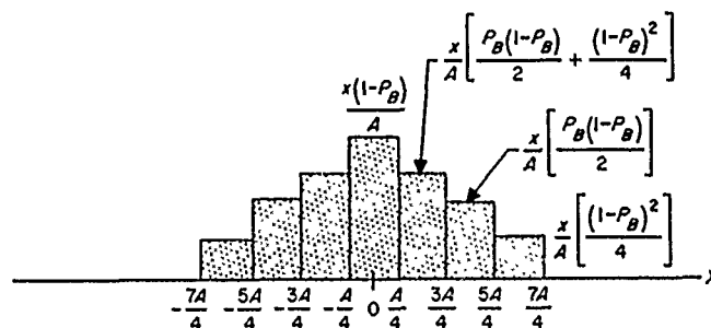
Figure 62. Probability density of errors for nonredundant PCM, four levels
