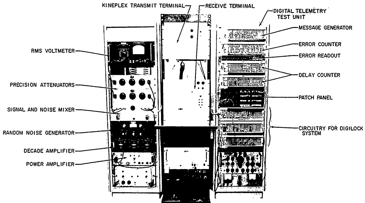
Figure 71. Instrumentation for testing Kineplex data transmission system
