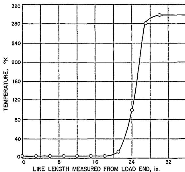
Figure 30. Temperature distribution along helium load transmission line
