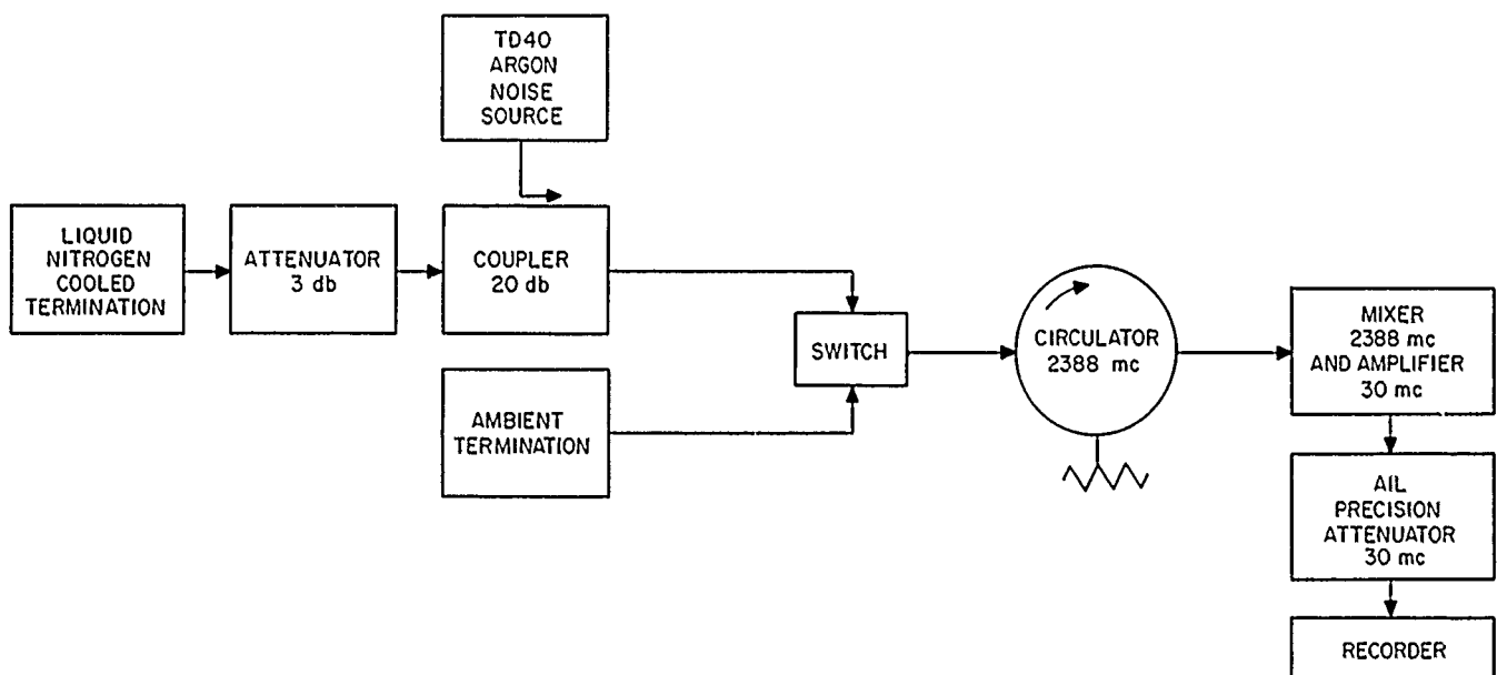
Figure 32. Noise source evaluation setup
