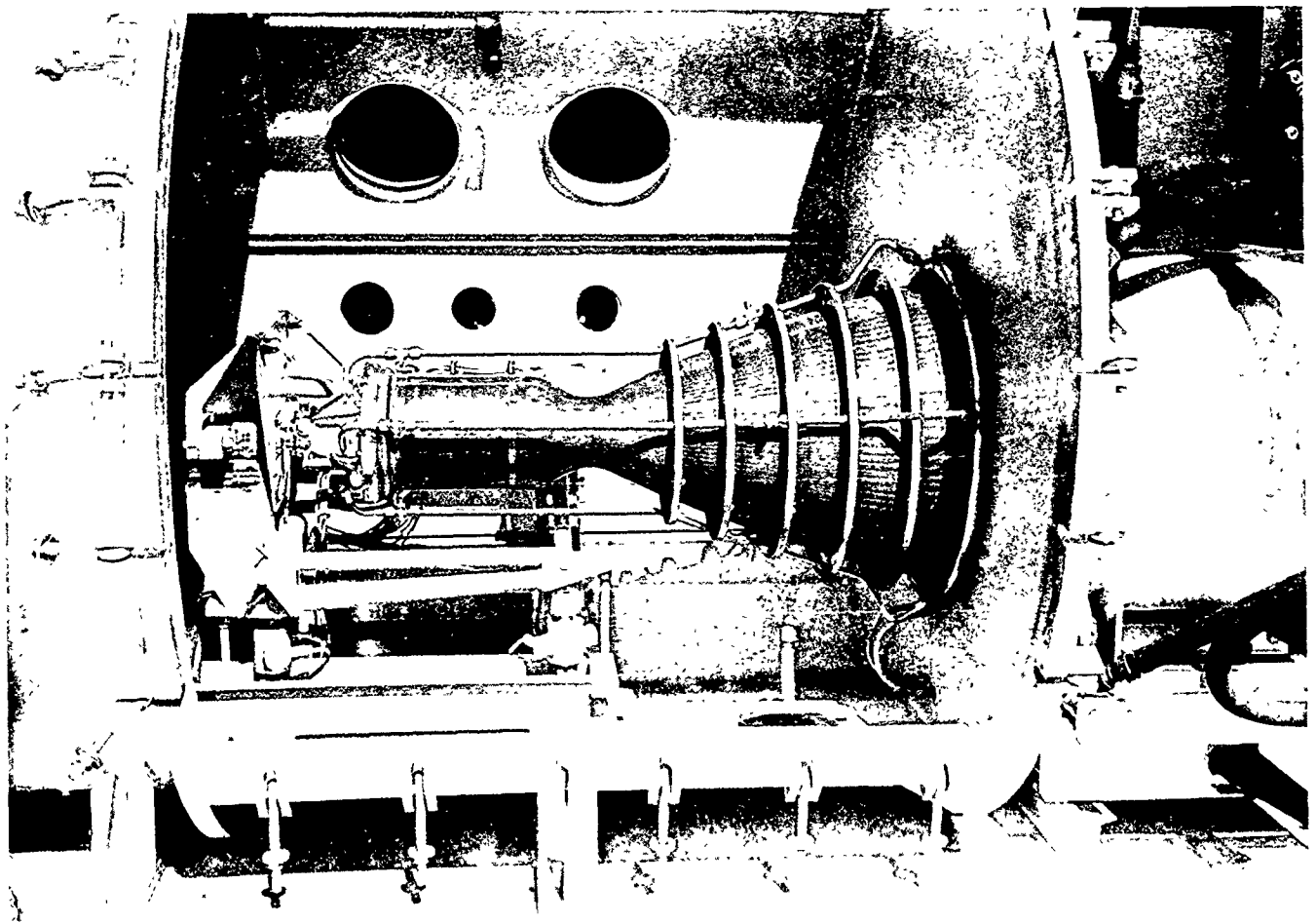
Figure 119. Thrust stand in vacuum chamber with mockup motor
