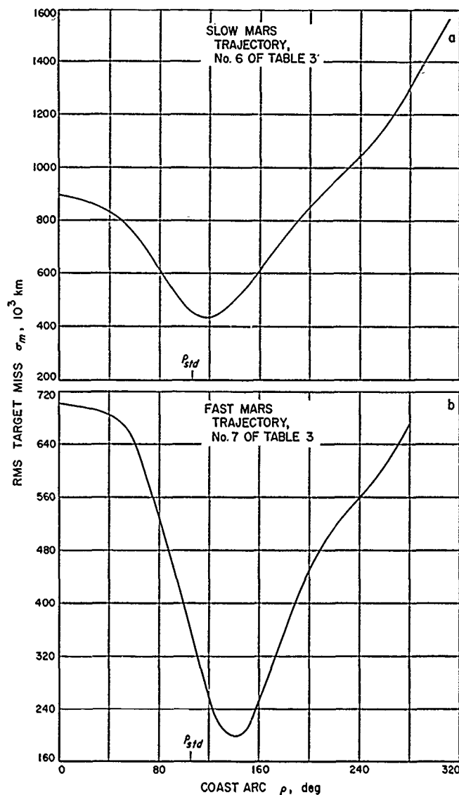
Figure 8. Mars miss distances vs coasting arc
