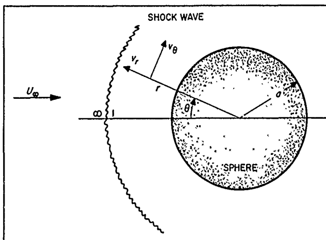
Figure 96. Coordinate system on sphere in hypersonic flow
