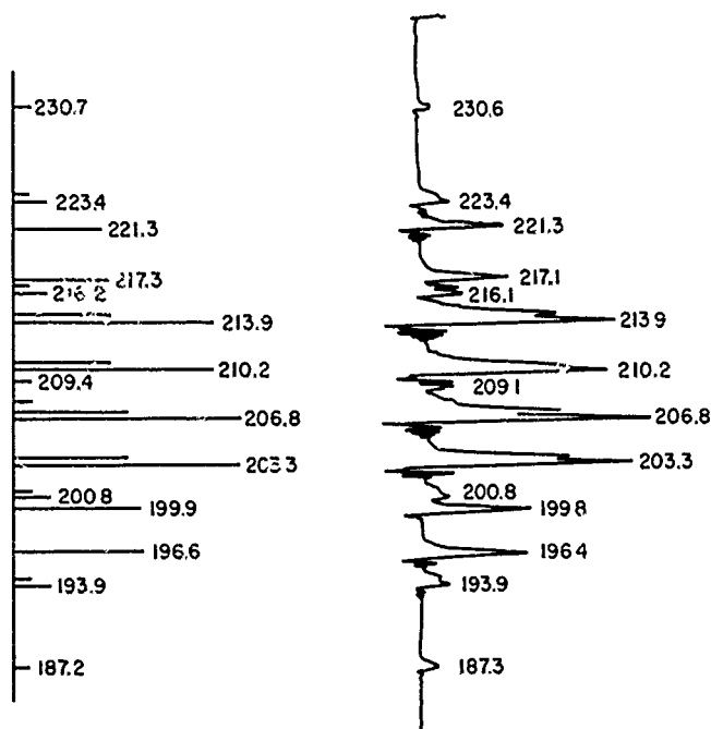
Figure 93. Nuclear magnetic resonance spectra of acetaldehyde diethylacetal at 60 mc with tetramethylsilane as internal reference
