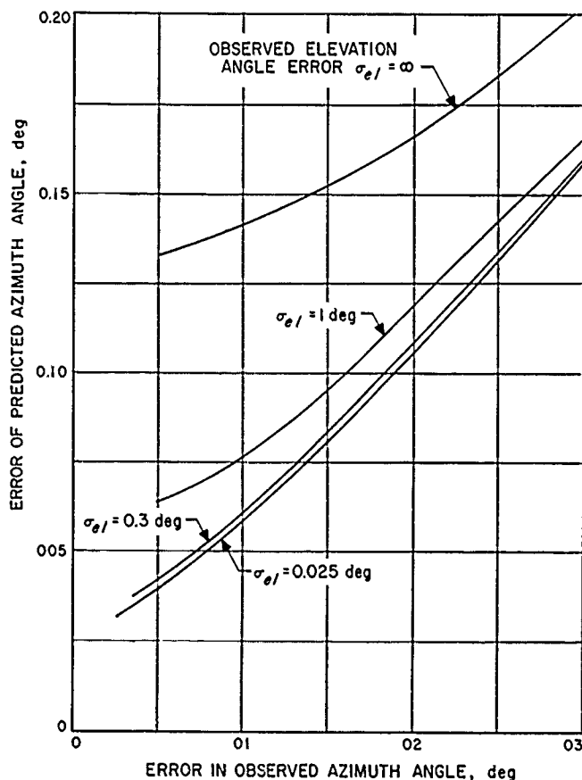
Figure 1. Error of predicted azimuth angle vs errors in observed azimuth and elevation angles
