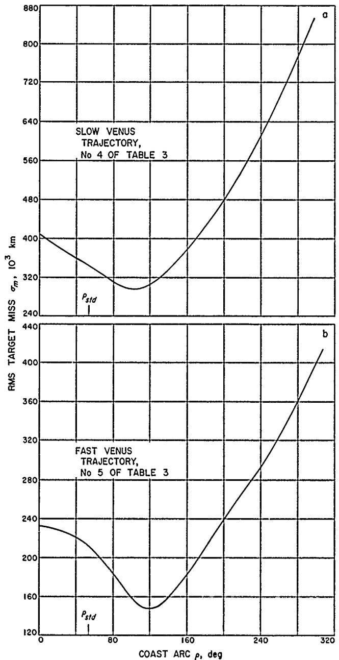
Figure 7. Venus miss distances vs coasting arc
