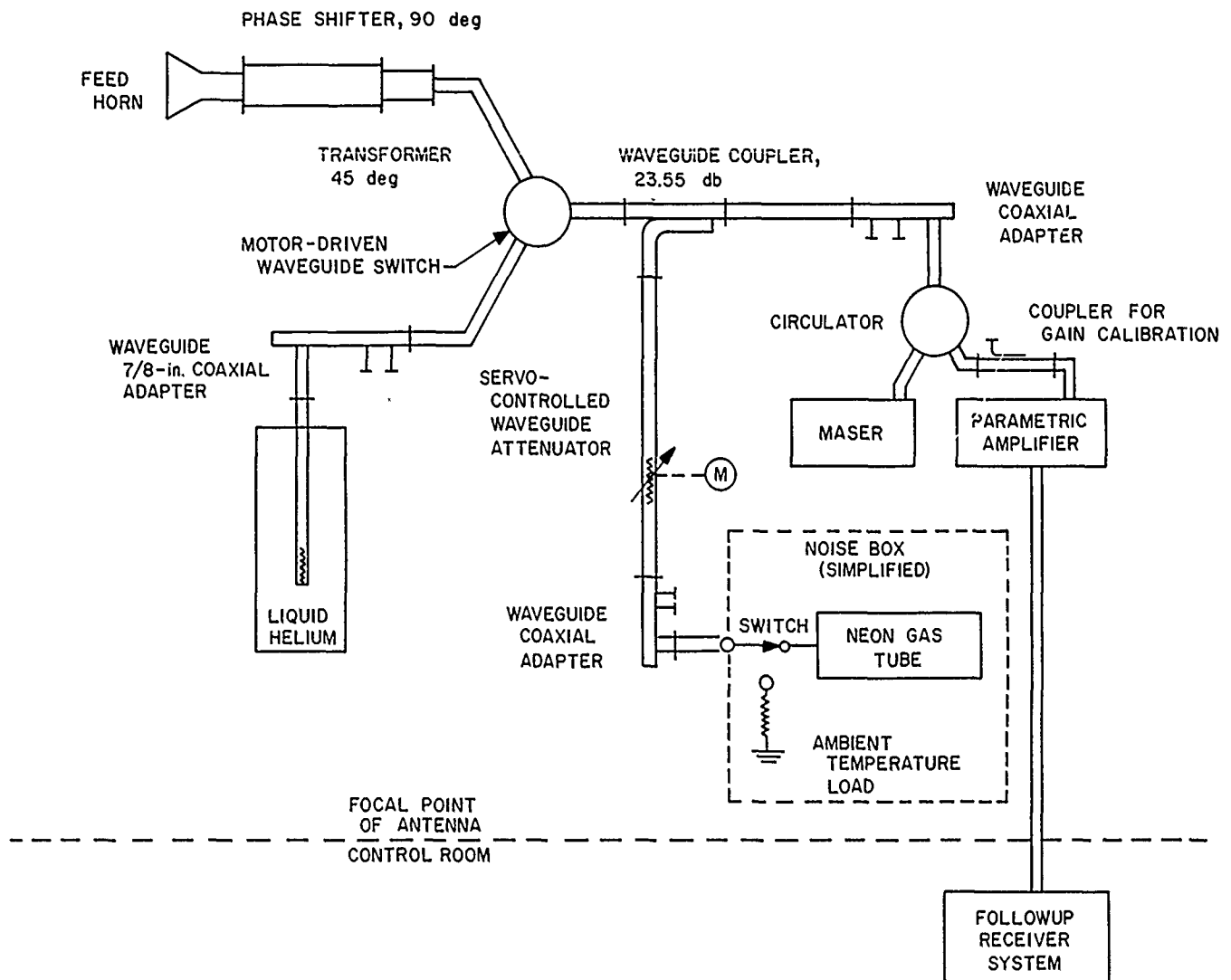
Figure 27. Feed system for Venus radar receiver
