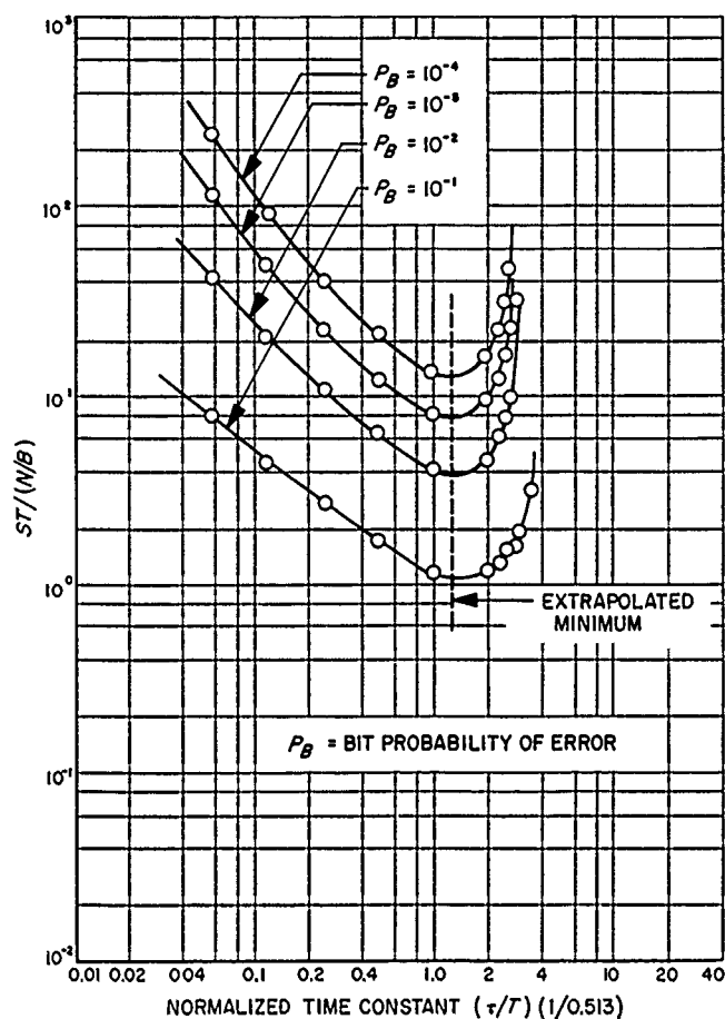
Figure 69. Extrapolated values for filter time constant
