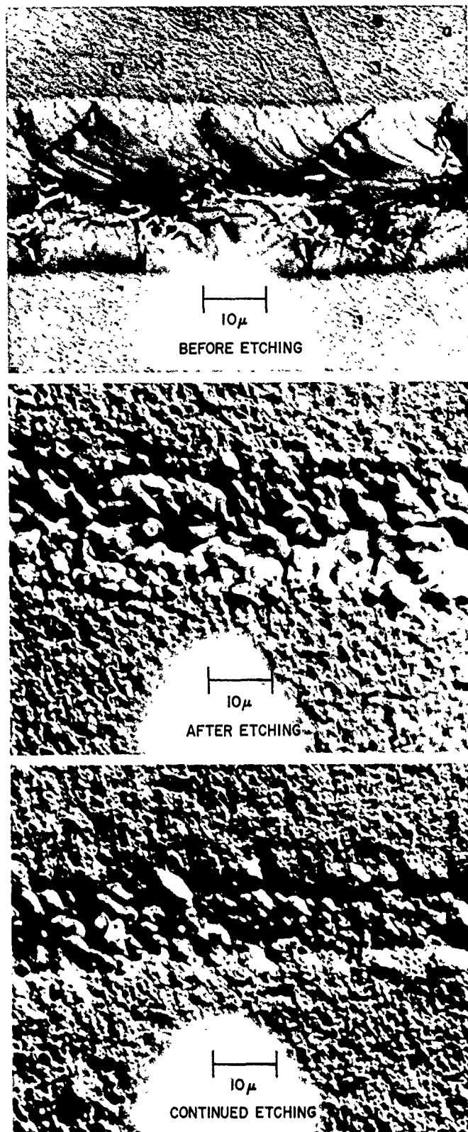
Figure 43. Photomicrograph of microzone melted path on germanium film before and after etching
