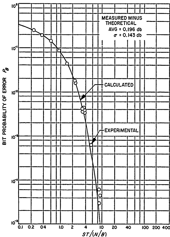
Figure 67. Probability of error for bit-by-bit PSK detection with matched filter
