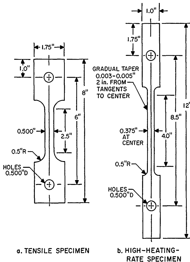
Figure 108. Tensile and high-heating-rate test specimens
