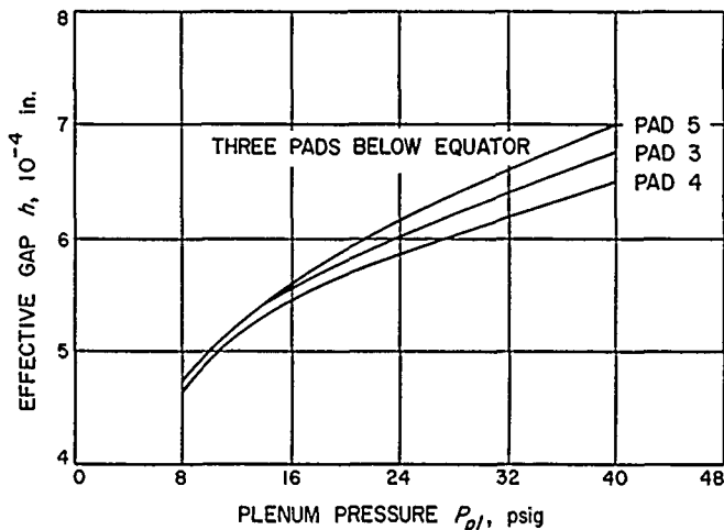
Figure 13. Six-pad spinning sphere, gap as a function of plenum pressure
