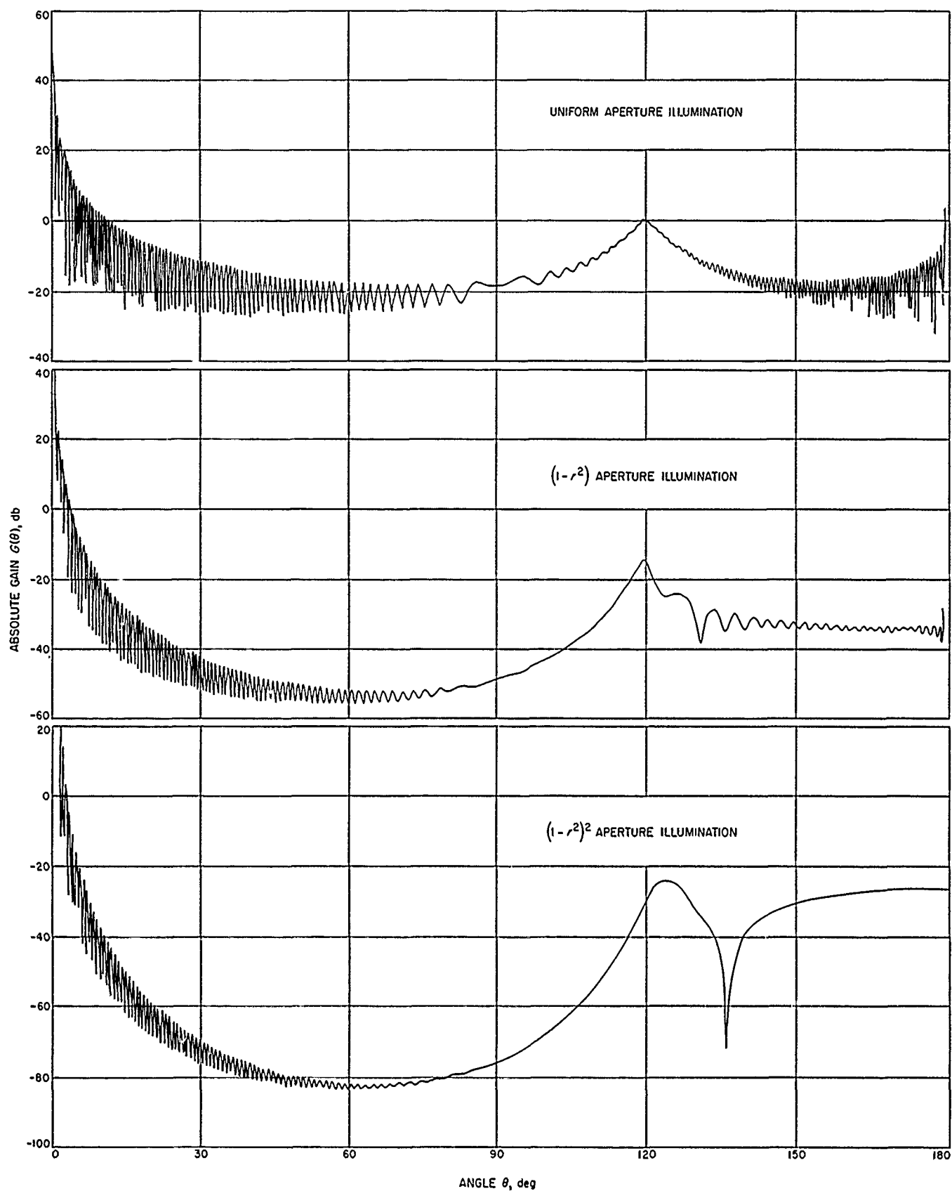
Figure 47. Absolute gain vs angle for D/\lambda = 83 and various aperture illuminations
