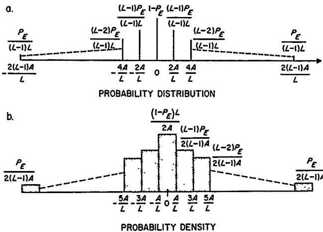
Figure 57. Probability distribution and density of errors for quantized PPM
