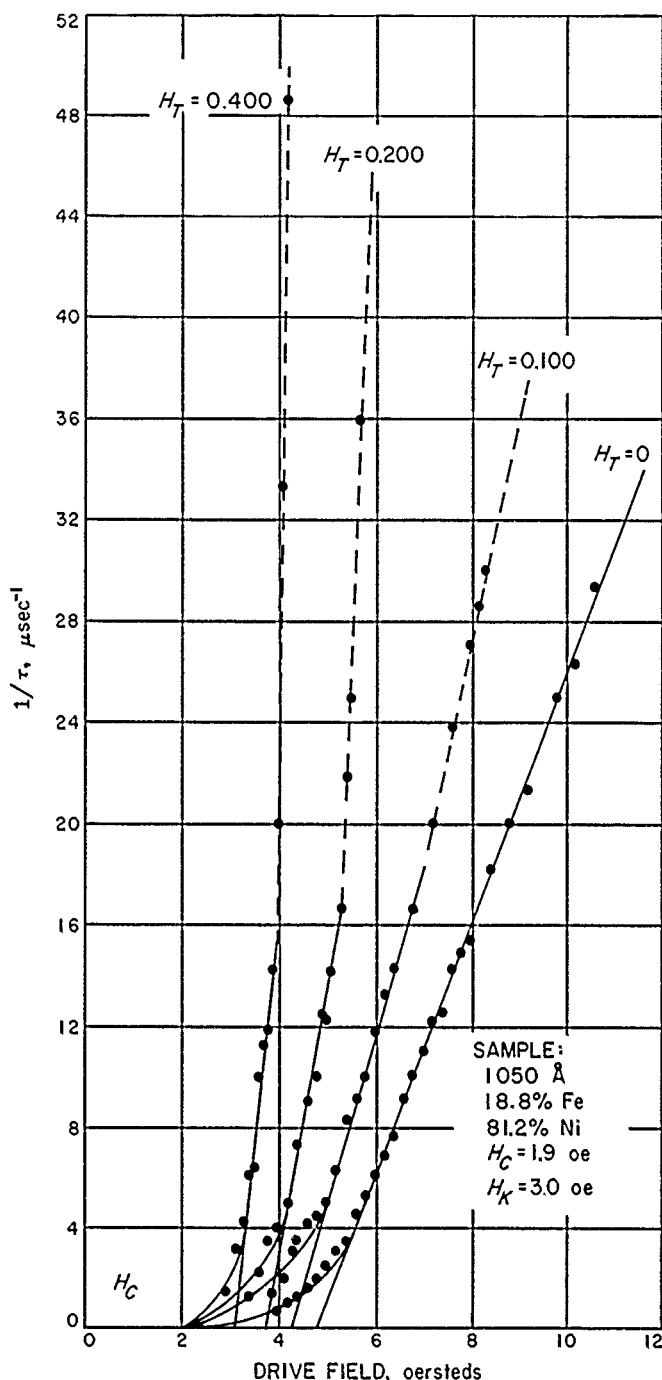
Figure 16. Typical reversal time vs drive field plot with transverse field as a parameter
