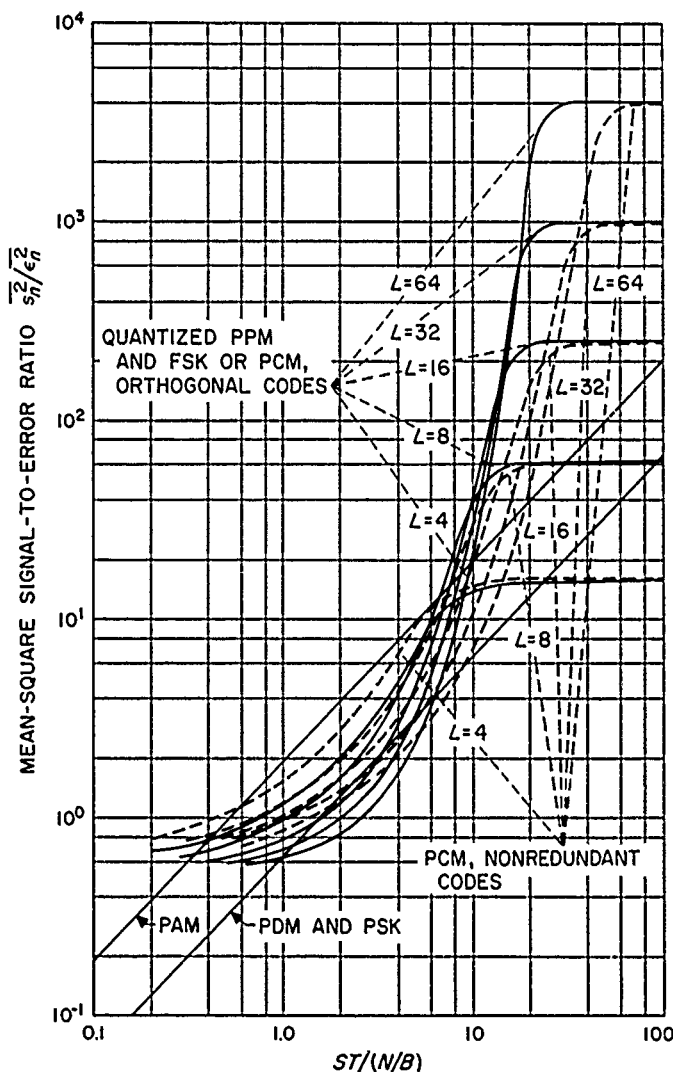
Figure 53. Mean-square signal-to-error ratio
