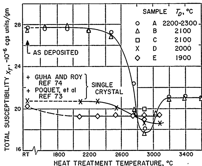
Figure 104. Total diamagnetic susceptibility of pyrolytic carbons deposited at temperatures T_D as a function of heat treatment temperature, values for natural single-crystal graphite shown for comparison
