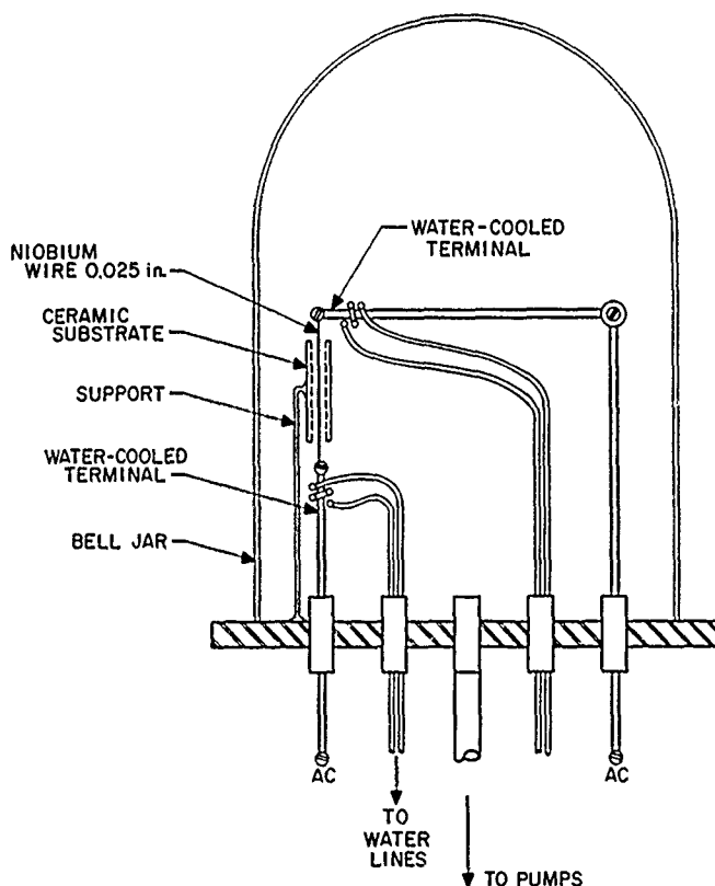
Figure 44. Vacuum chamber arrangement for niobium thin-film deposition
