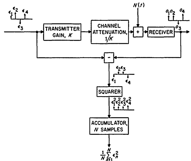
Figure 50. Measurement of mean-square error
