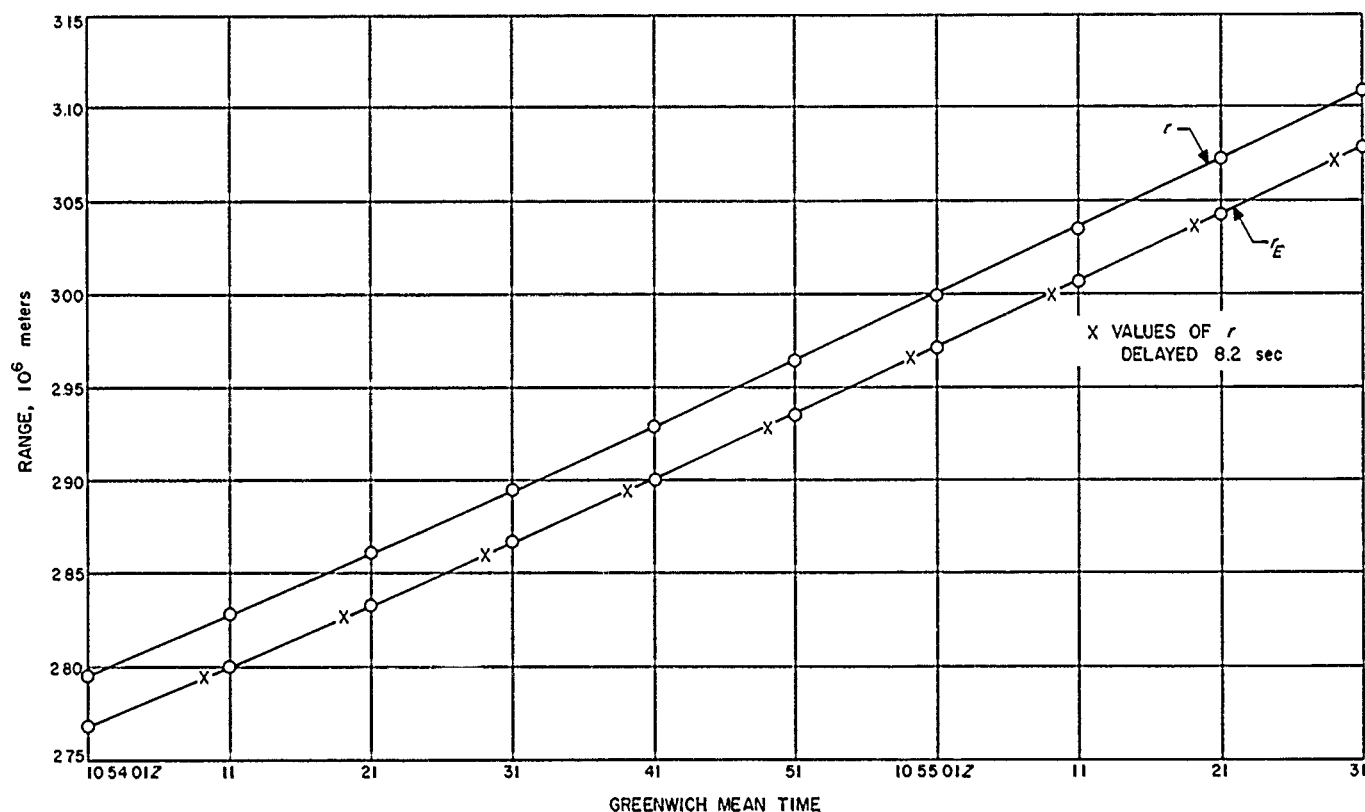
Figure 63. Echo pass 1107, first ranging portion
