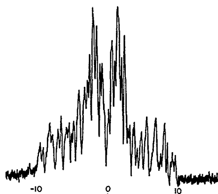
a. VINYL PROTONS OF CYCLOPENTADIENE (60 mc)
