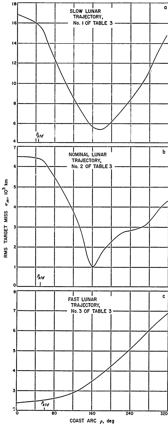
Figure 6. Moon miss distances vs coasting arc
