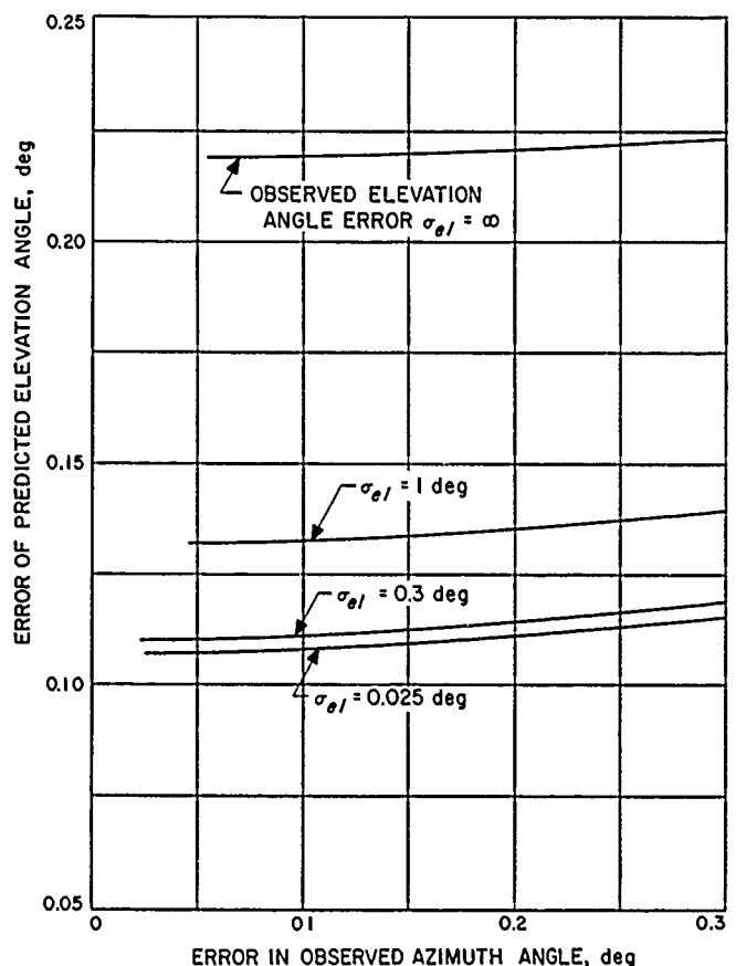
Figure 2. Error of predicted elevation angle vs errors in observed azimuth and elevation angles
