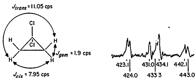
Figure 95. Up-field C^{13} satellite of 1,1-dichlorocyclopropane at 60 mc with chemical shifts relative to benzene J_{C^{13}-H} = 166.4 cps
