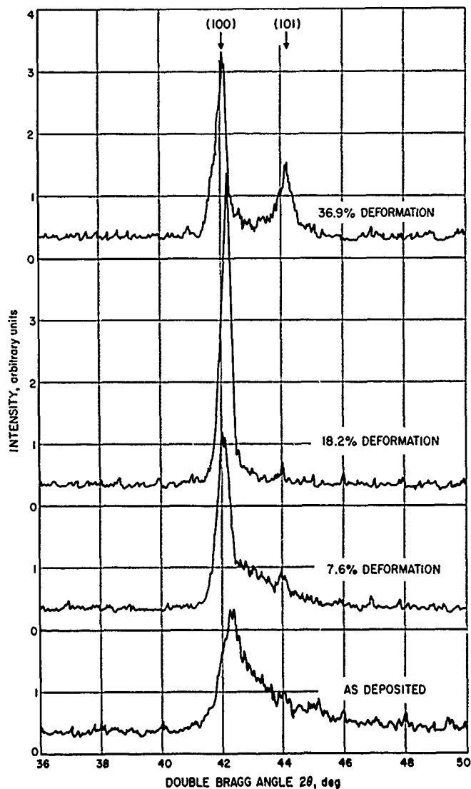
Figure 103. Development of modulations in (10) X-ray reflections of pyrolytic graphite after various deformations at 5000°F, CuK \alpha radiation, Block 14701
