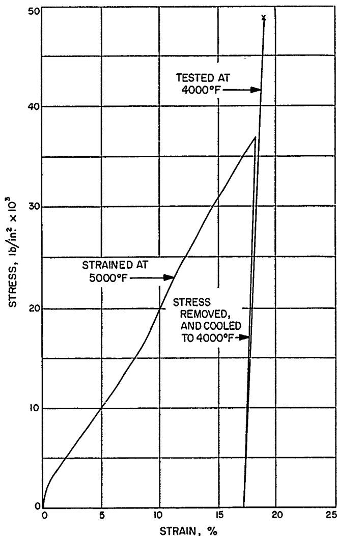
Figure 101. Engineering stress-strain curve for pyrolytic graphite prestrained at 5000°F, tested at 4000°F: stress parallel to basal planes, strain rate 2 \times 10^{-4} \text{ sec}^{-1} , Block 14701
