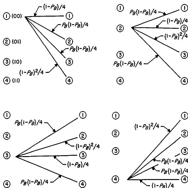
Figure 61. Transition diagram for nonredundant PCM, four levels
