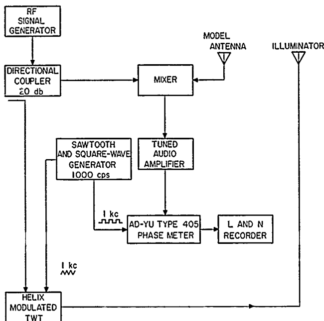
Figure 38. Phase measurement setup
