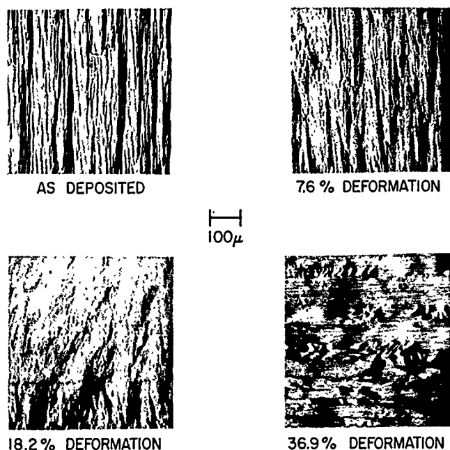
Figure 102. Microstructure of pyrolytic graphite after various deformations at 5000°F, Block 14701 unetched using polarized light
