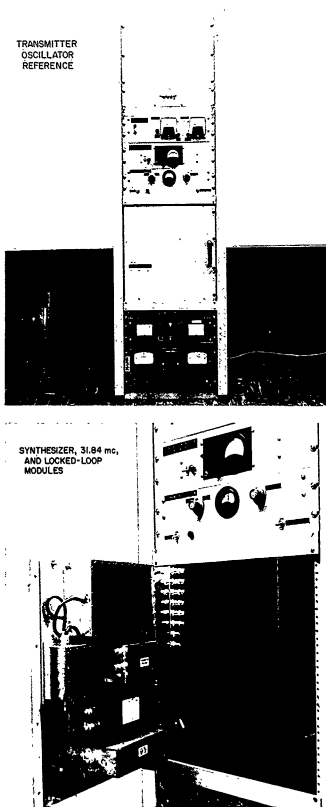
Figure 83. Transmitter oscillator reference for Venus radar experiment with 31.84-mc synthesizer and locked-loop modules
