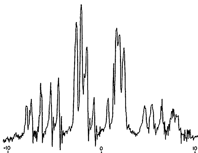
b. DECOUPLED VINYL PROTONS
