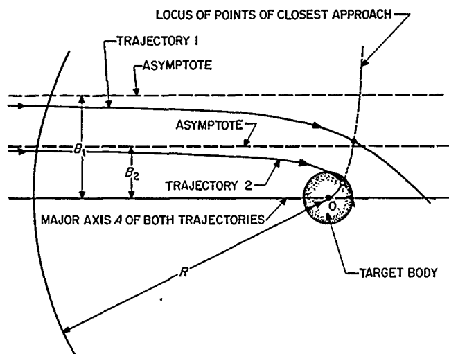
Figure 3. Near-target geometry showing varied trajectories
