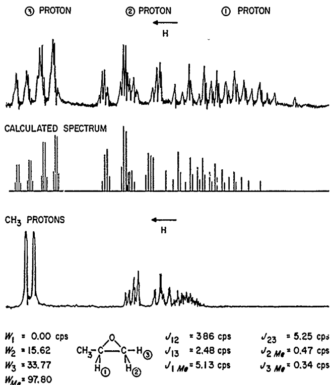
Figure 94. High-resolution NMR spectrum of propylene oxide
