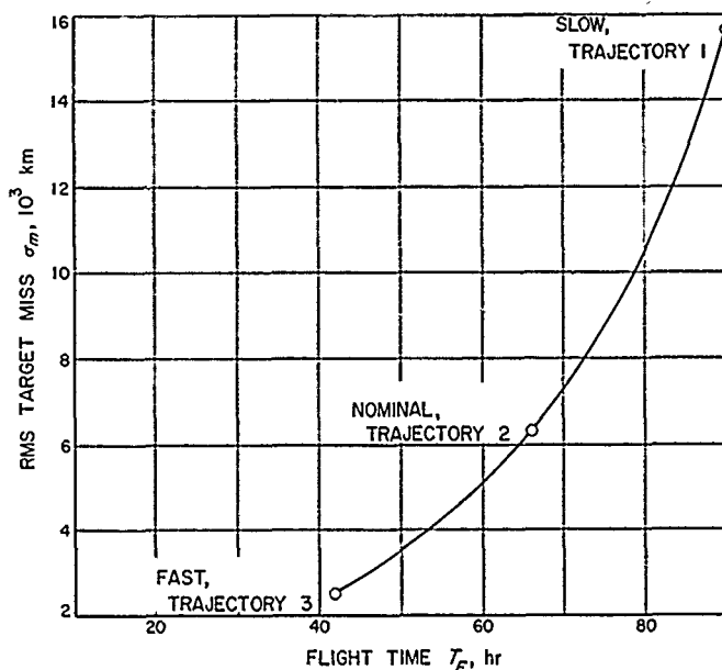
Figure 9. Moon miss distances vs flight time
