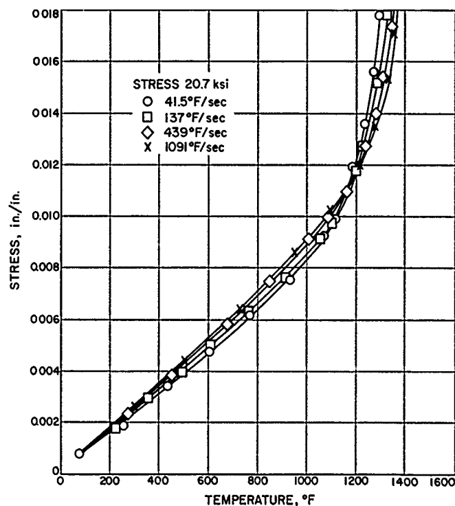
Figure 112. Typical strain-temperature curves at various heating rates for 17-7 PH (1050) stainless steel
