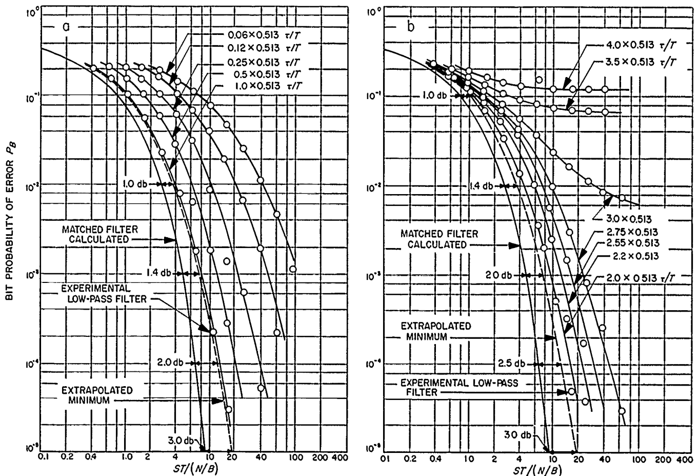
Figure 68. Probability of error for bit-by-bit PSK detection with low-pass filter
