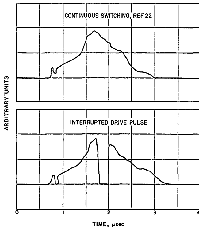
Figure 17. Typical voltage transient observed with longitudinal loop while switching films in Region I
