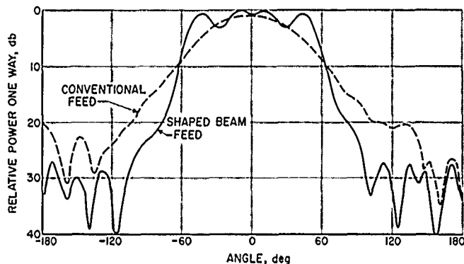
Figure 24. Conventional and shaped beam E-plane patterns
