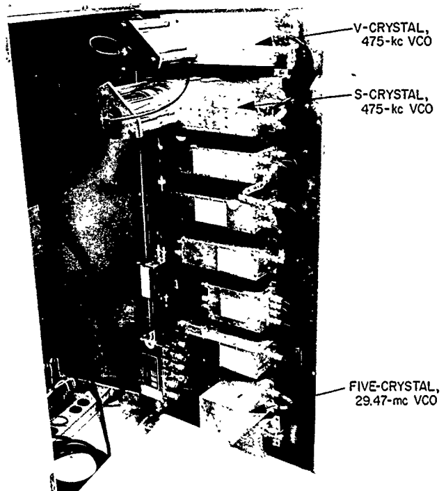
Figure 85. RF modules for synthesized receiver local oscillator
