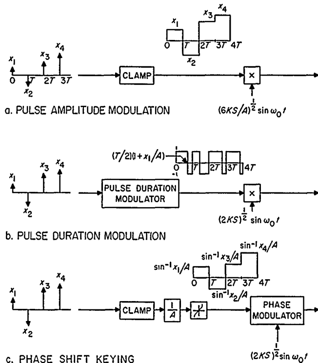
Figure 51. Modulation systems pertinent to linear synchronous detection
