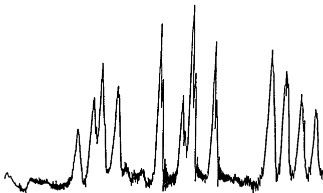
b. DECOUPLED SPECTRUM OF PROPYLENE OXIDE
