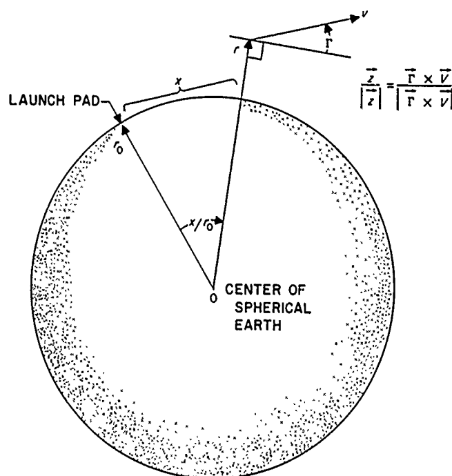
Figure 5. Coordinate system used in parking orbit error study
