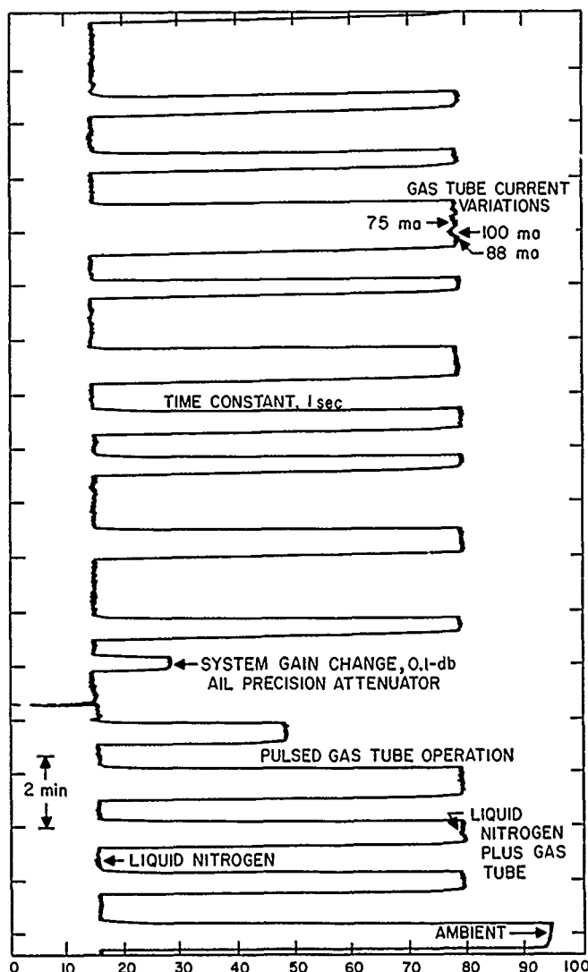
Figure 33. Recording of excess noise of argon TD40 noise source at 2388 mc
