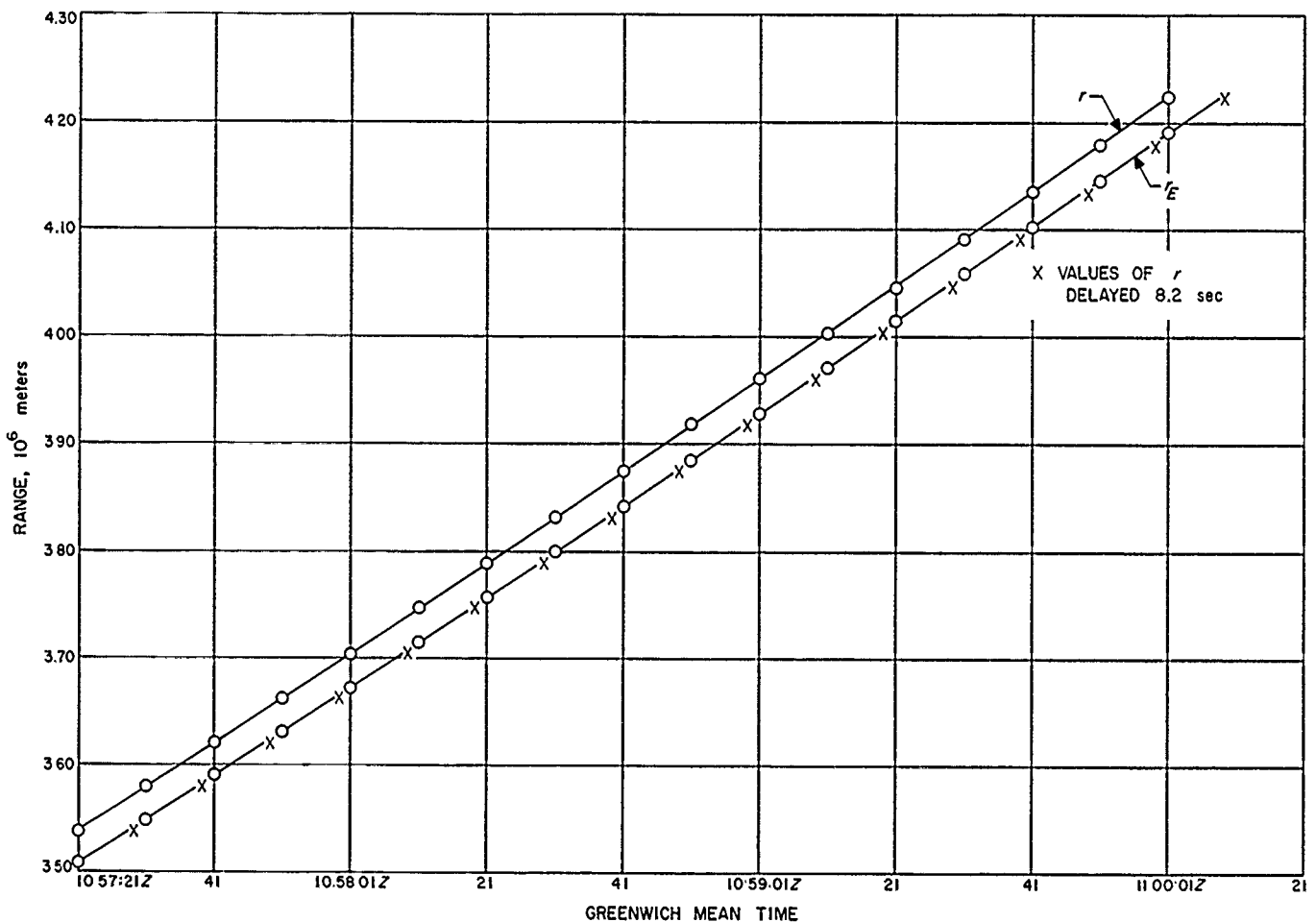
Figure 64. Echo pass 1107, second ranging portion
