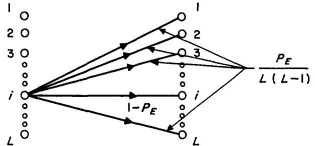
Figure 56. Transition diagram for quantized PPM
