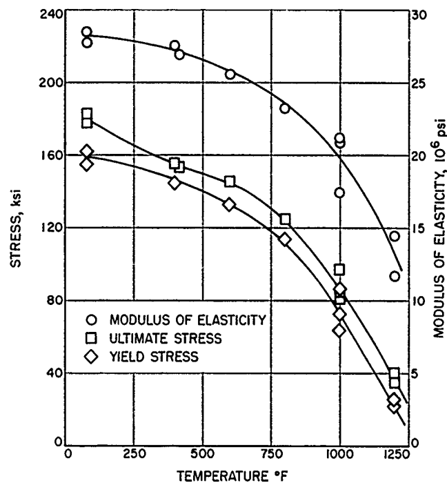
Figure 110. Ultimate stress, yield stress, and modulus data for 17-7 PH (1050) stainless steel at temperatures from 70 to 1200°F
