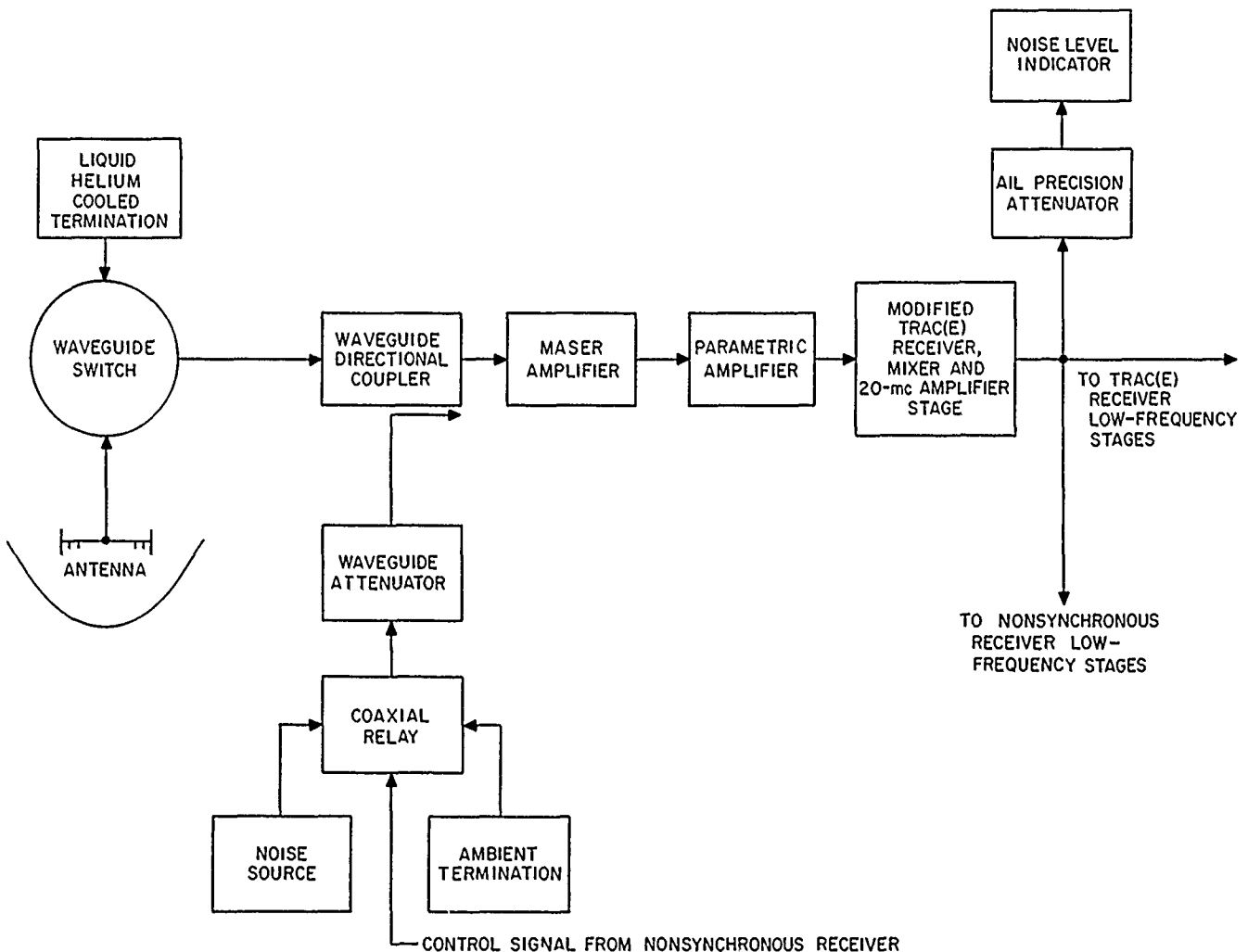
Figure 37. Venus radar system temperature measurement equipment
