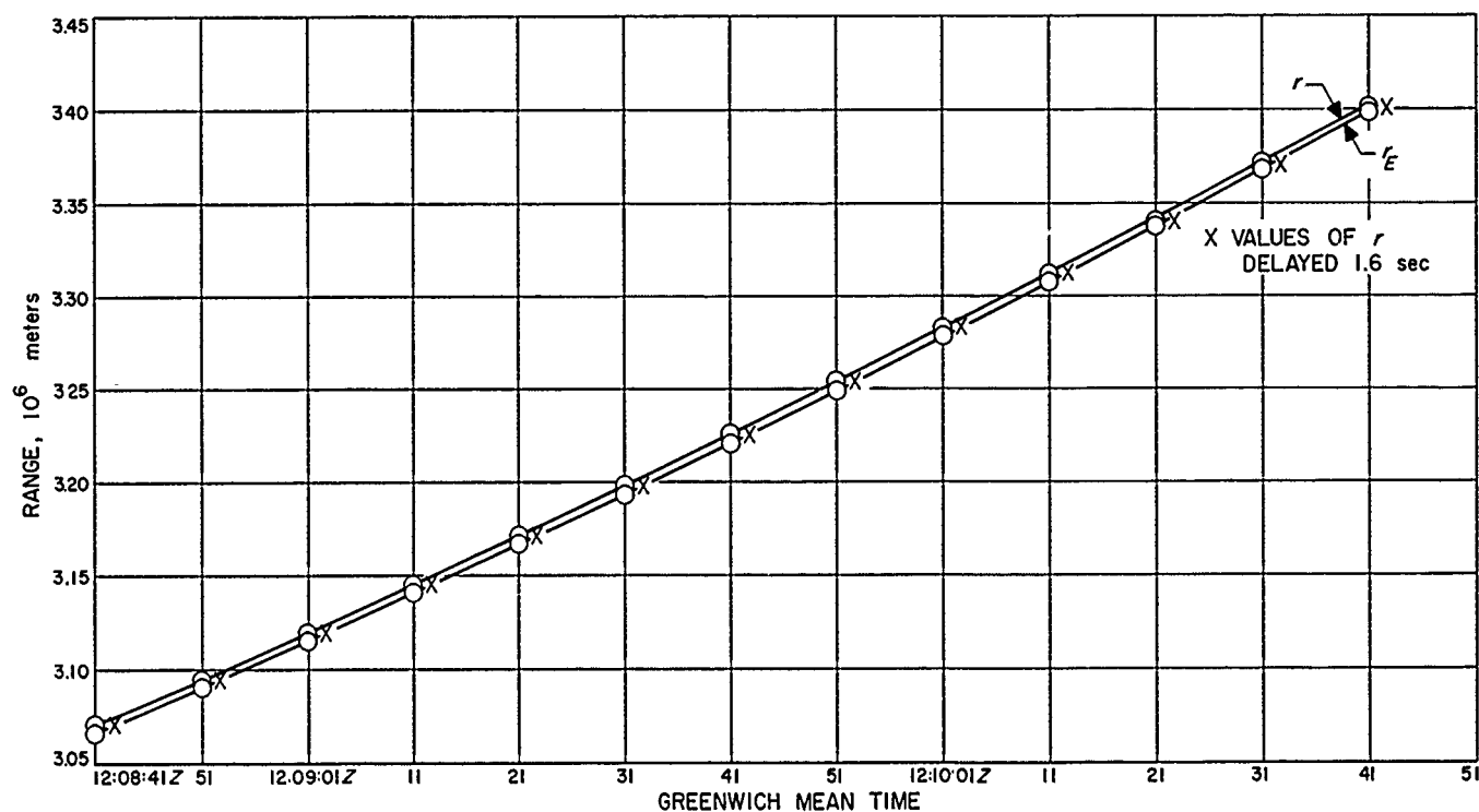
Figure 65. Echo pass 1185, ranging portion
