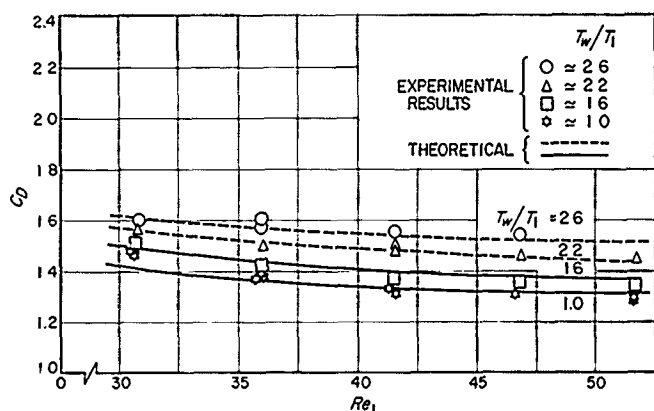
Figure 97. Theoretical and experimental sphere drag, 3.8 < M_\infty < 4.3 ; 0.013 < K_n < 0.200 ; 1 < T_{10}/T_1 < 2.6
