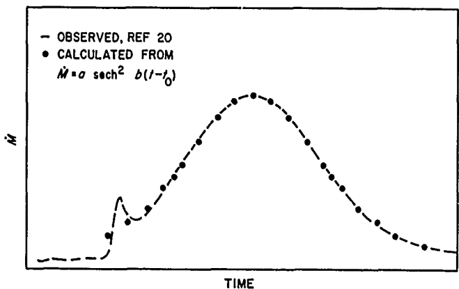
Figure 18. Observed voltage transient during reversal compared with that calculated from nonuniform rotation model
