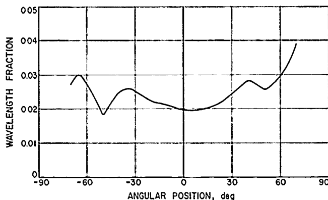
Figure 40. Antenna H-plane phase pattern
