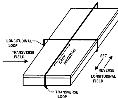
Figure 15. Relative direction of external fields on thin film and position of loops used to observe flux changes
