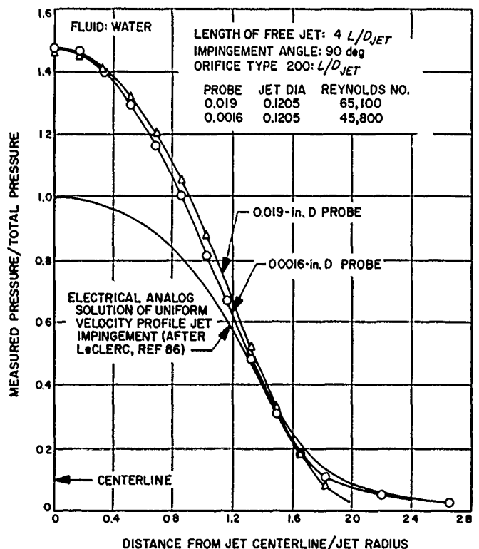
Figure 121. Pressure distribution produced by a free liquid jet with fully developed turbulent profile, impinging on a flat plate
