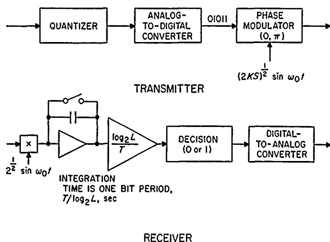
Figure 59. Nonredundant PCM system
