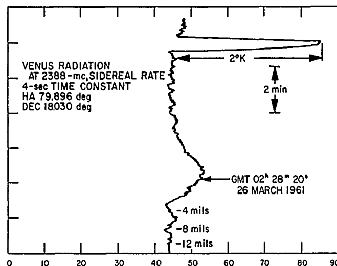
Figure 35. Drift curve of 2388-mc radiation for Venus
