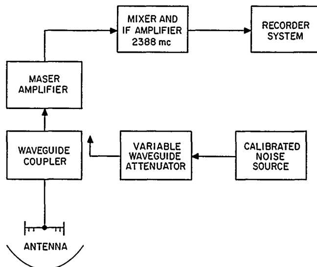
Figure 34. Radiometer setup using 2388-mc maser amplifier
