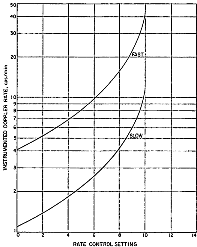
Figure 81. Pulsed oscillator rate control characteristics
