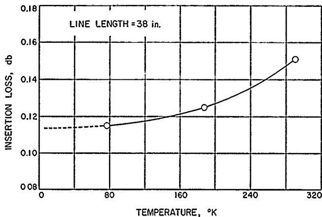
Figure 31. Insertion loss of 0.75-inch transmission line vs temperature
