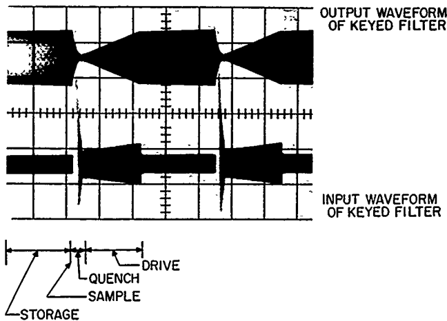
Figure 74. Keyed filter input and output waveforms
