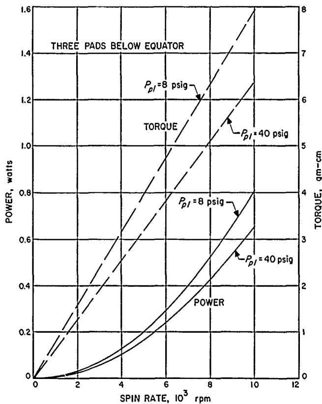
Figure 14. Six-pad spinning sphere, torque and power as a function of speed
