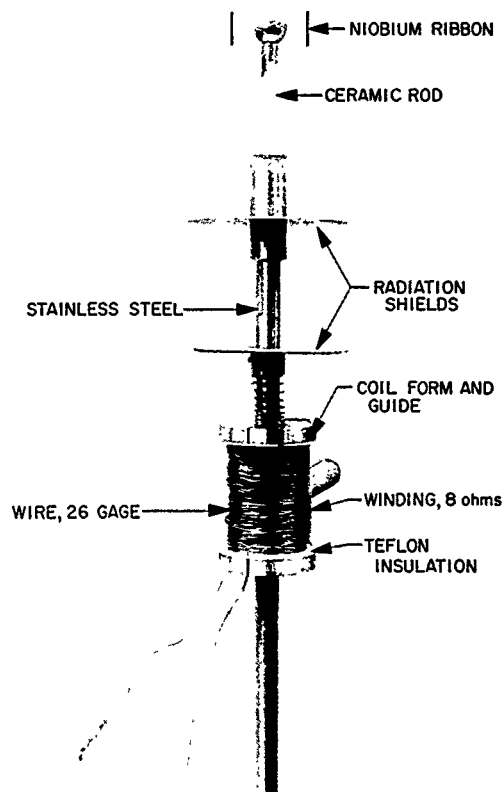
Figure 45. Support for uniform film deposition on spheres
