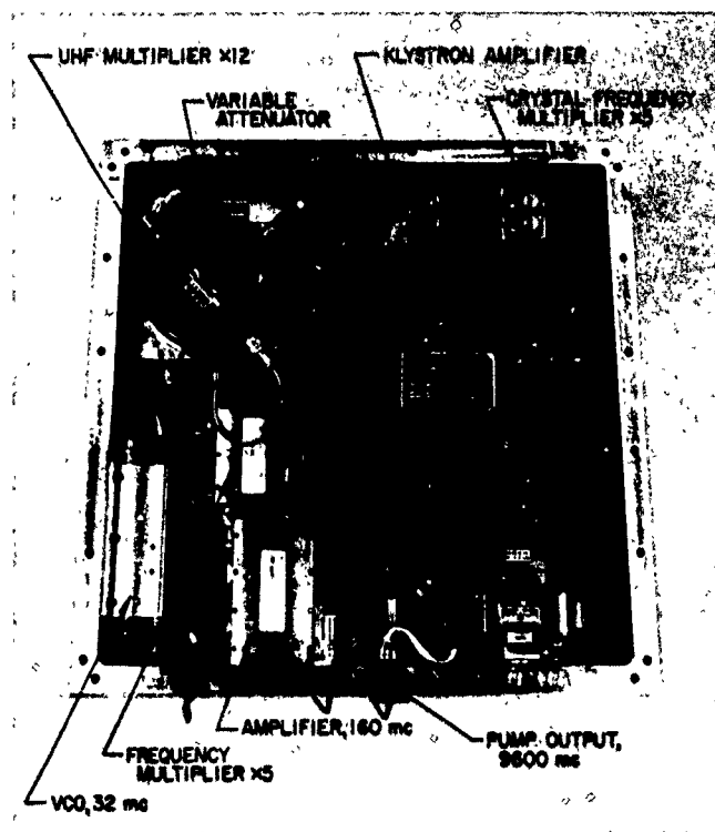
Figure 88. Pump source components
