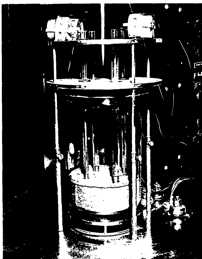
Figure 107. Dynamic penetration apparatus for simulated lunar material
