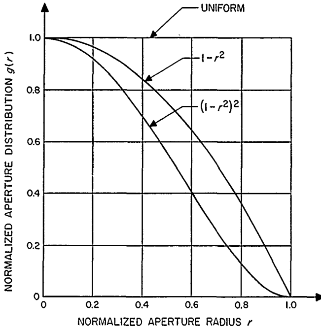
Figure 49. Aperture distributions
