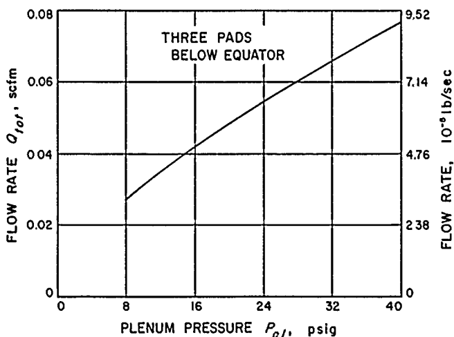
Figure 12. Flow rate of the six-pad spinning sphere
