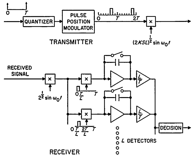
Figure 54. Quantized pulse position modulation system employing correlation detection
