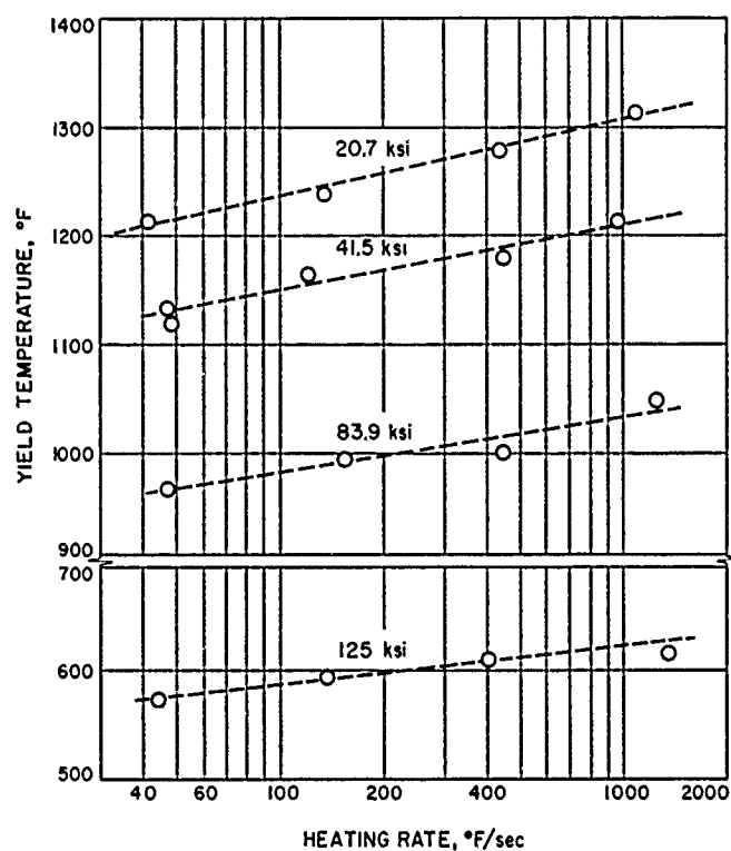
Figure 113. Effect of heating rate on yield temperatures for various stress levels
