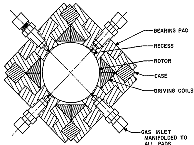
Figure 10. Section drawing of six-pad spinning sphere
