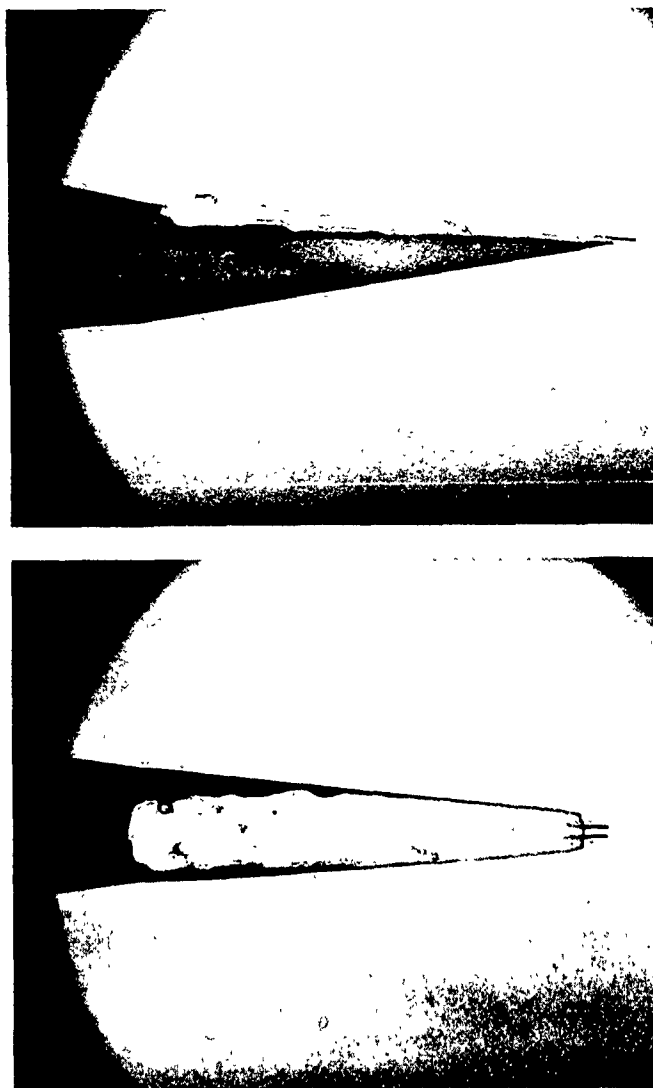
Figure 98. Hypersonic hot-wire probes
