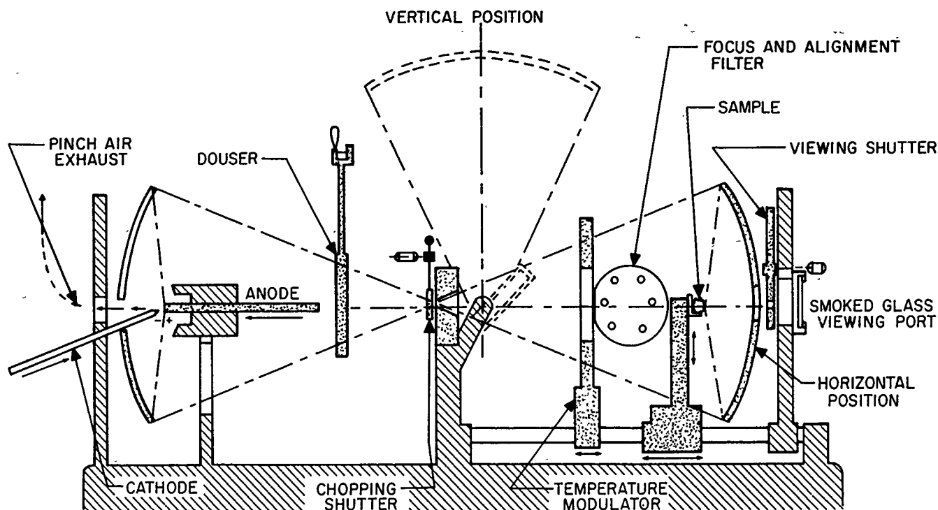
Figure 105. Arc imaging furnace for materials research
