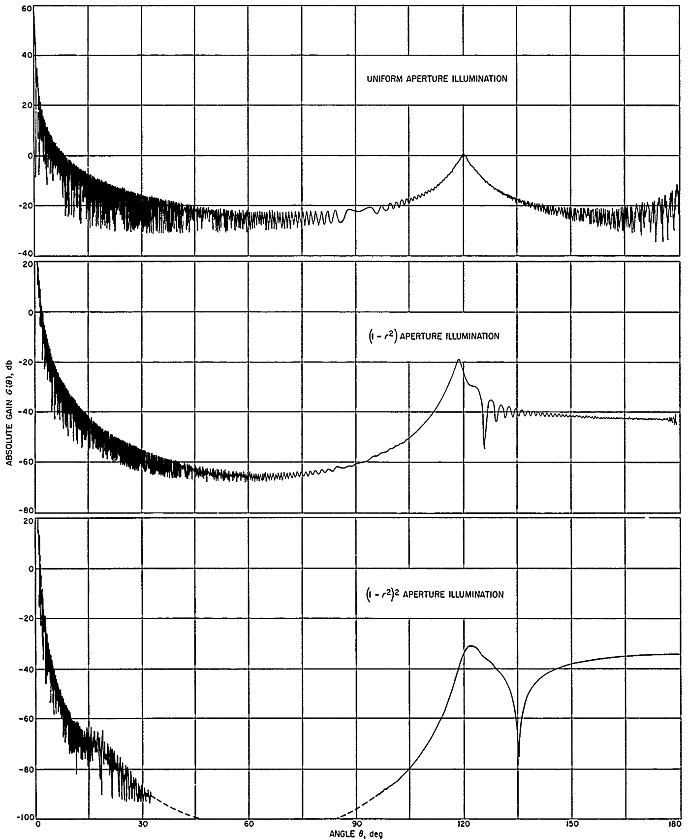
Figure 48. Absolute gain vs angle for D/\lambda = 200 and various aperture illuminations
