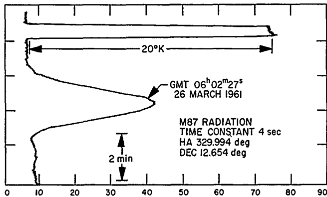
Figure 36. Drift curve of 2388-mc radiation for M87
