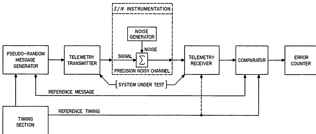
Figure 66. Bit-by-bit telemetry test system
