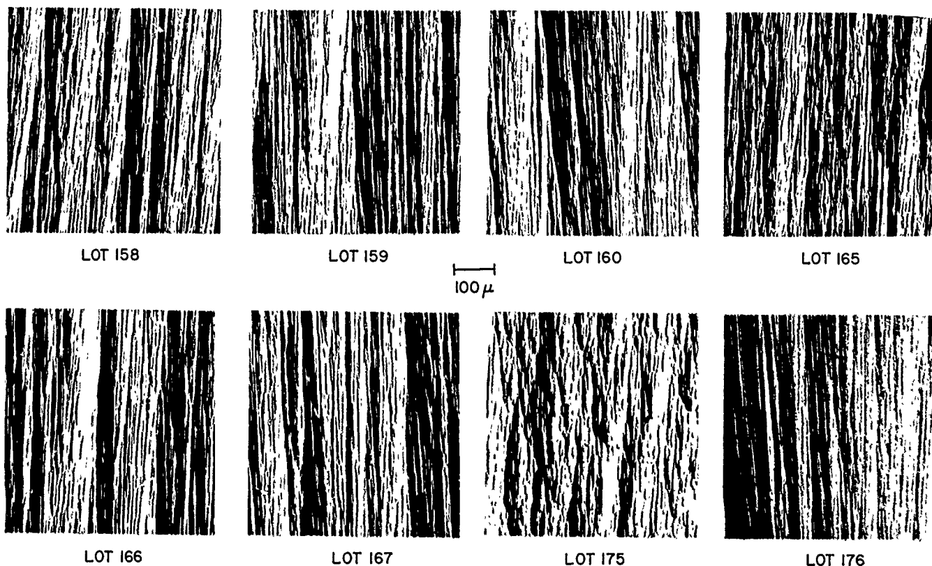
Figure 100. Microstructure of as-deposited pyrolytic graphite, unetched using polarized light
