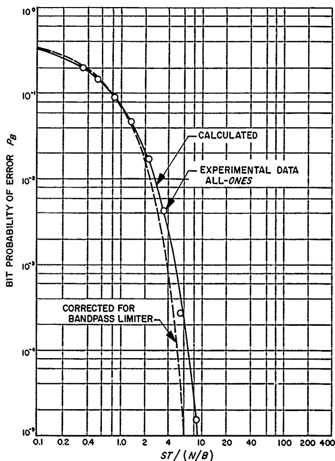
Figure 70. Probability of error for bit-by-bit detection using all-ones data
