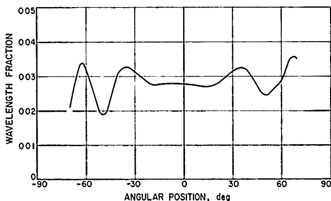
Figure 39. Antenna E-plane phase pattern
