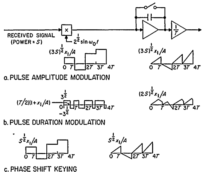
Figure 52. Waveforms at input and output of pulsed integrator for linear synchronous detection
