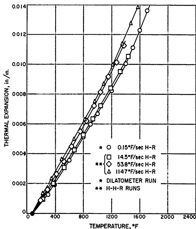
Figure 111. Effect of heating rate on thermal expansion of 17-7 PH (1050) stainless steel
