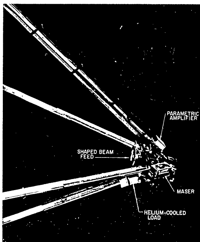
Figure 28. Maser and low-noise feed installation
