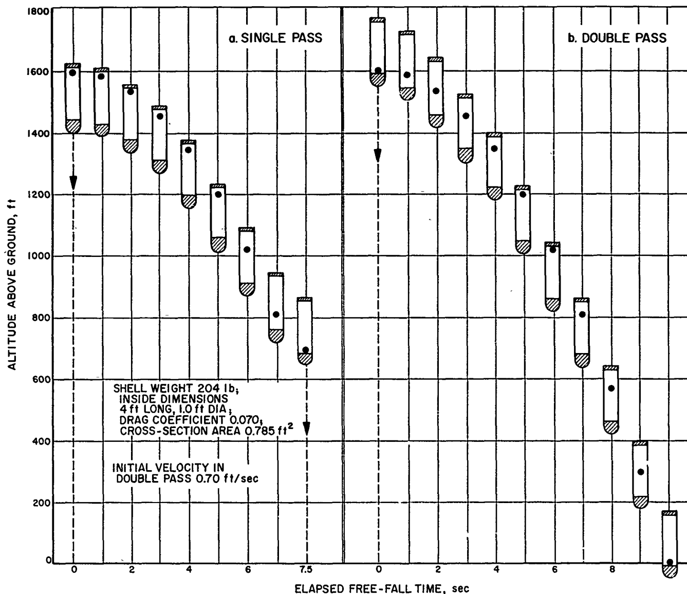
Figure 115. Relative vertical displacement between experiment and capsule shell for single- and double-pass techniques
