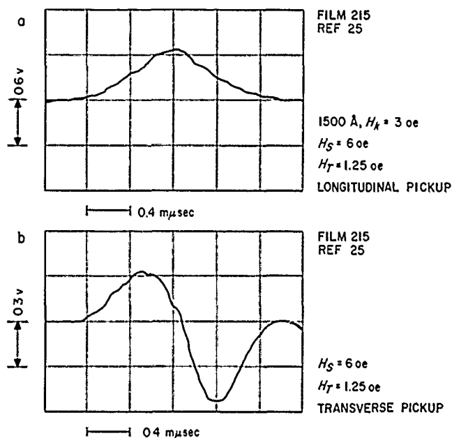
Figure 19. Comparison of observed longitudinal and transverse flux changes during reversal of thin film in Region III
