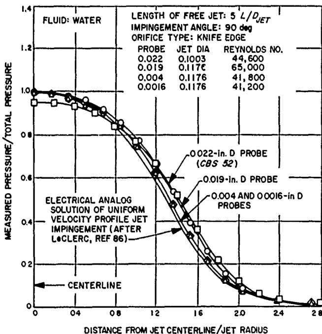
Figure 120. Pressure distribution produced by a free liquid jet with uniform velocity profile, impinging on a flat plate
