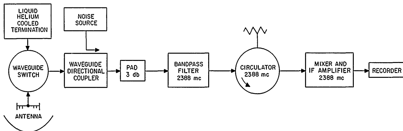
Figure 29. Block diagram of 2388-mc antenna temperature measurement setup
