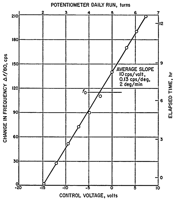
Figure 80. The 475-kc VCO characteristics, f_0 = 474.975 kc
