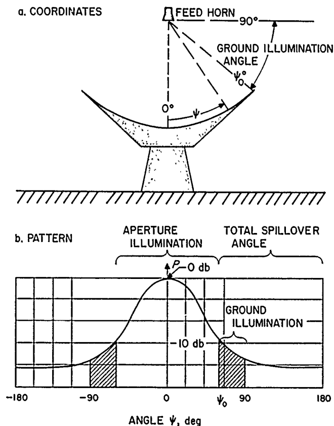
Figure 23. Typical primary feed pattern
