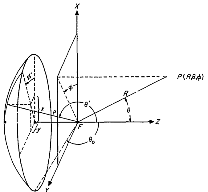
Figure 46. Antenna geometry
