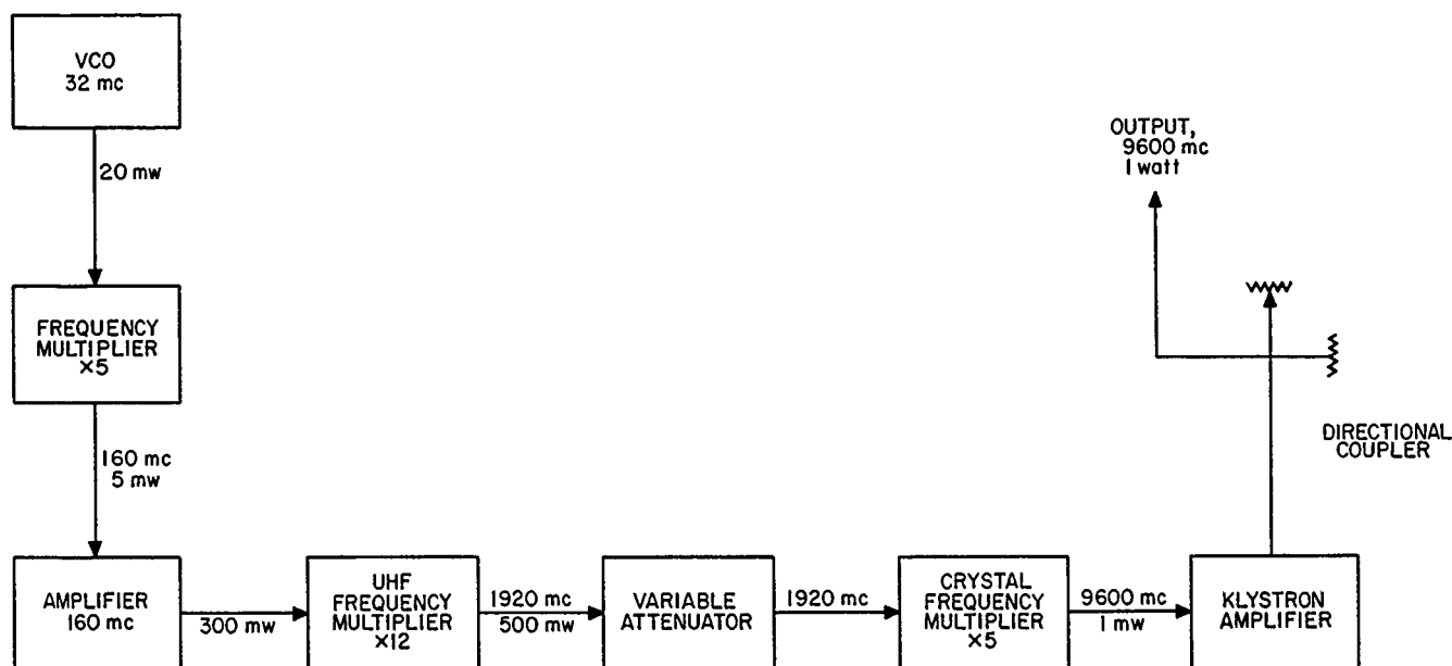
Figure 87. Block diagram of 9600-mc pump source
