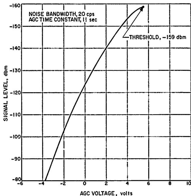
Figure 89. The 2388-mc receiver gain characteristic
