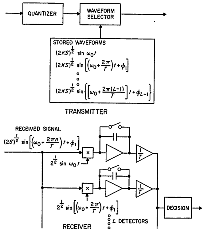
Figure 58. Quantized FSK system employing correlation detection
