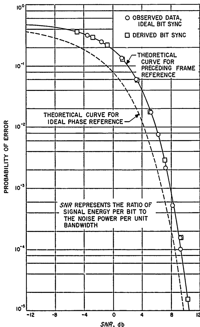
Figure 76. Probability of error vs SNR for Kineplex system with preceding frame reference
