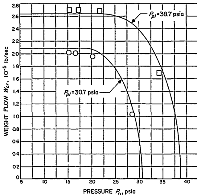
Figure 20. Weight flow through orifice vs absolute pressure at bearing entrance
