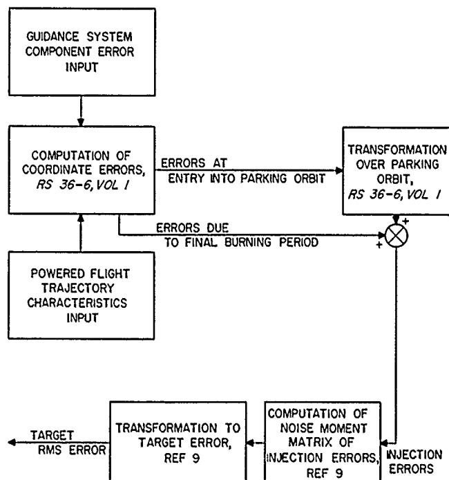
Figure 4. Computation of target miss distances resulting from component errors
