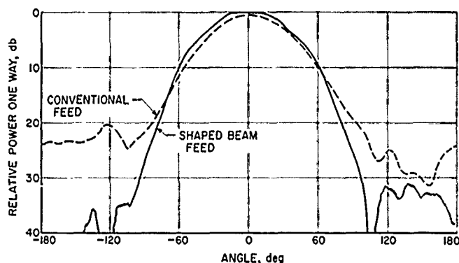
Figure 25. Conventional and shaped beam H-plane patterns
