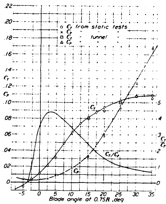
FIGURE 23 Characteristics of 2-blade propeller 6624. Rot at zero V , n/D = 0.5
