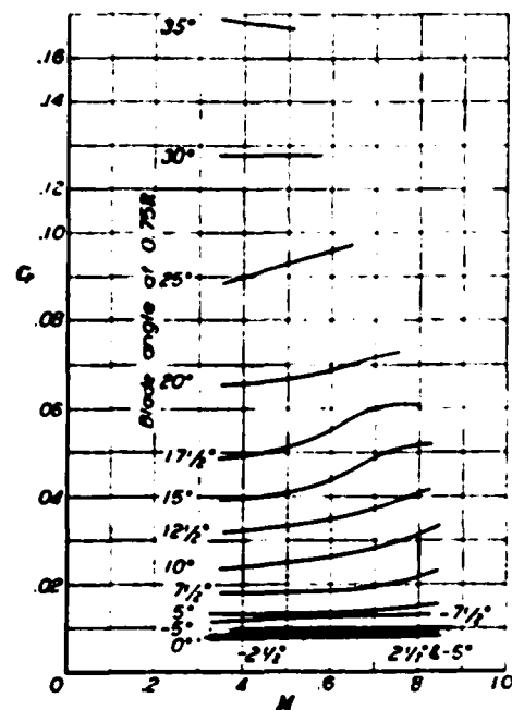
FIGURE 9—Variation of static-power coefficient with tip-speed ratio and blade angle Propeller No. 1A, 2 blades
