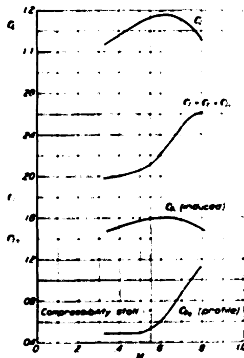
FIGURE 17. Effect of compressibility on airfoil coefficients obtained from the static test propeller coefficients for 2-blade propeller 3623 R6 at 15^\circ at 0.75 ft/sec.
