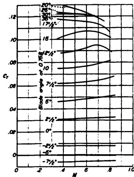
FIGURE 8—Variation of static-thrust coefficient with tip-speed ratio and blade angle Propeller No. 1A, 2 blades
