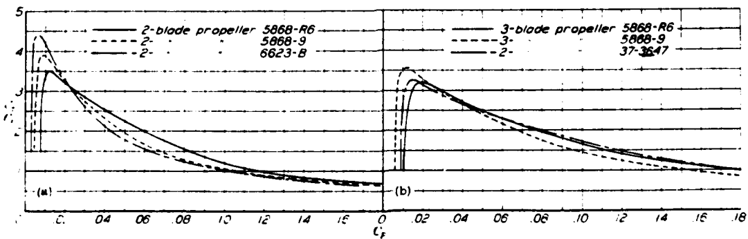
FIGURE 29.- Comparison of propeller characteristics. C_T/C_P against C_F ; V \propto D, 0; M, 0.5 .
