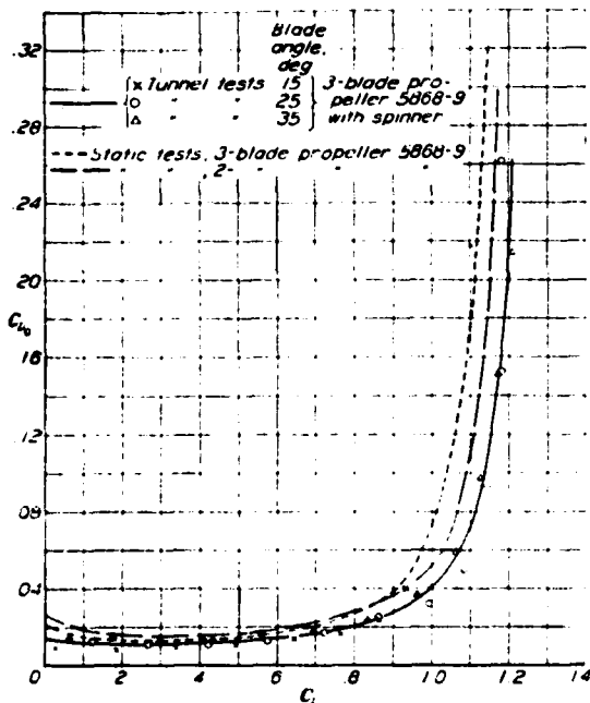
FIGURE 33 Comparison of polars obtained from wind-tunnel and static tests of propeller 5868-9
