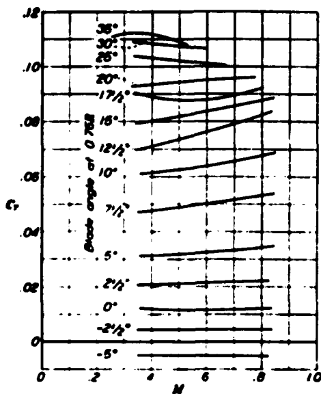
FIGURE 11. Variation of static thrust coefficient with tip-speed ratio and blade angle. Propeller No. 1, R, 2 Blade.
