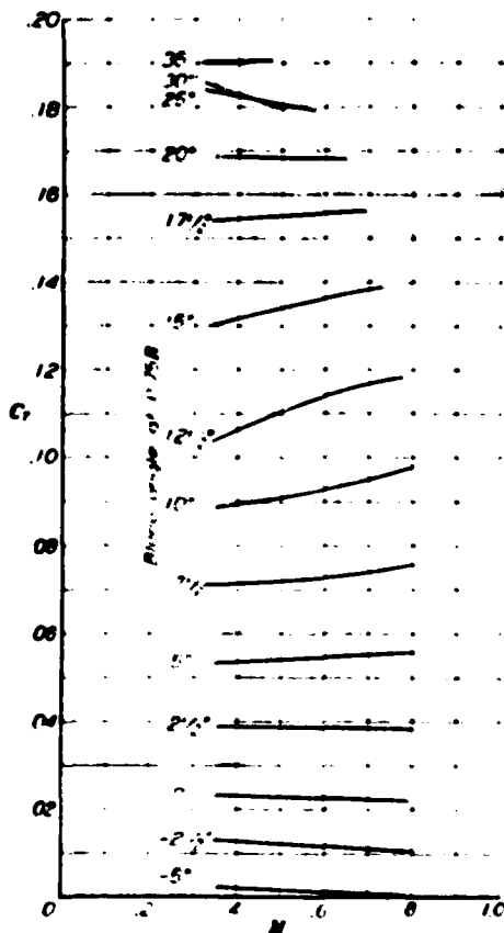
FIGURE 13. Variation of static thrust coefficient with tip-speed ratio and blade angle. Propeller No. 2, R, 2 Blade.
