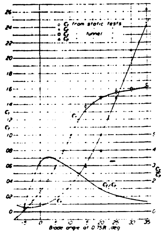
FIGURE 22. Characteristics of 2-blade propeller. Same as in Fig. 19, M = 0.5 .
