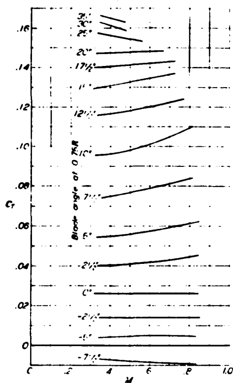
FIGURE 7. Variation of static thrust coefficient with tip-speed ratio and blade angle. Propeller No. 9, 3 blades.
