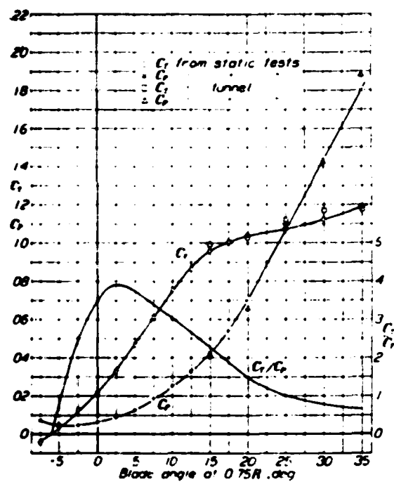
FIGURE 21. Characteristics of 2-blade propeller. Same as in Fig. 19, M = 0.5 .
