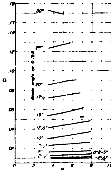
FIGURE 14. Variation of static power coefficient with tip-speed ratio and blade angle. Propeller No. 2, R, 2 Blade.
