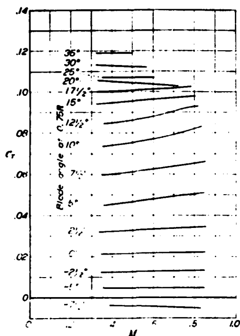
FIGURE 5. Variation of static thrust coefficient with tip-speed ratio and blade angle. Propeller No. 9, 2 blades.
