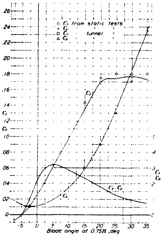
FIGURE 24 Characteristics of 3-blade propeller 5608. Rot at zero V , n/D = 0.5
