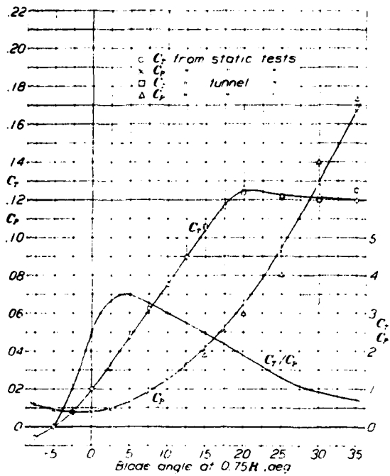
FIGURE 22 Characteristics of 2-blade propeller 5608. Rot at zero V , n/D = 0.5
