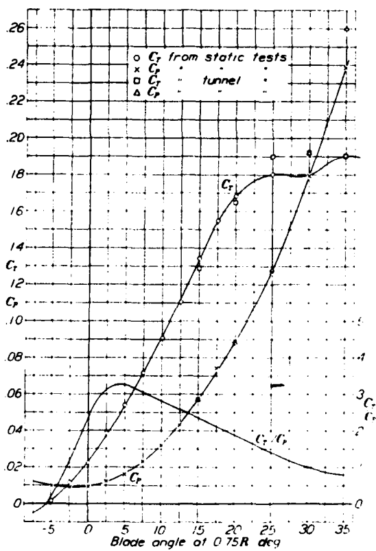
FIGURE 25 Characteristics of 2-blade propeller 37-3047 at zero V , n/D = 0.5
