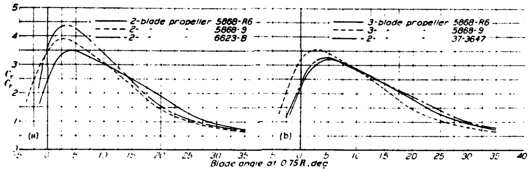
FIGURE 28.- Comparison of propeller characteristics. C_T/C_P against blade angle; V \propto D, 0; M, 0.5 .
