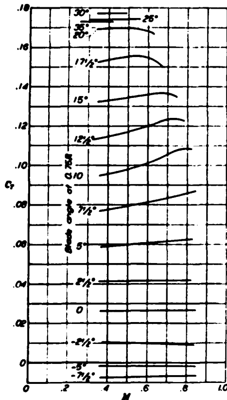
FIGURE 10—Variation of static-thrust coefficient with tip-speed ratio and blade angle Propeller No. 1B, 3 blades
