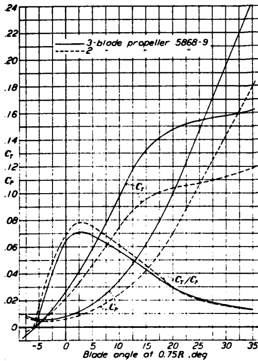
FIGURE 26.- Comparison of static aerodynamic characteristics of 2-blade and 3-blade propellers. M, 0.5 .
