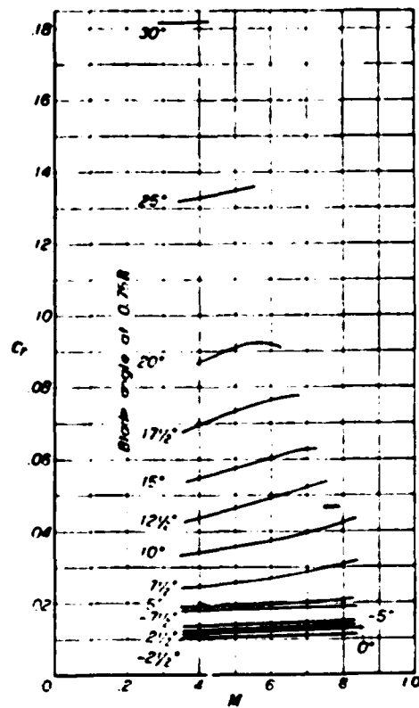
FIGURE 11—Variation of static-power coefficient with tip-speed ratio and blade angle Propeller No. 1B, 3 blades
