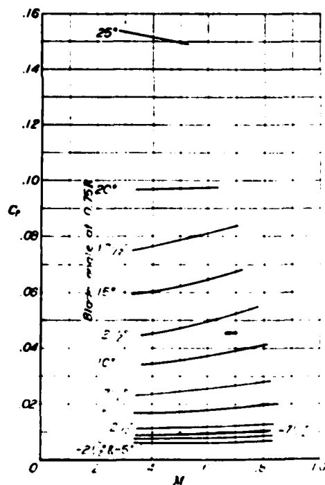
FIGURE 8. Variation of static power coefficient with tip-speed ratio and blade angle. Propeller No. 9, 3 blades.
