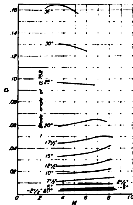
FIGURE 12. Variation of static power coefficient with tip-speed ratio and blade angle. Propeller No. 1, R, 2 Blade.
