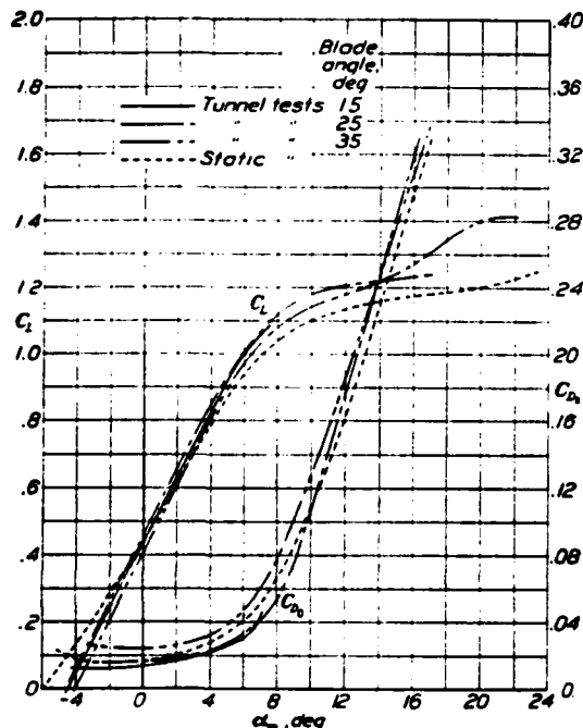
FIGURE 32.—Comparison of lift and drag coefficients obtained from wind-tunnel and static tests for 2-blade propeller 5063.9
