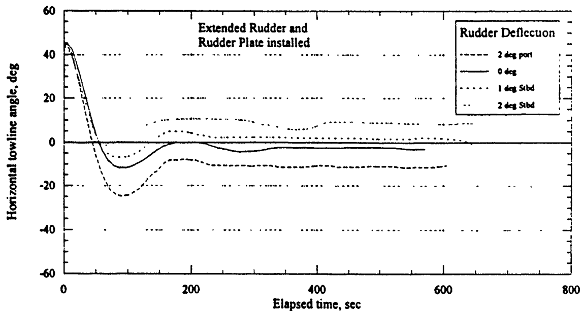
Fig. 20. Effect of rudder deflection on SSN-688 class at 5650 LTSW displacement, 0.75 ft (0.23 m) GM and 7.5 ft (2.29 m) trim down by the stern at 4 kn.
