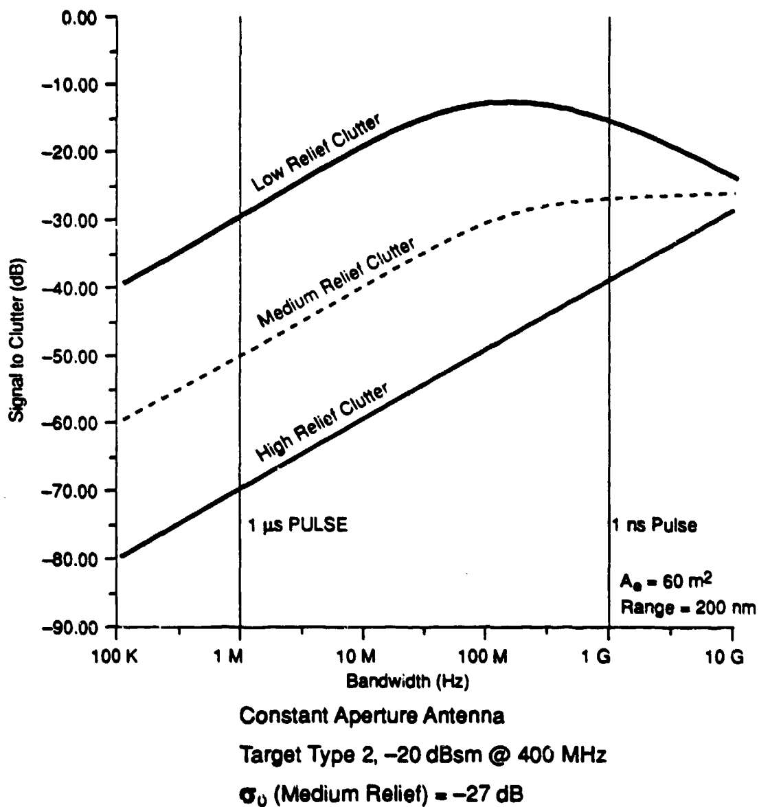
FIGURE H-6. SIGNAL BANDWIDTH EFFECT ON SIGNAL/CLUTTER
