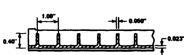
Typical Cross Section Machined from Flat Plate
