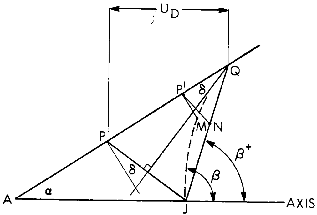
Figure 3. The Collapse Process for a Variable Collapse Velocity Liner, PER [2].
