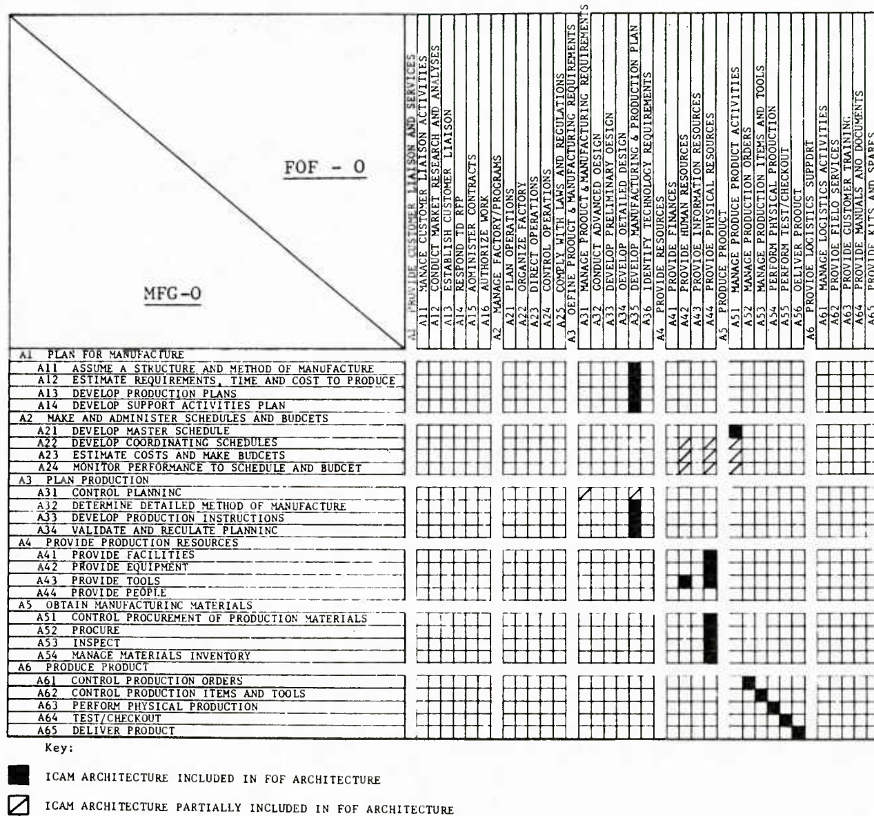
Figure 6-3 Relationship ICAM Manufacturing Architecture (MFG0) versus FoF Architecture
