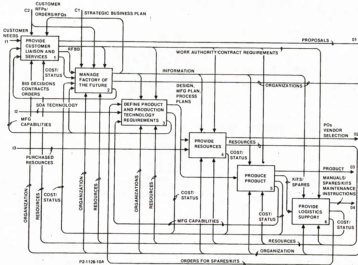
Figure 3-1 Factory of the Future Generic Functions
