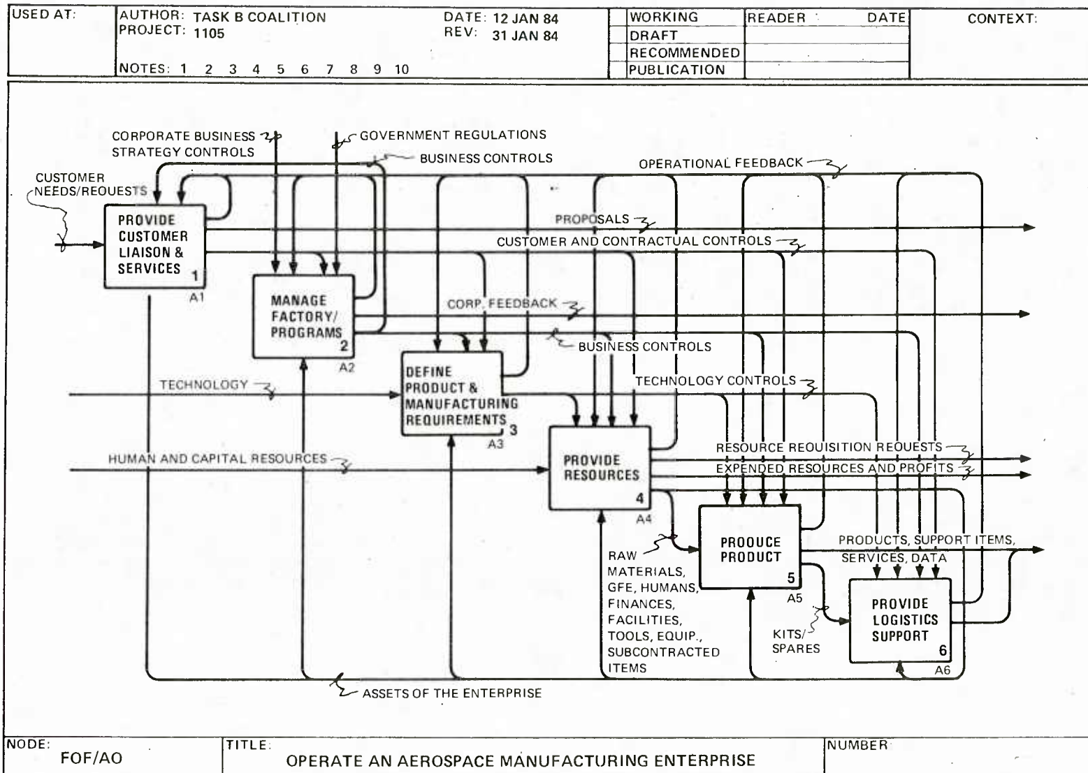
Figure 3-5 Operate an Aerospace Manufacturing Enterprise
