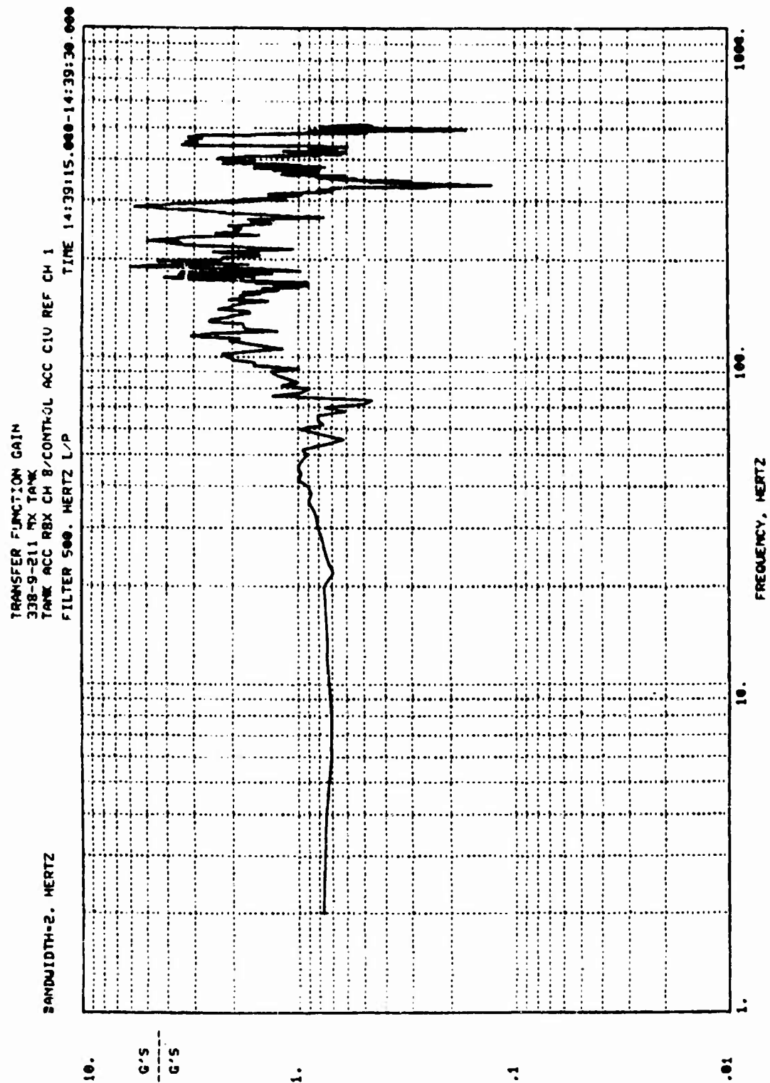
Figure 195. Pressurant Boss X-Axis Gain
