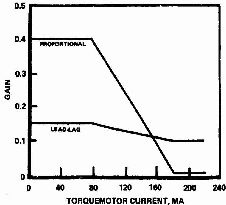
Figure 60. Gain Schedule
