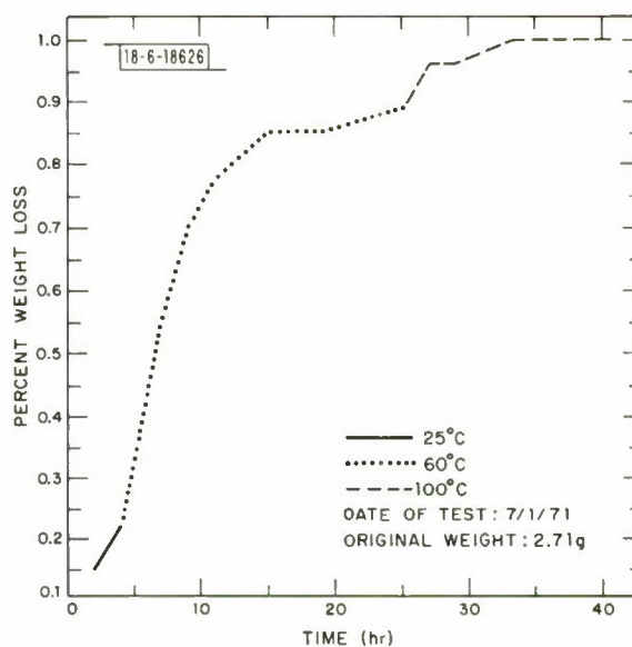
Fig. 12. Vacuum outgassing of a graphite epoxy laminate.
