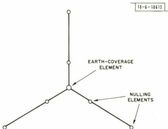
Fig. 1. 7-element double-triangle array.
