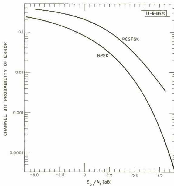
Fig. 7. Bit probability of error performance for PCSFSK.
