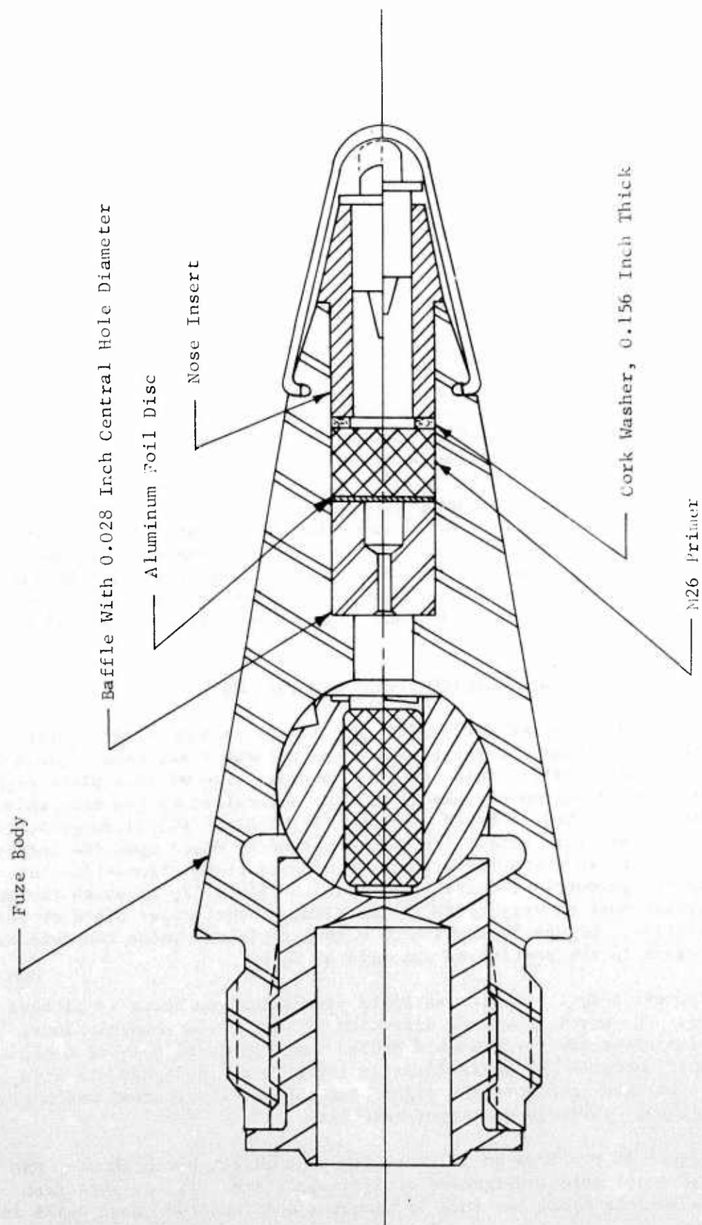
Figure 28. Delay Fuze Assembly Used for Rounds 1 - 7 Inclusive
