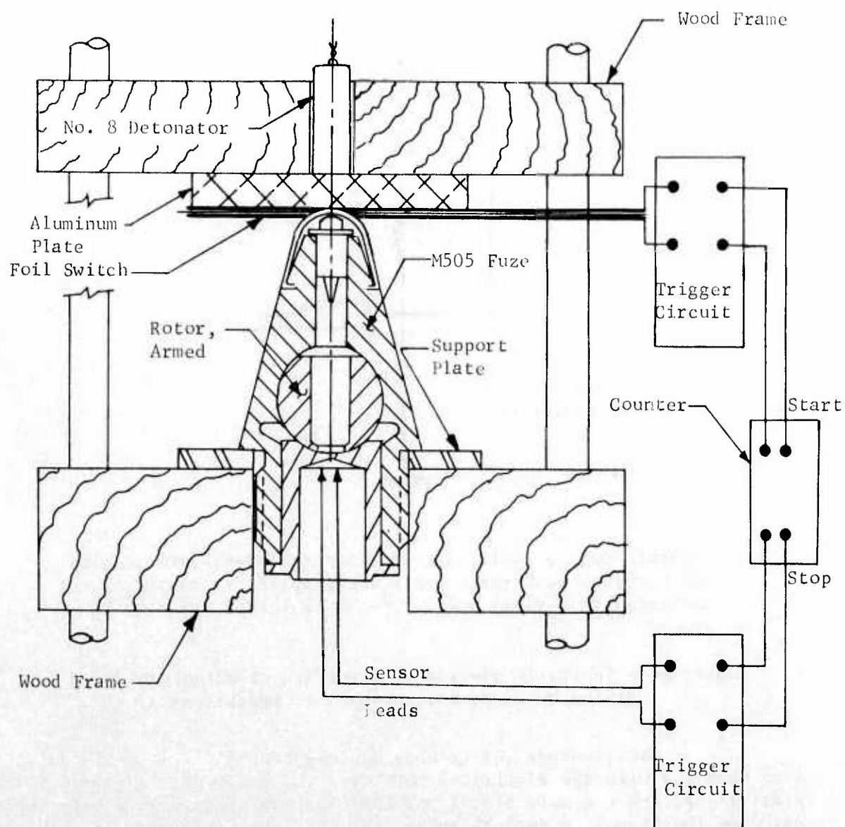
Figure 15. Schematic of Test Assembly for Quasi-Dynamic Fuze Delay Time Measurements
