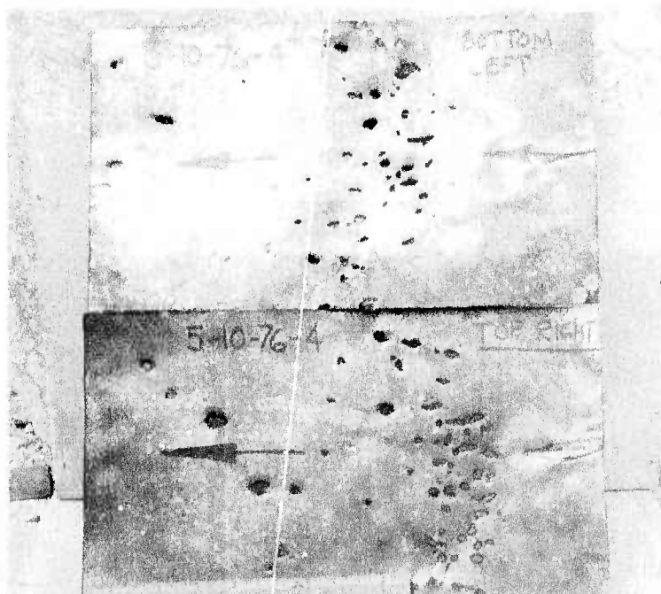
Figure 31. Characteristic Small 1-Inch-Diameter Petalled (1-P) Target Hole and Side Witness Plate Signature Obtained With Delay Fuze Functioning
