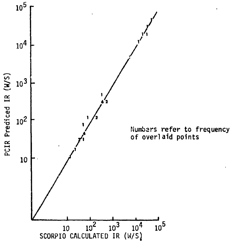
Figure 5: Comparison of PCIR Predicted and SCORPIO Calculated IR source Radiation at 90° Aspect Angle for the 4.0-4.8 \mu m Wavelength CO 2 Band.
