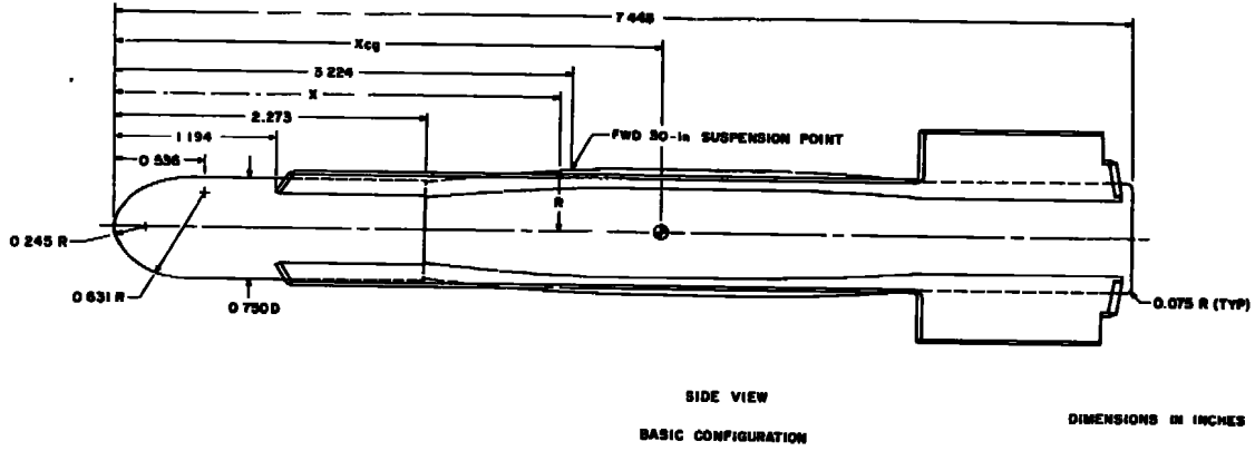
Figure 6. Details of the GBU-8 model.
