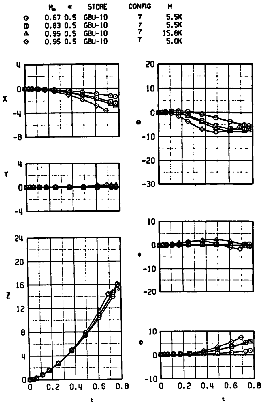
Figure 23. Separation characteristics of the GBU-10 from the F-15 aircraft.
