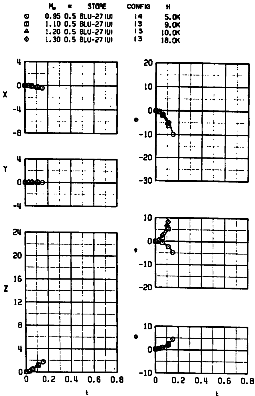
b. M_\infty = 0.95, 1.1, 1.2, \text{ and } 1.3 Figure 25. Concluded.
