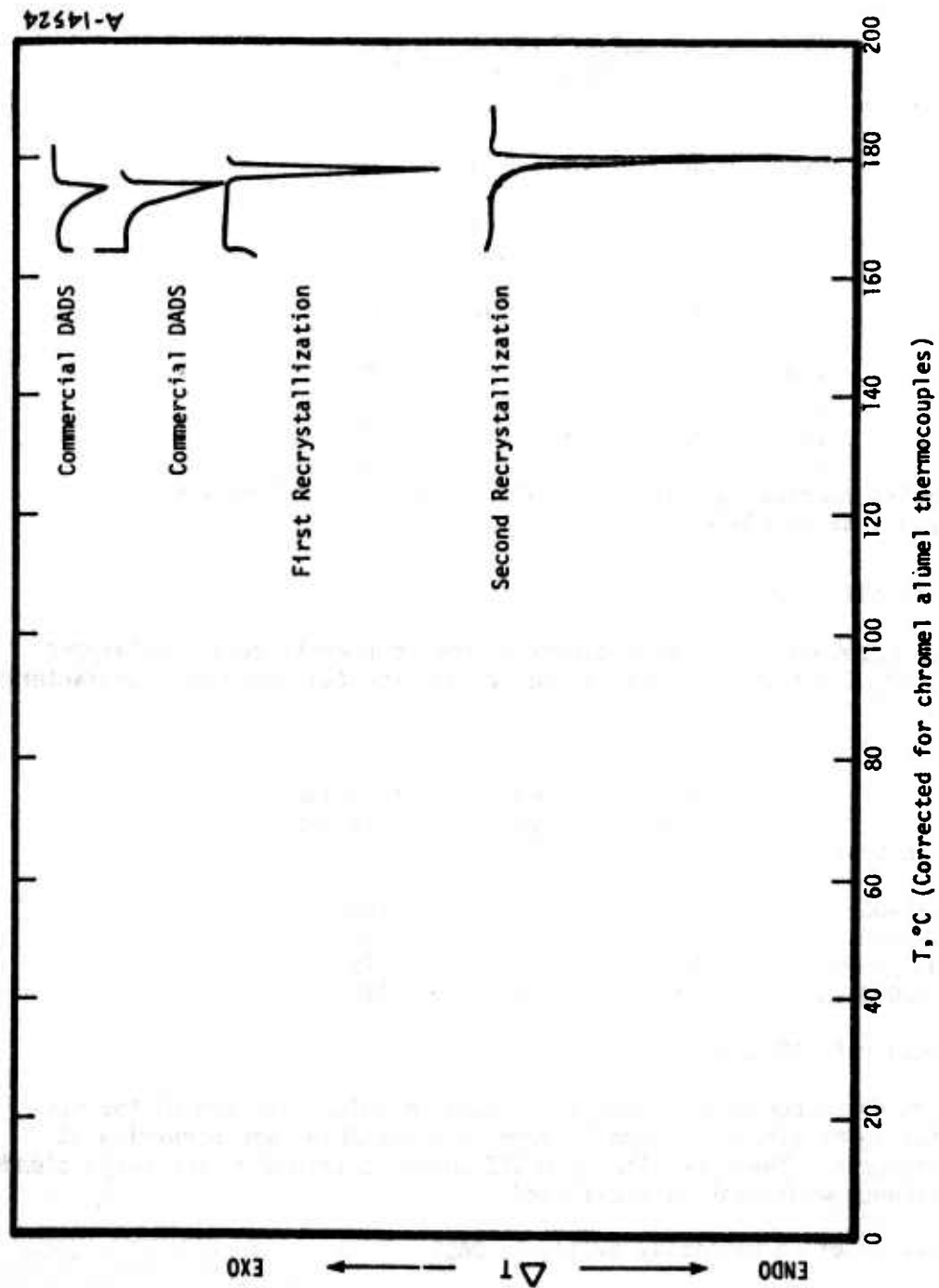
Figure 11. DSC of DADS ( \Delta T = 2^\circ\text{C}/\text{min} ).
