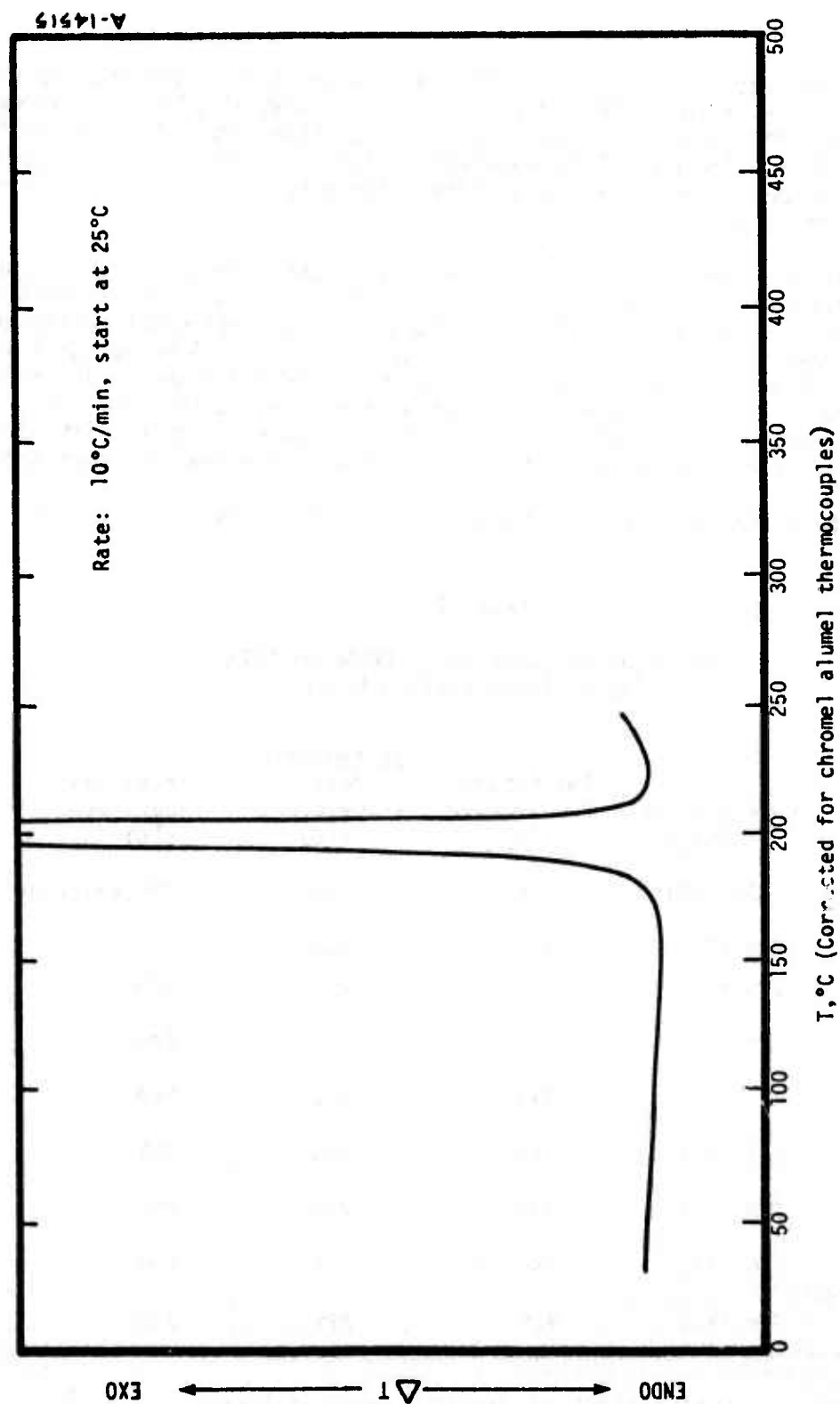
Figure 2. Cure exotherm of Epon 828/IPH.
