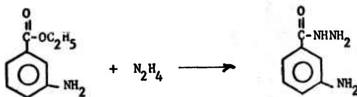
MABH
