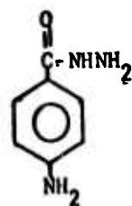
p-aminobenzhydrazide (PABH)
