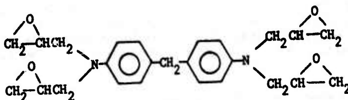
N,N,N',N'-Tetraglycidyl- 4,4'-methylenedianiline
