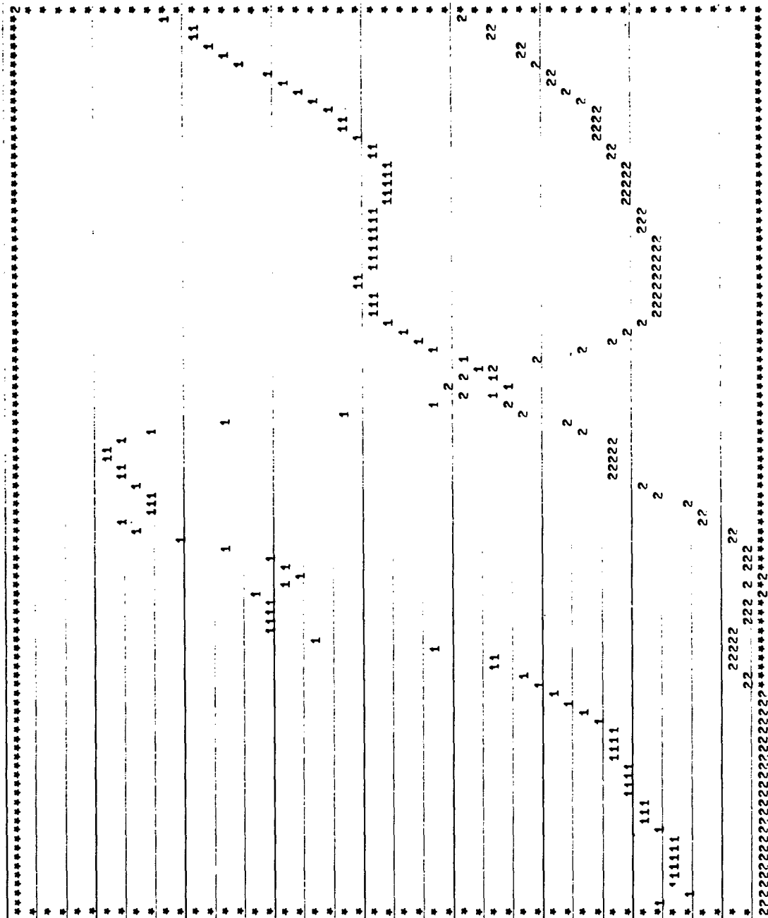
Figure 20. Temperature Behavior (Experiment No. 67) of Ions m/e 19, 20
