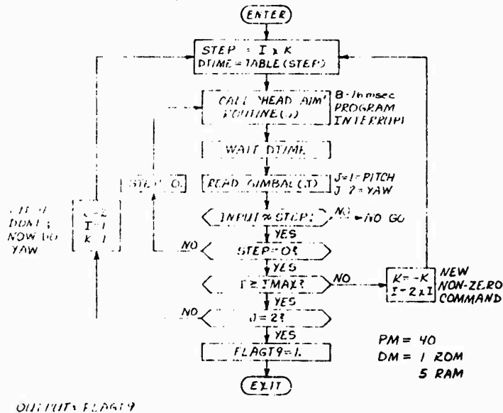
Figure 94. Target Seeker Gimbal Test Module SU-1, Flow Diagram
