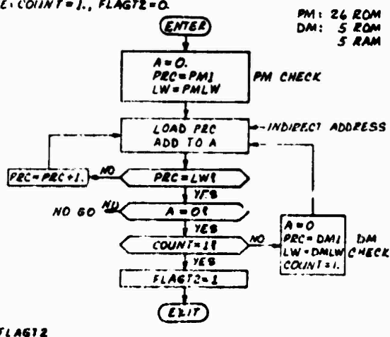
Figure 88. Computer Program Memory Test Module ST-2, Flow Diagram
