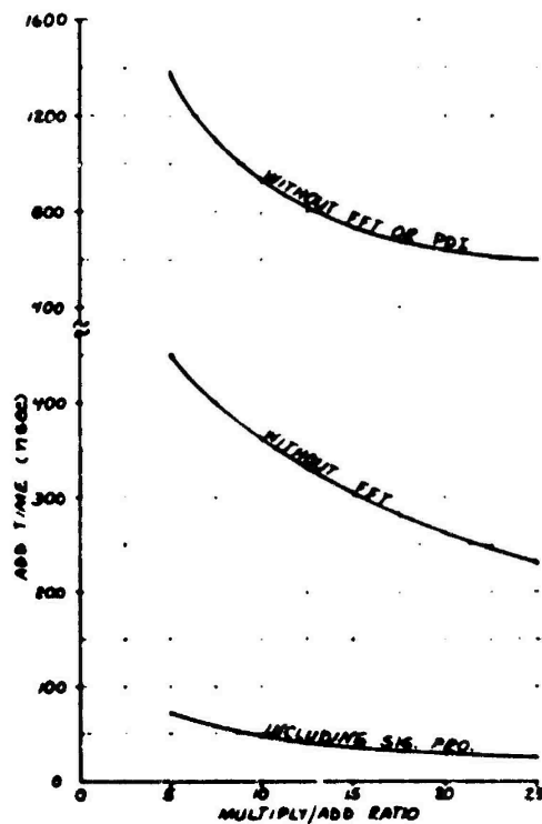
Figure 139 Computer Multiply/Add Time Ratio vs Add Time -
