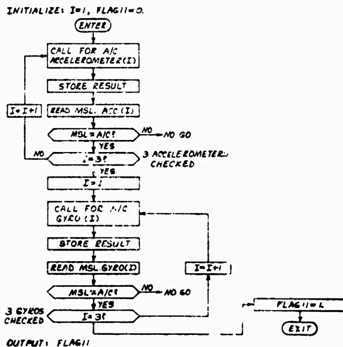
Figure 95. Inertial Sensor Test Module SU-3, Flow Diagram
