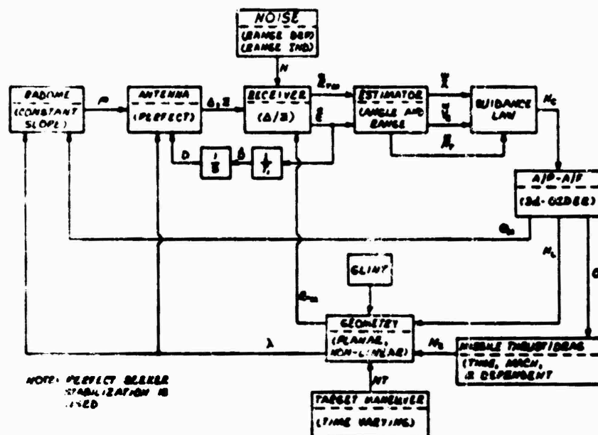
Figure 98 Guidance and Estimation Simulation Model
