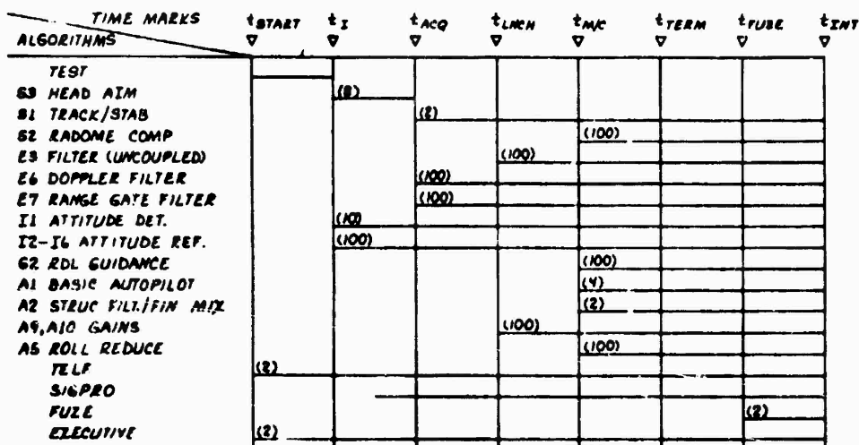
Figure 130 Function Time Line Diagram - Class I (Max.) Missile
