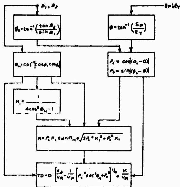
Figure 66 Time Delay Program Module F-2, Flow Diagram
