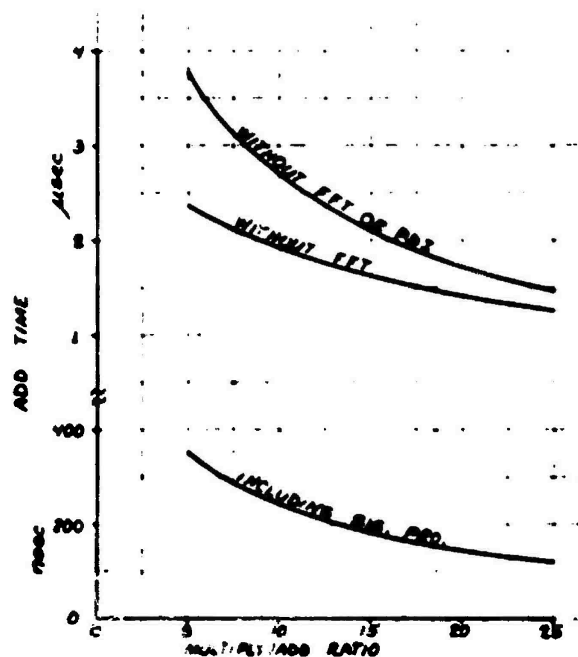
Figure 13b Computer Multiply/Add Time Ratio vs Add Times -
