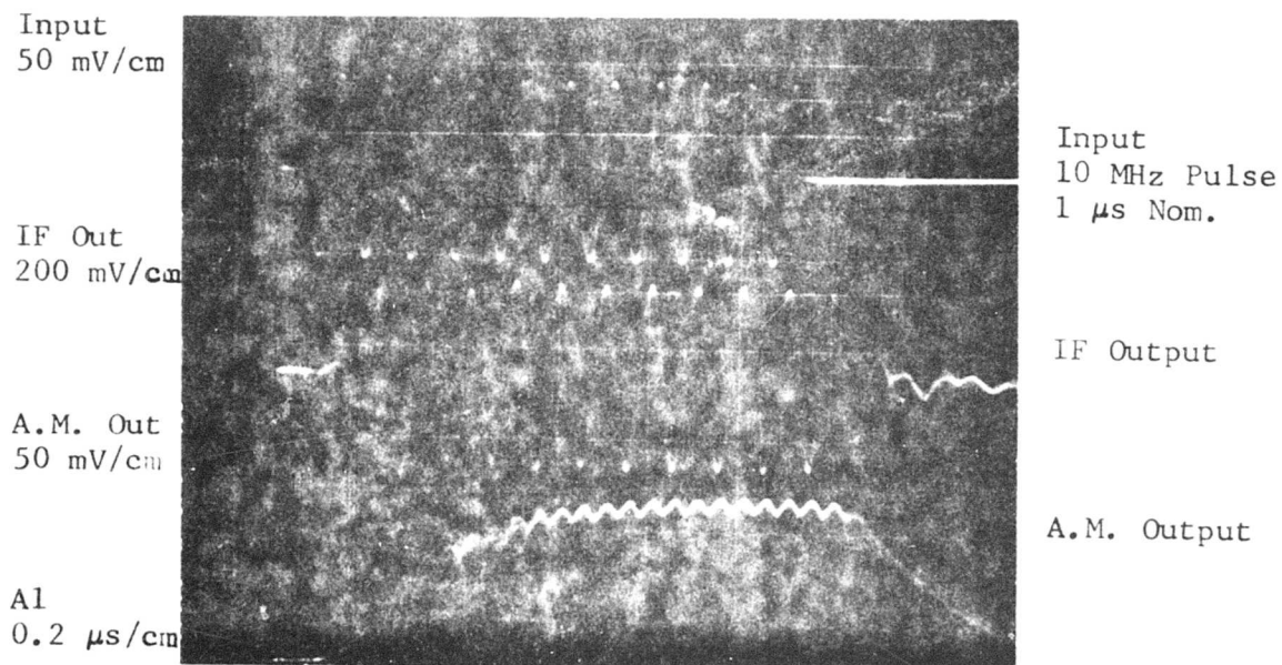
Figure 52 Amplifier output
