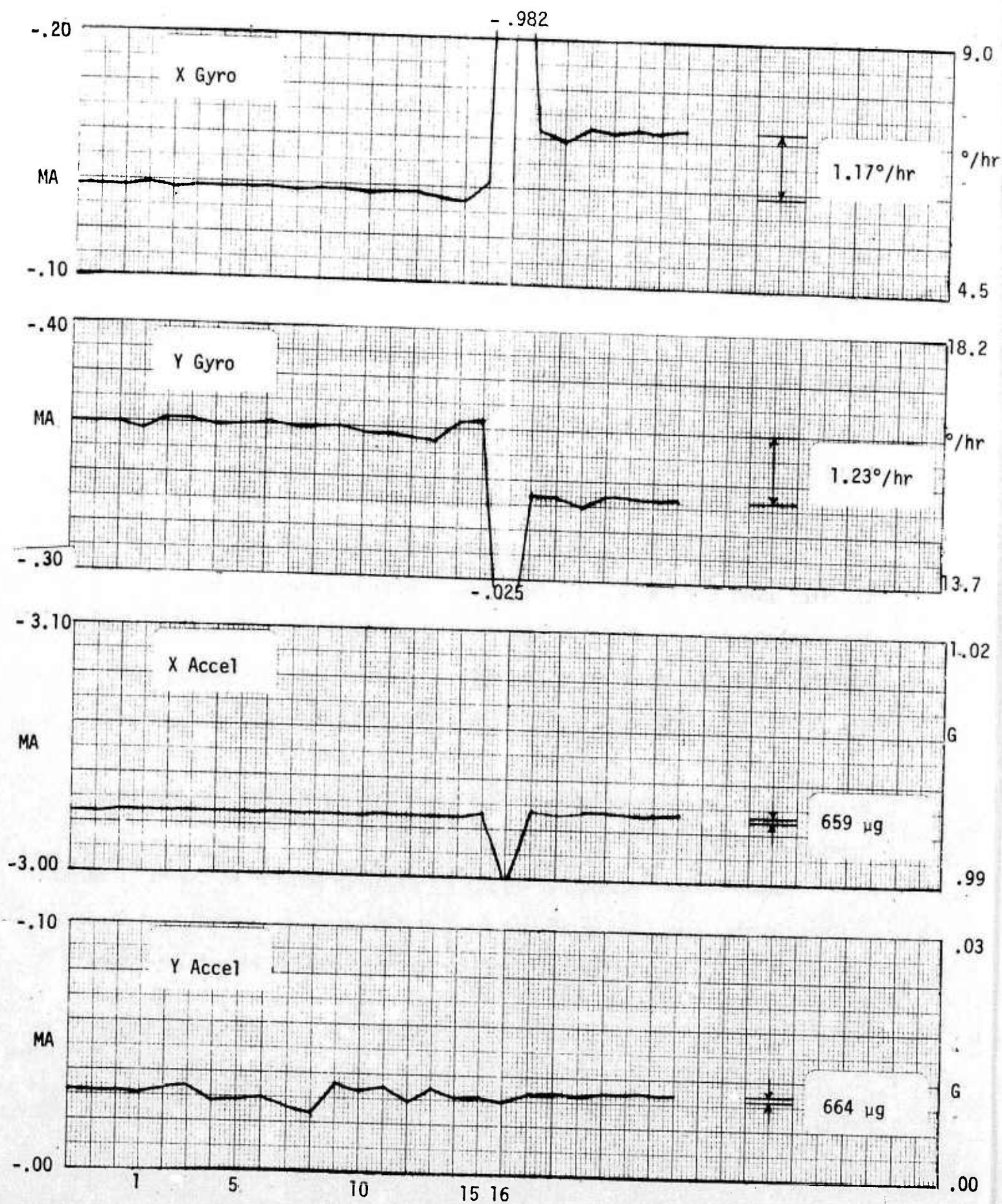
Figure B-1. Torquer Outputs - Vibration #1
