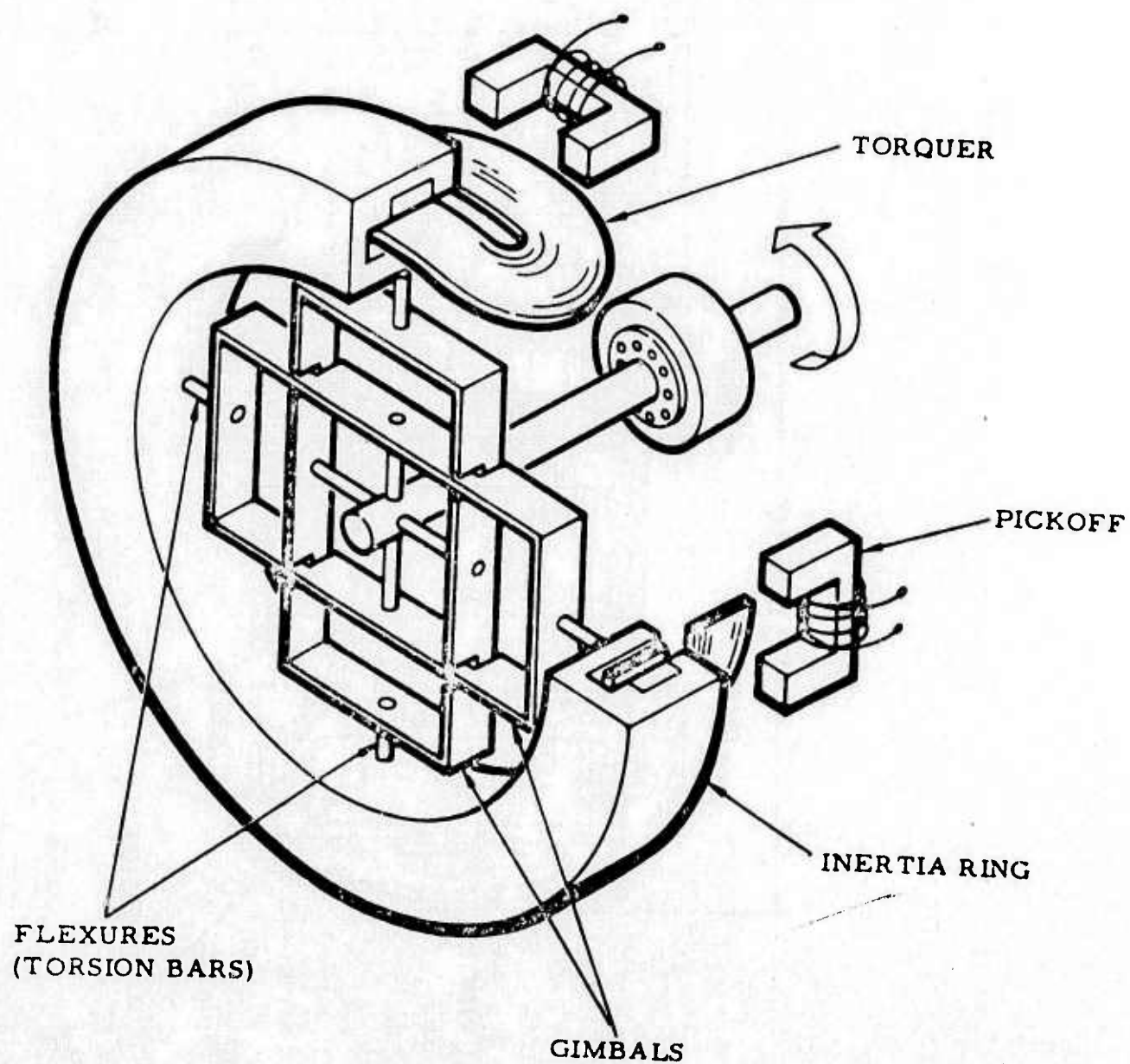
FIGURE 2. ROTOR SUSPENSION CONCEPTUAL VIEW
