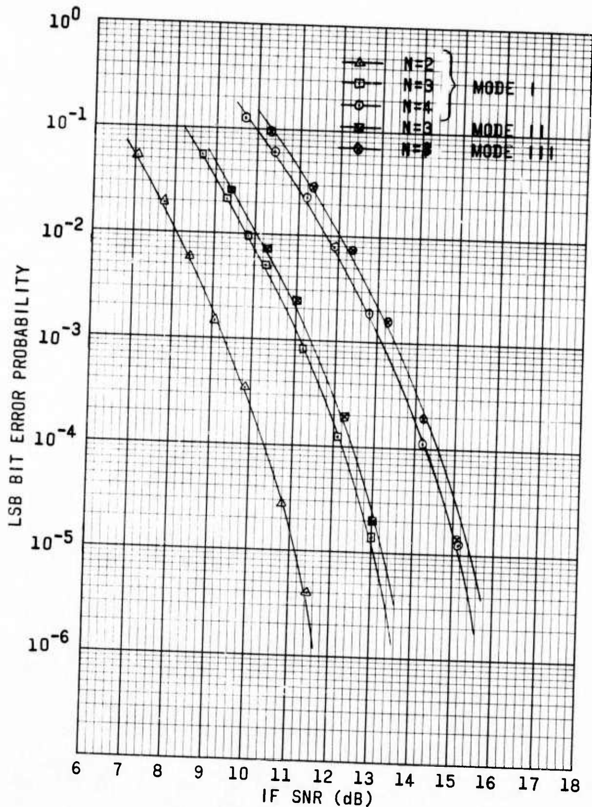
Figure 9. Variation in LSB BEP With IF SNR.
