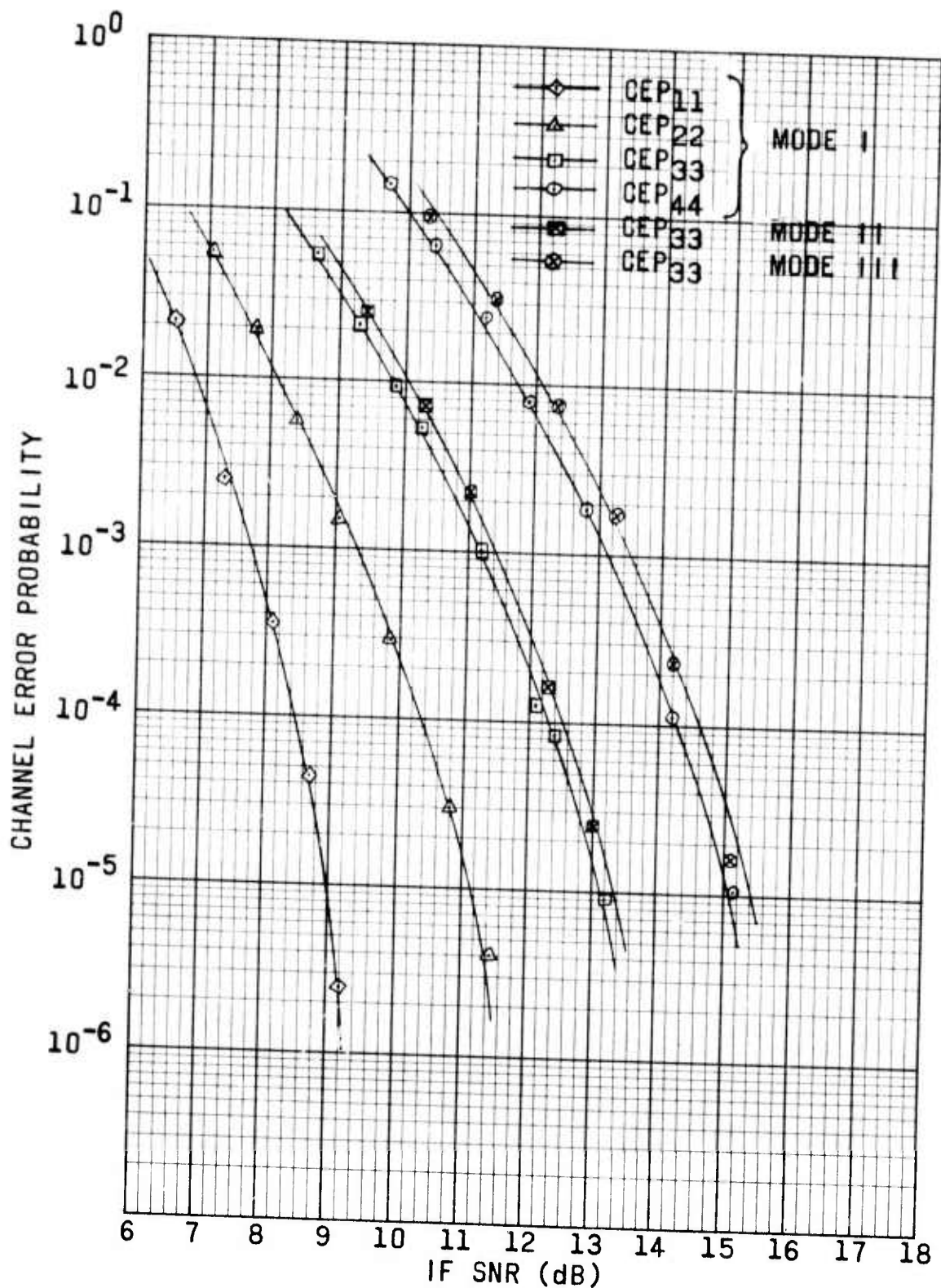
Figure 7. Variation in CEP With IF SNR.
