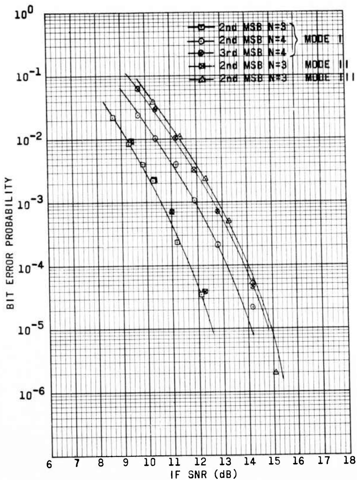
Figure 10. Variation of BEP of Middle Bits for N = 3 and 4 With IF SNR.
