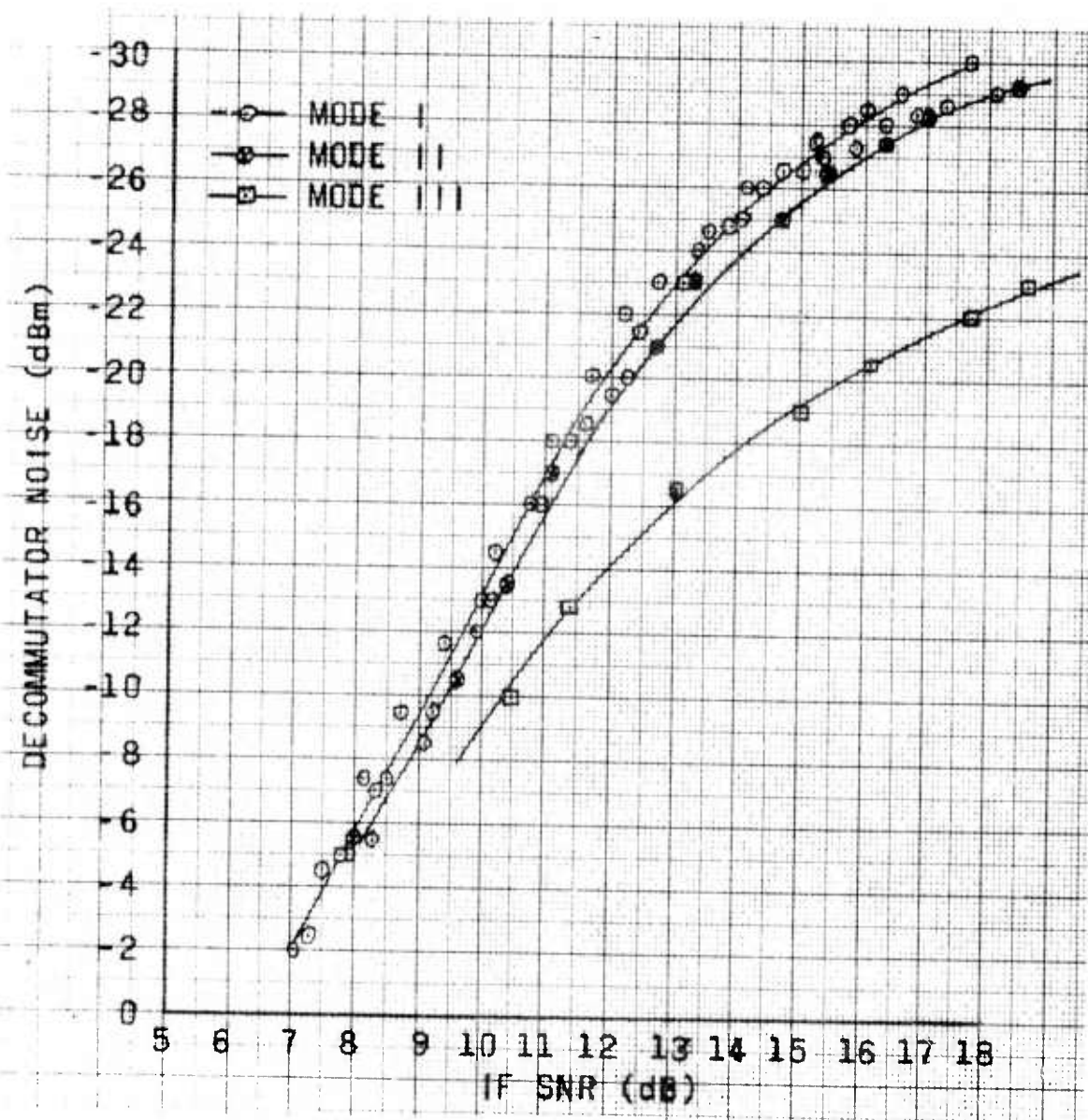
Figure 3. Relation Between Decommutator Noise and IF SNR.
