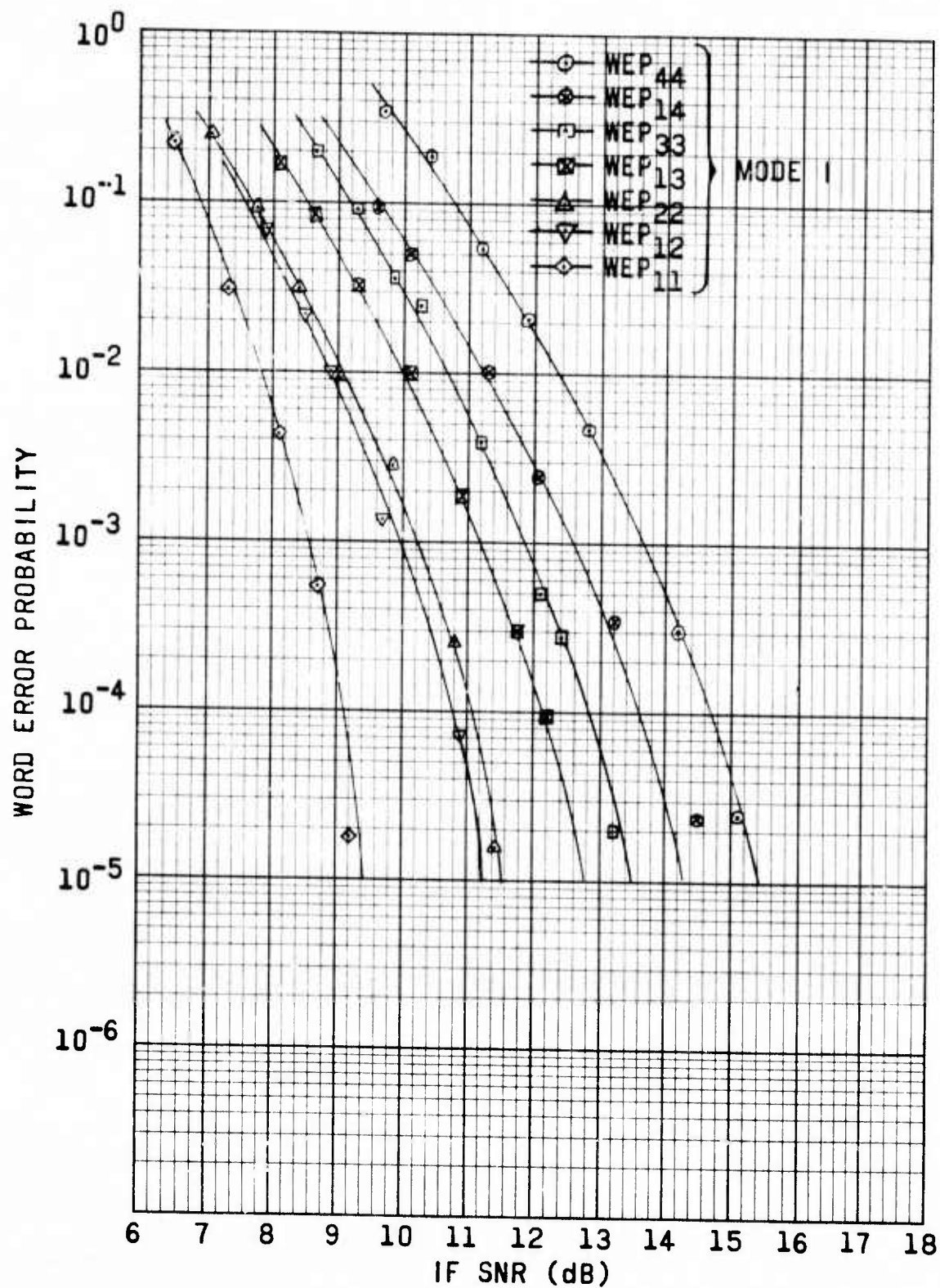
Figure 5. Variation of WEP With IF SNR for N Bits/Channel.
