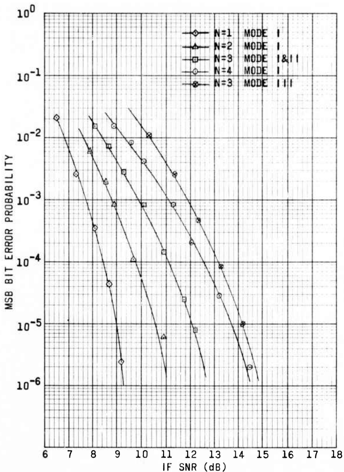
Figure 8. Variation in MSB BEP With IF SNR.
