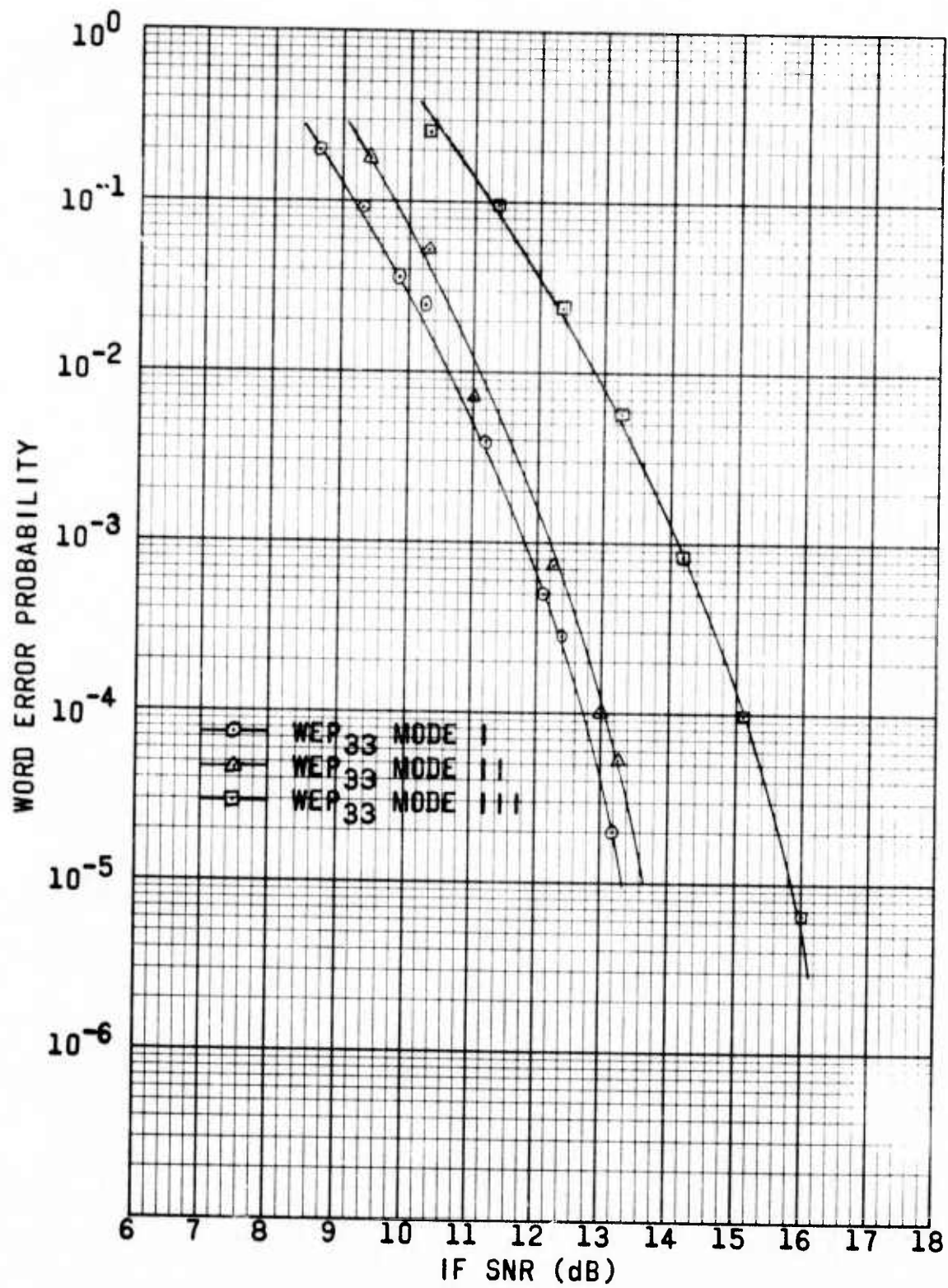
Figure 6. Variation in WEP With IF SNR for a Change in IF Bandwidth or Sample Rate.
