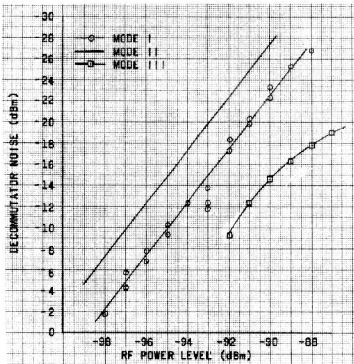
Figure 4. Relation Between Decommulator Noise and RF Power Level.
