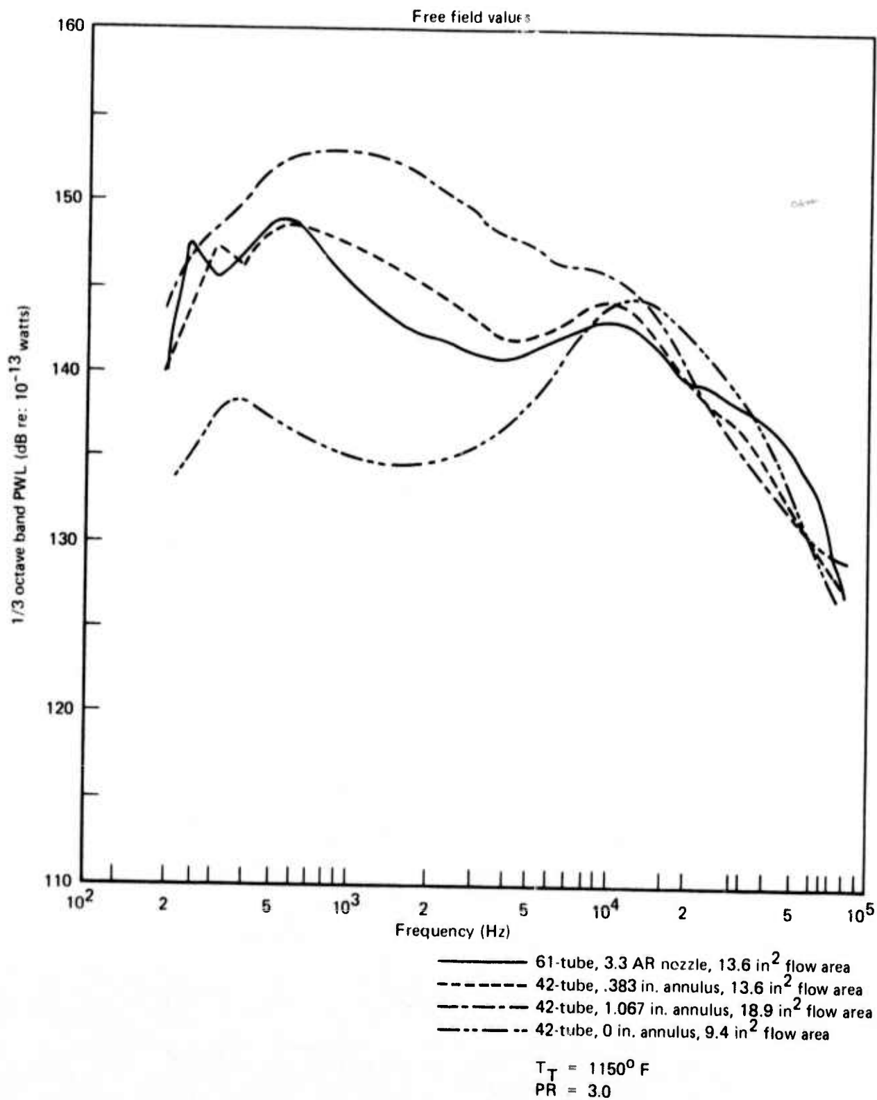
Figure 118. — Comparison of Regular Multitube Nozzle Noise With Multitube/Plug Nozzle Noise Levels
