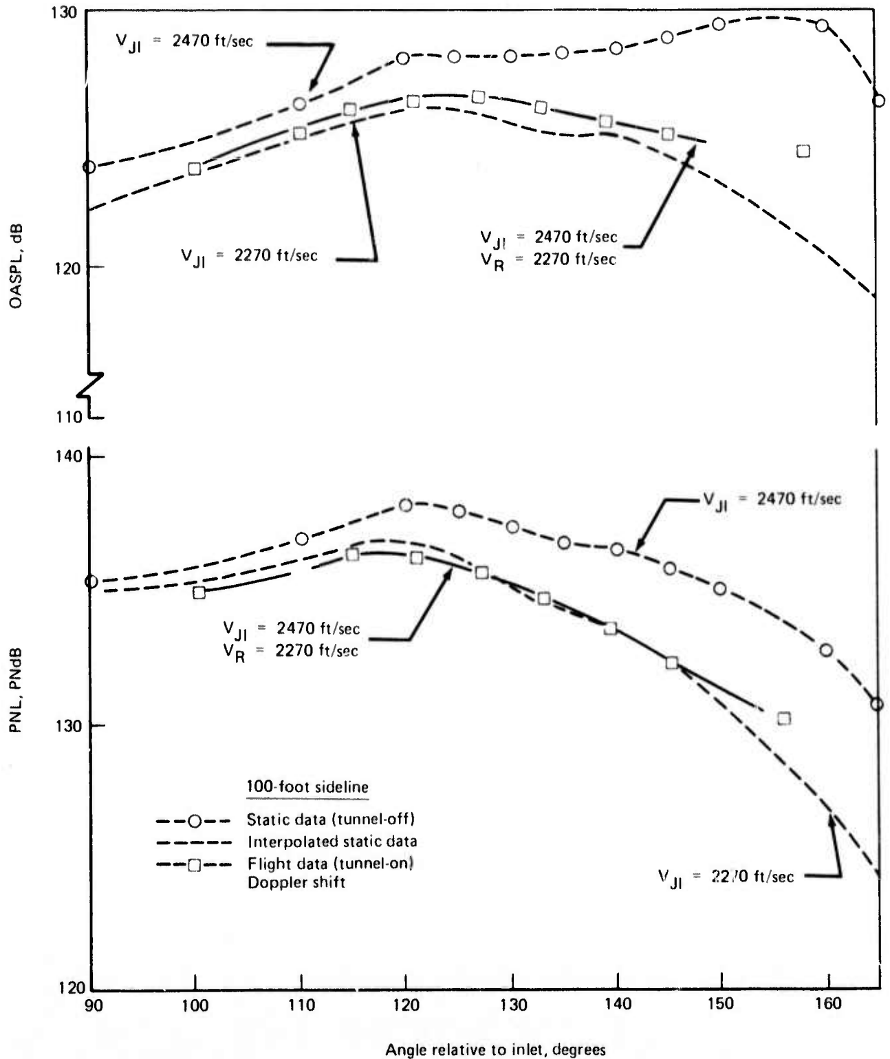
Figure 219.—9 ft by 9 ft Wind Tunnel Noise Test, OASPL and PNL Directivity, Static versus Flight, 37-Tube Nozzle (Ref) With AR 3.7 Shroud, PR 4
