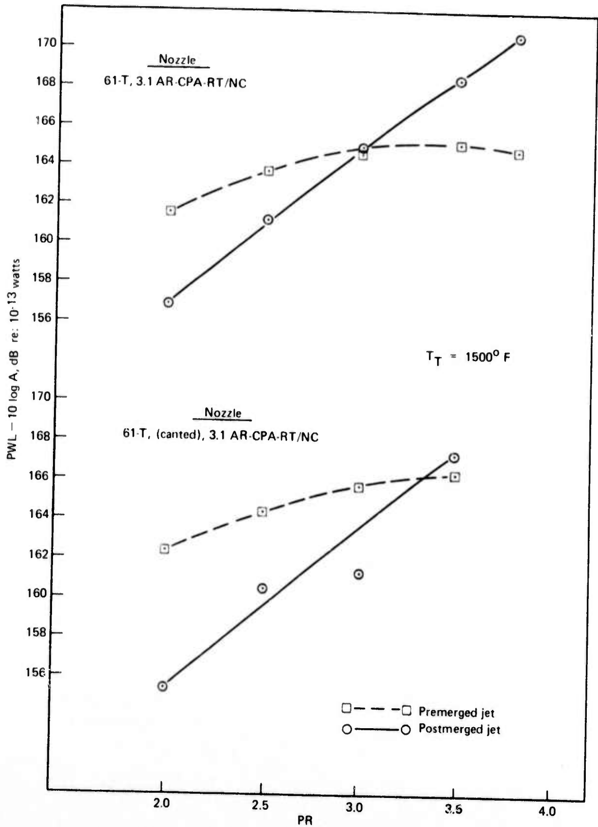
Figure 125. — 61-Tube and 61-Tube (canted) Nozzles Premerged and Postmerged Jet Noise Levels, T_T = 1500^\circ F
