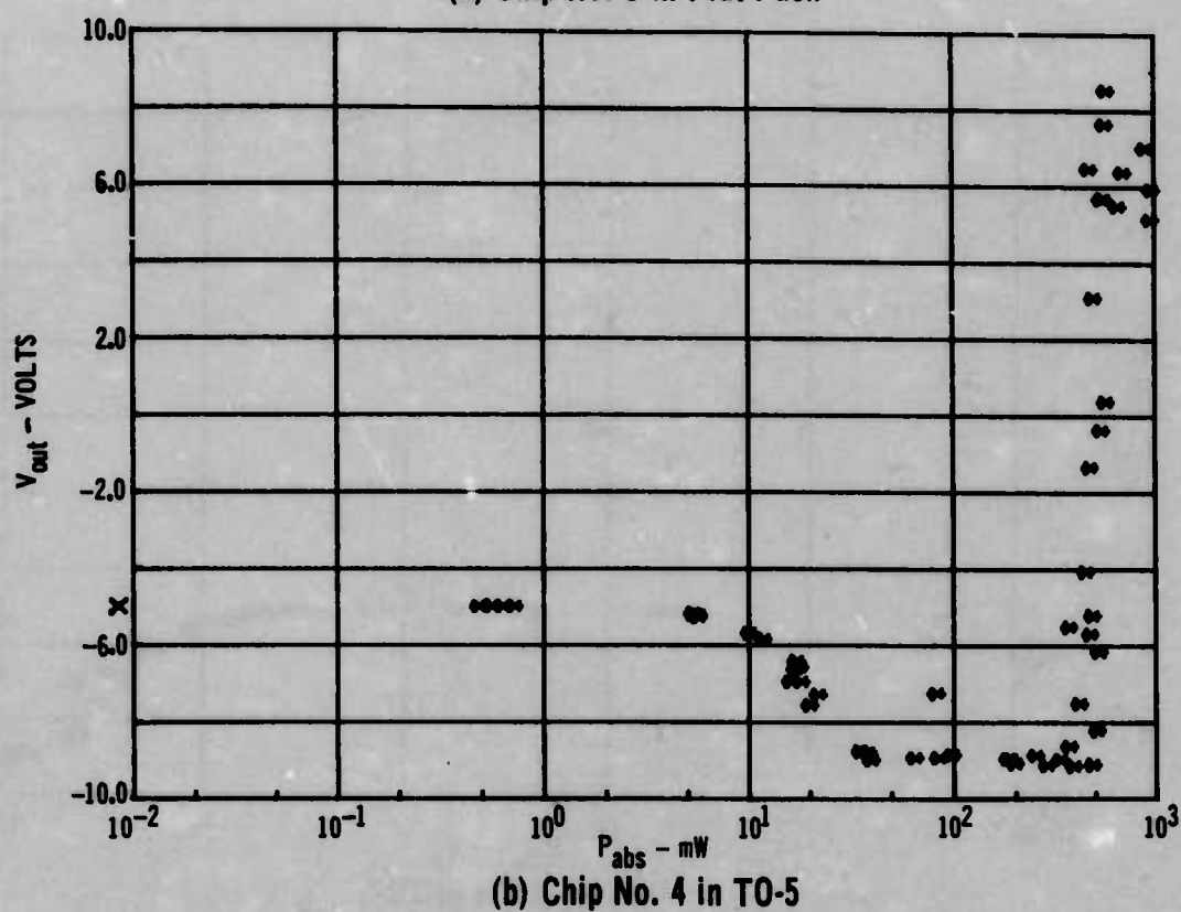
FIGURE A-12 741 FLAT PACK VS 741 TO-5 SUSCEPTIBILITY AT 5.6 GHz
