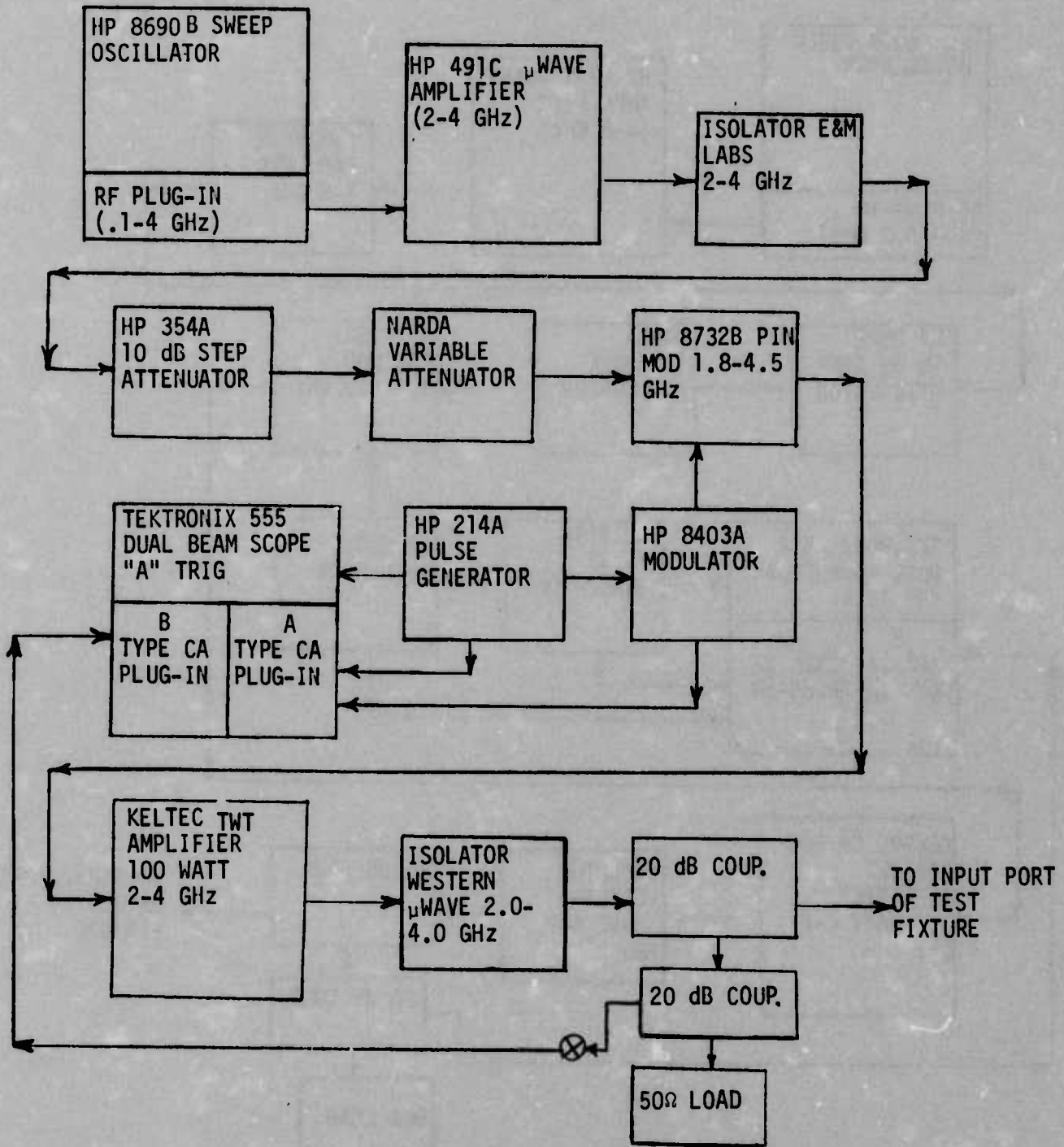
Figure 61 Test Setup for Catastrophic Failure Testing of 7400 and 741 at 3 GHz
