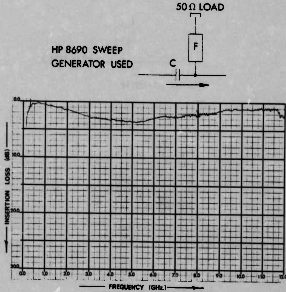
FIGURE 7 BIAS UNIT RF PATH INSERTION LOSS
