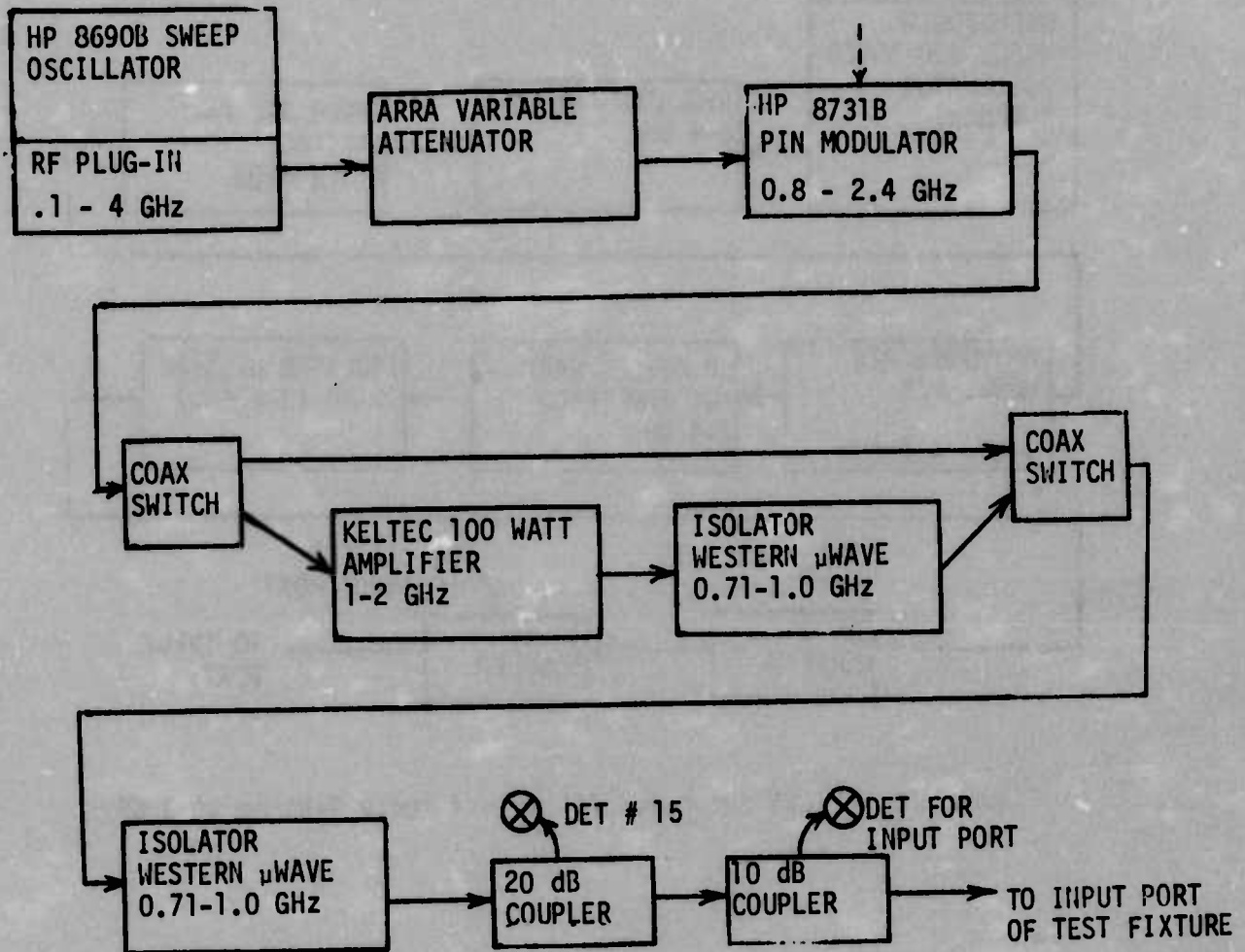
Figure 37 RF Test Setup for 741 Interference Testing at 0.91 GHz
