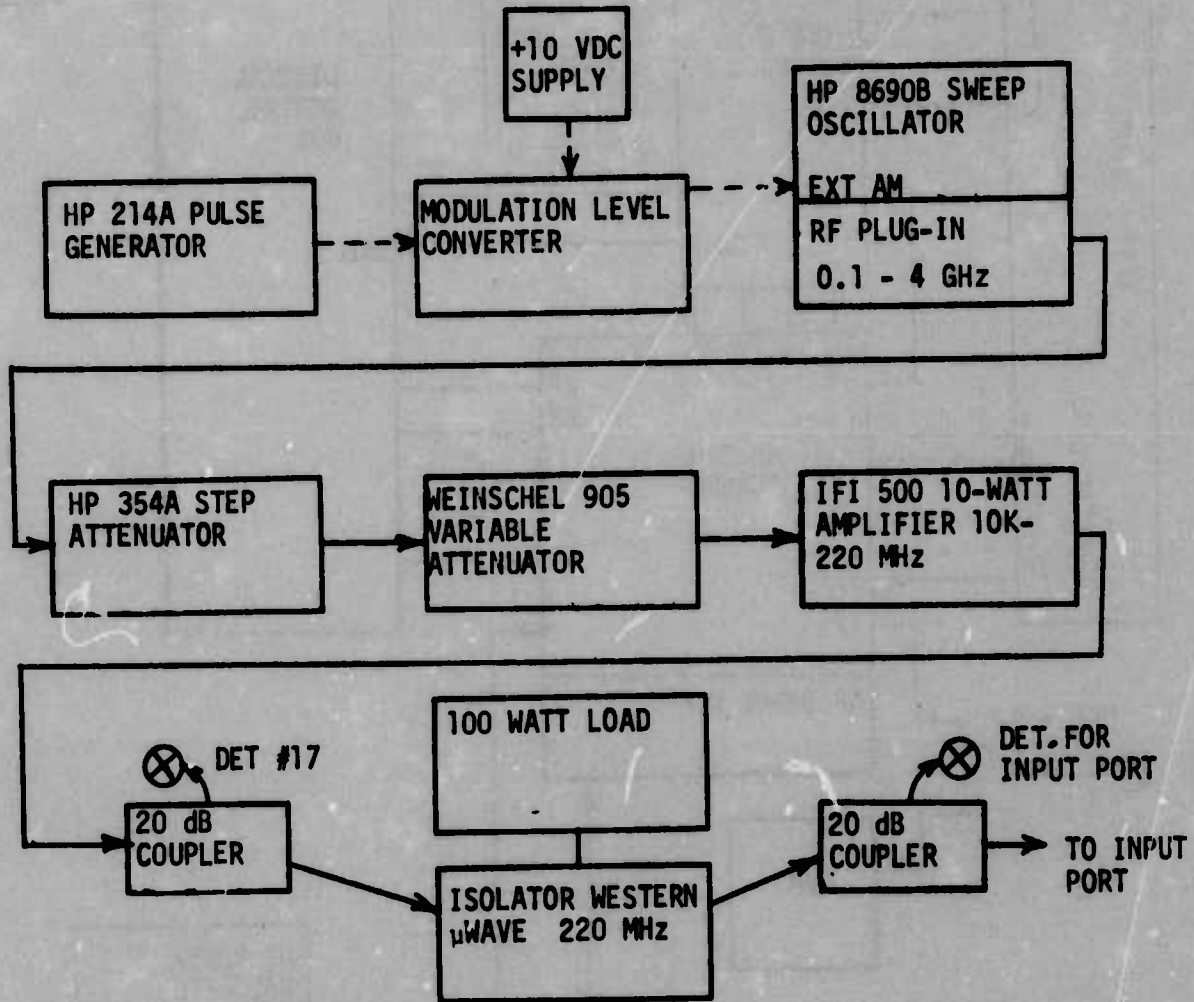
Figure 48 RF Test Setup for 2002 and Extra Digital Device Interference Tests at 0.22 GHz
