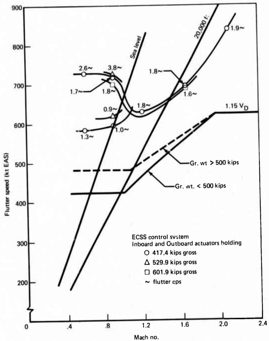
FIGURE 15.—SYMMETRIC HORIZONTAL STABILIZER FLUTTER BOUNDARIES, ACTUATORS HOLDING
