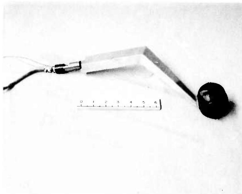
Figure 28. 400-Y-35-054 Internal Balance Sting
