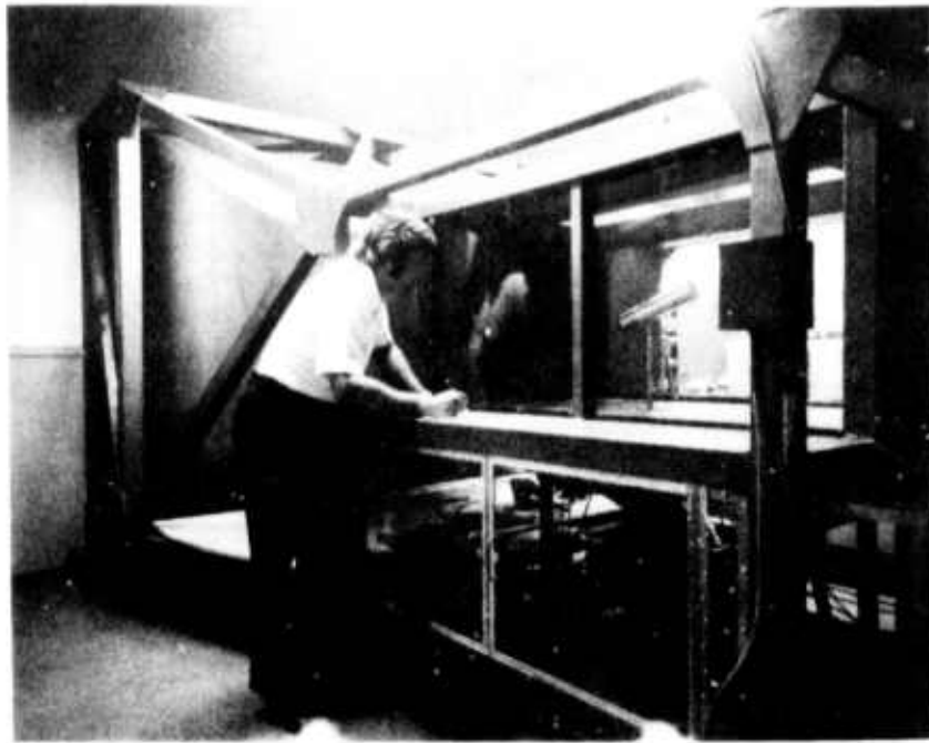
Figure 5. Wind Tunnel Settling Chamber, Contraction Cone, and Test Section
