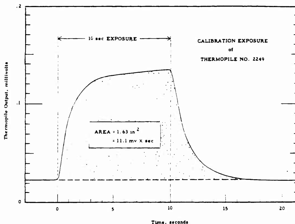
Figure 4.1 Typical total-thermal calibration trace for a 10-second exposure
