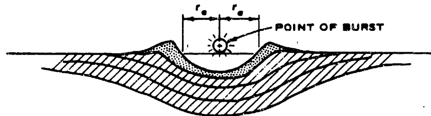
a. Conventional crater.
