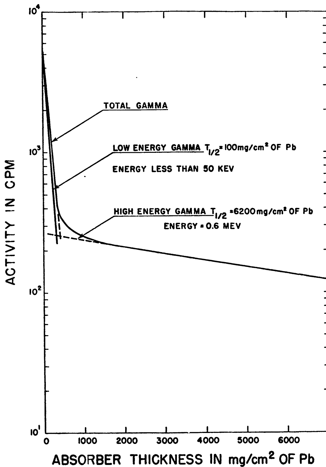
Fig. 5.4—Gamma-absorption curve.
