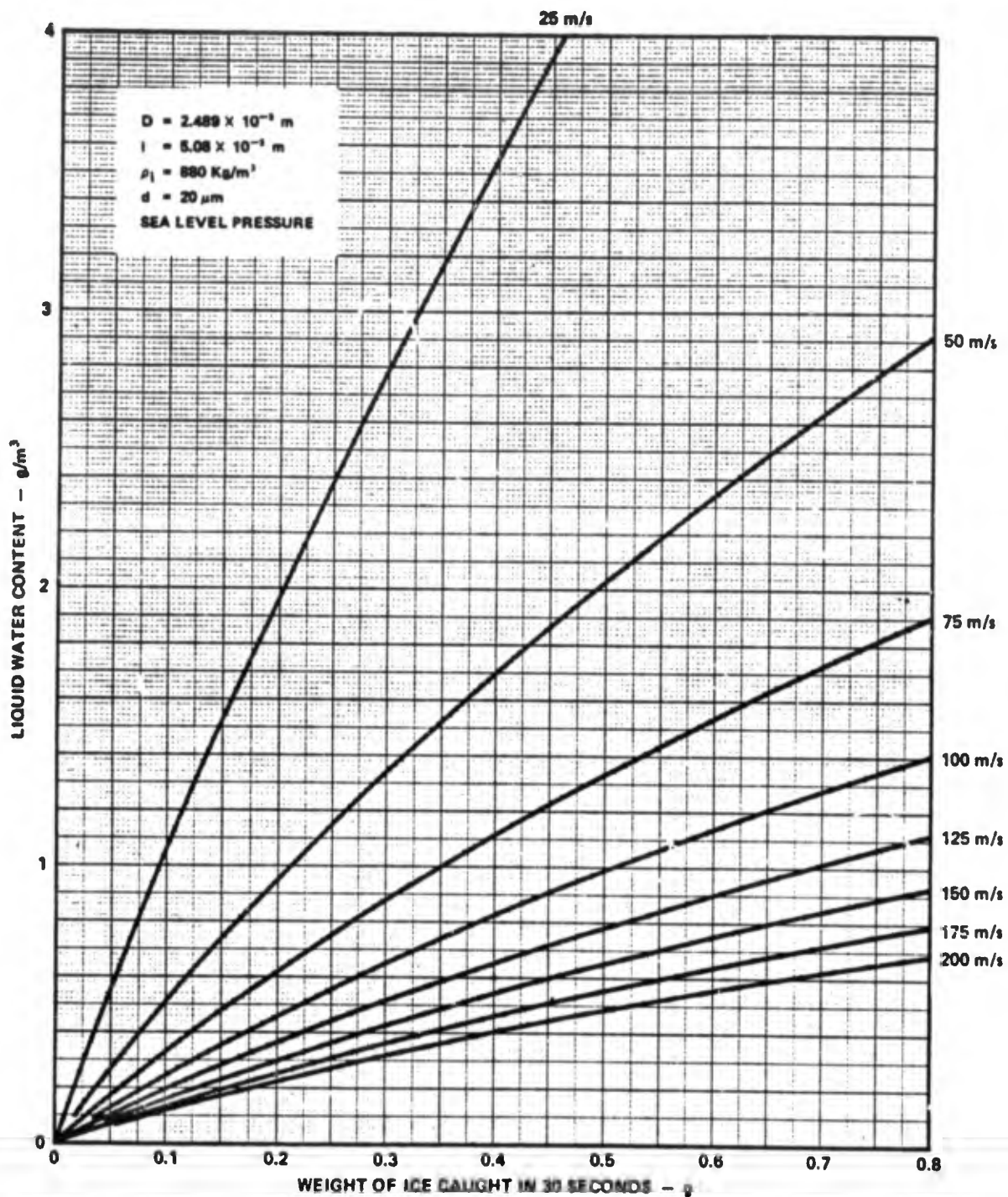
FIG. 6: LIQUID WATER CONTENT VERSUS WEIGHT OF ICE CAUGHT IN 30 SECONDS AT VARIOUS AIRSPEEDS BY ROTATING CYLINDER METHOD
