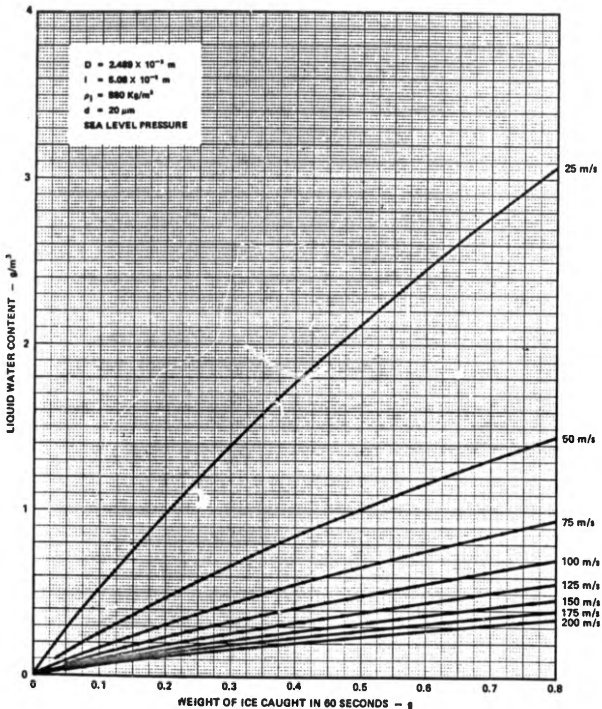
FIG. 5: LIQUID WATER CONTENT VERSUS WEIGHT OF ICE CAUGHT IN 60 SECONDS AT VARIOUS AIRSPEEDS BY ROTATING CYLINDER METHOD
