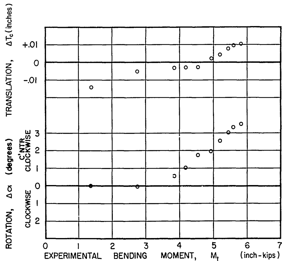
(b) ANGLE BEAM M-5, \theta = 60^\circ
