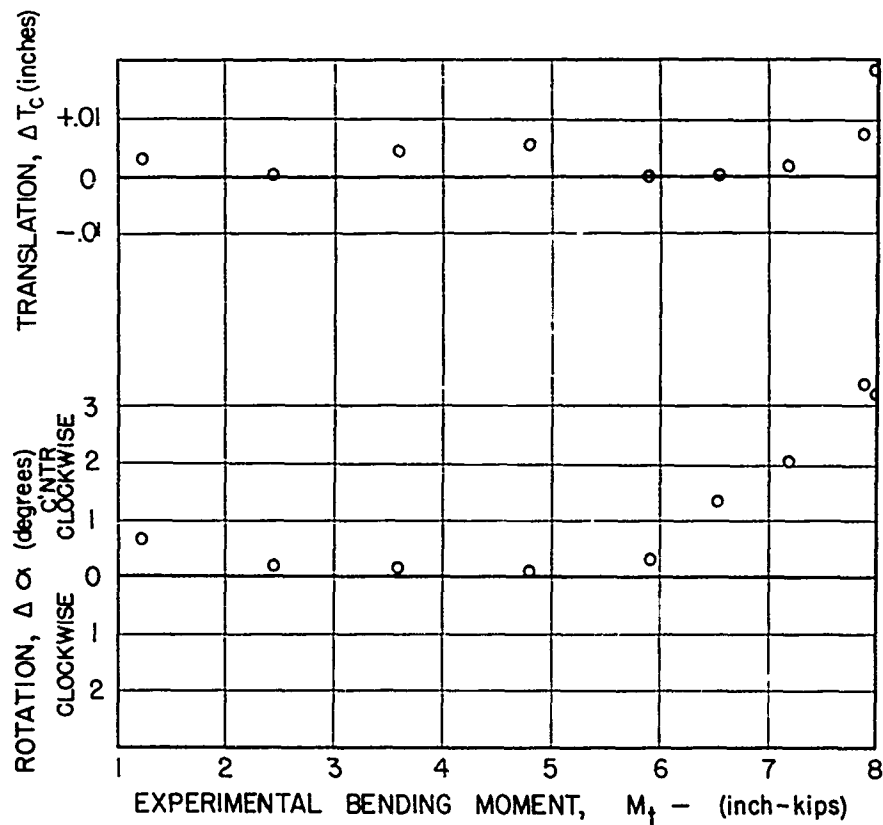
(a) ANGLE BEAM N-6, \theta = 30^\circ
