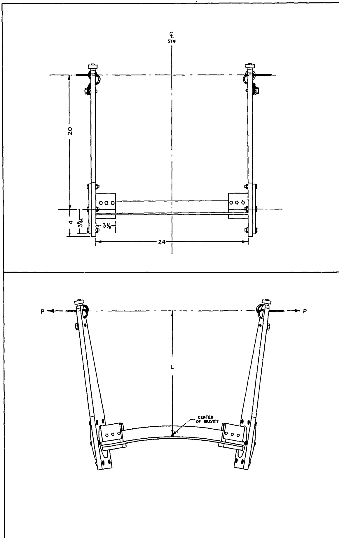
FIG. 7 — PLAN VIEW OF PLASTIC BENDING APPARATUS
