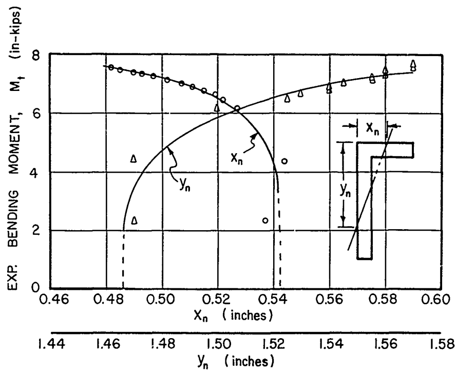
(a) ANGLE BEAM M-2, \theta = 30^\circ
