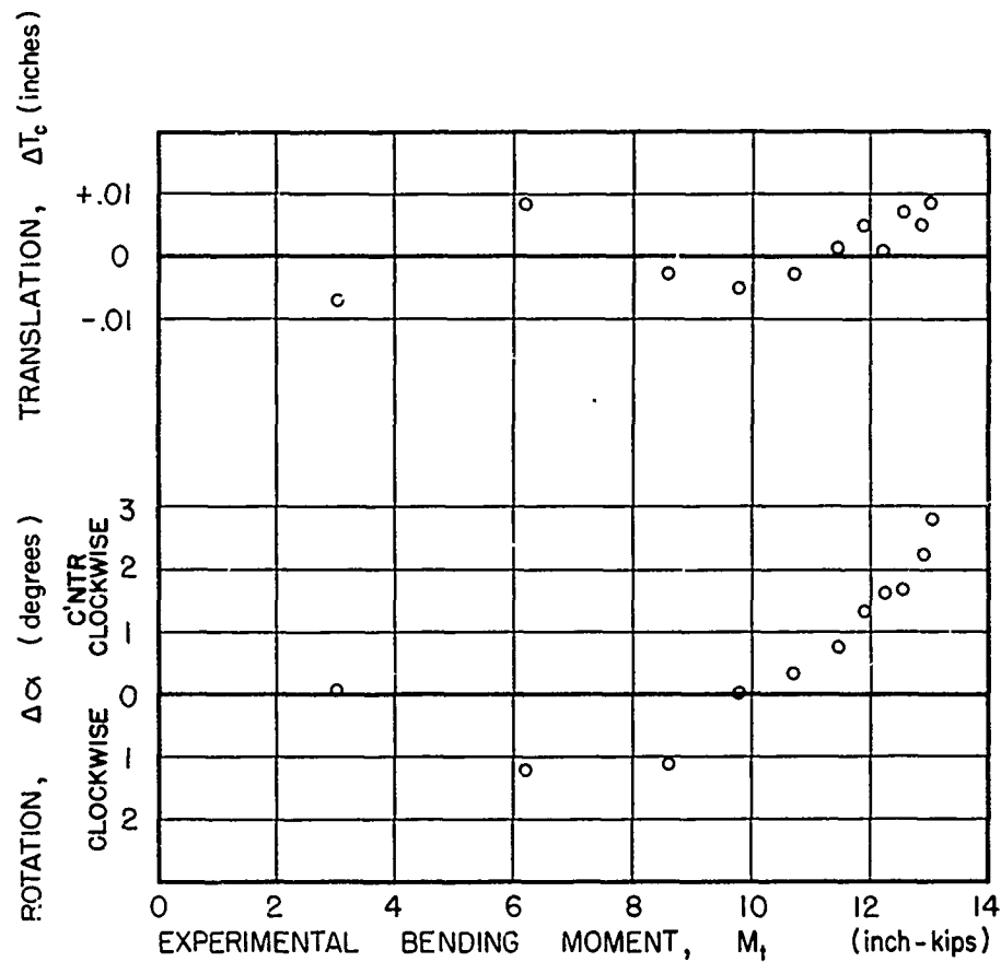
(a) ANGLE BEAM M-4, \theta = 0^\circ
