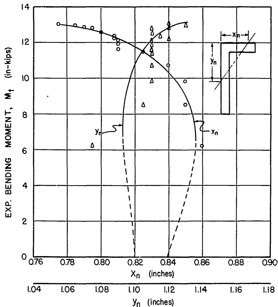
(a) ANGLE BEAM M-4, \theta = 0^\circ
