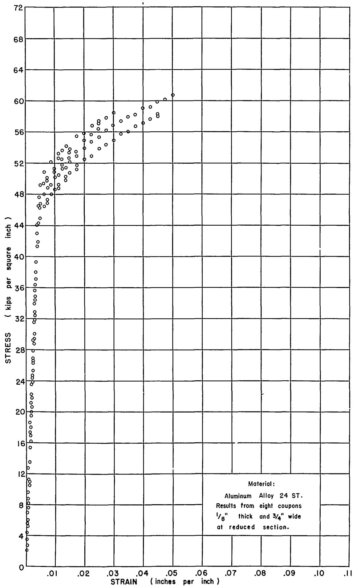
FIG. 3 — TENSION TEST RESULTS
