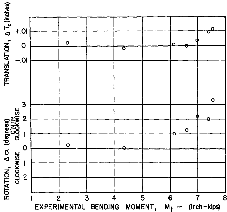
(a) ANGLE BEAM M-2, \theta = 30^\circ
