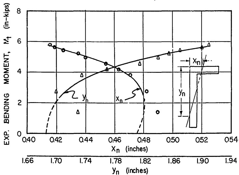
(b) ANGLE BEAM M-5, \theta = 60^\circ
