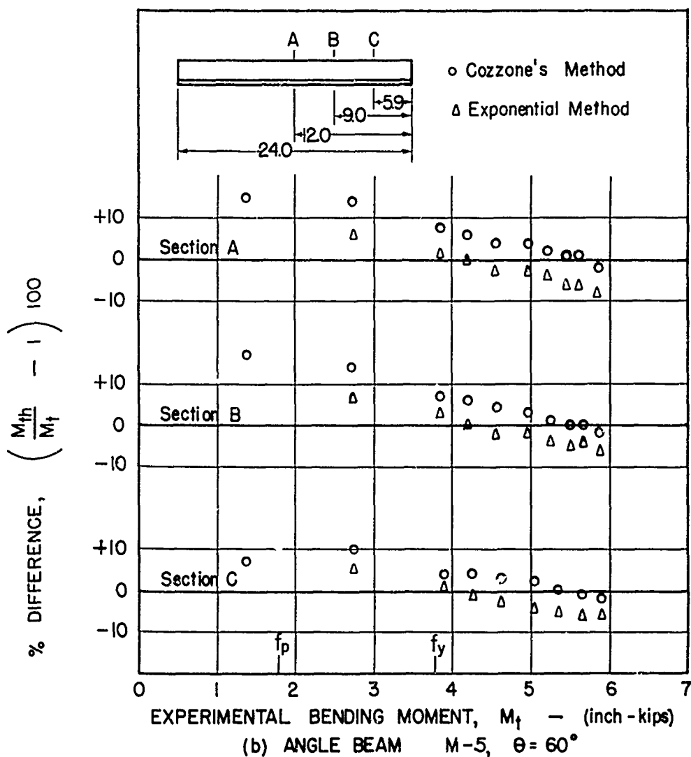
FIG. 12 - % DIFFERENCE BETWEEN EXPERIMENTAL AND COMPUTED BENDING MOMENTS FOR ANGLE BEAMS M-4 & M-5
