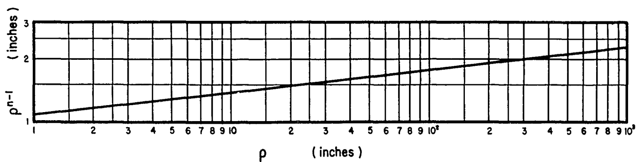
FIG. 21 — VALUES OF \rho AND c FOR USE IN THE EXPONENTIAL EQUATION
