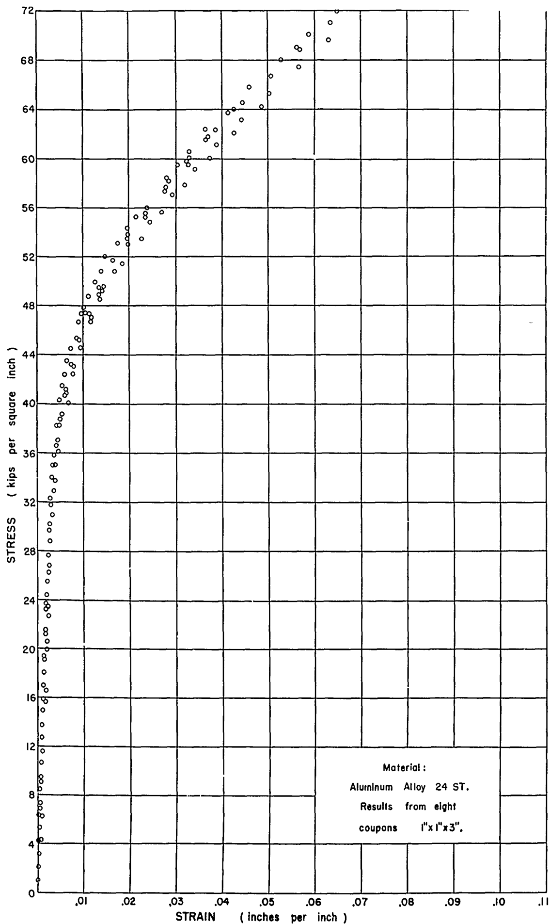
FIG. 4 — COMPRESSION TEST RESULTS
