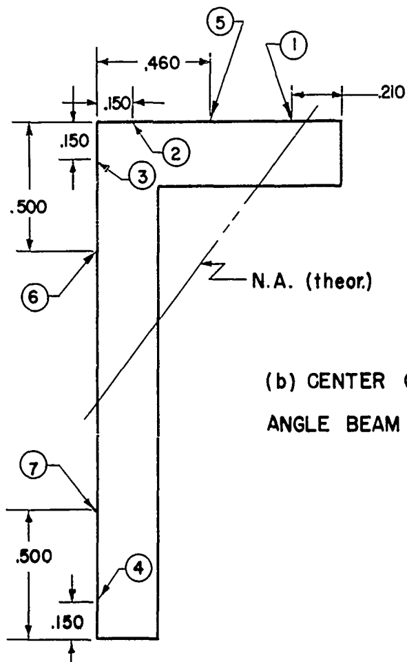
FIG. 8 — LOCATION OF ELECTRIC STRAIN GAGES
