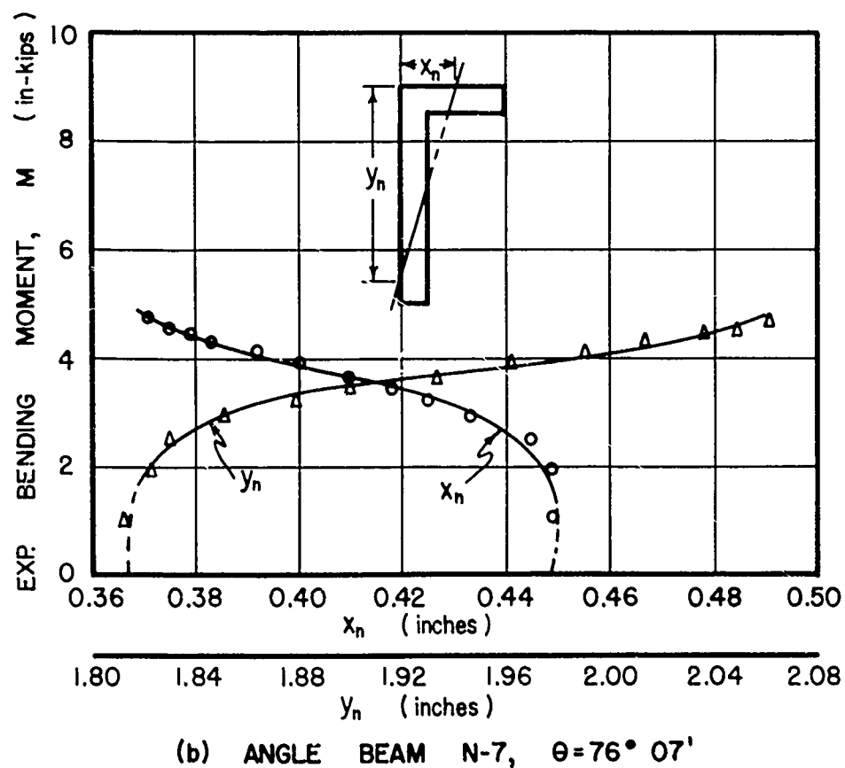
FIG. 19 — NEUTRAL AXIS LOCATION FOR ANGLE BEAMS N-6 AND N-7
