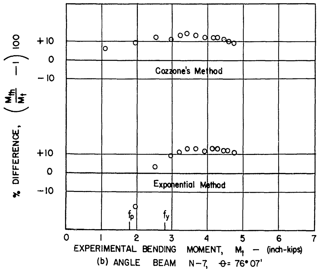
FIG. 13 - % DIFFERENCE BETWEEN EXPERIMENTAL AND COMPUTED BENDING MOMENTS FOR ANGLE BEAMS N-6 & N-7
