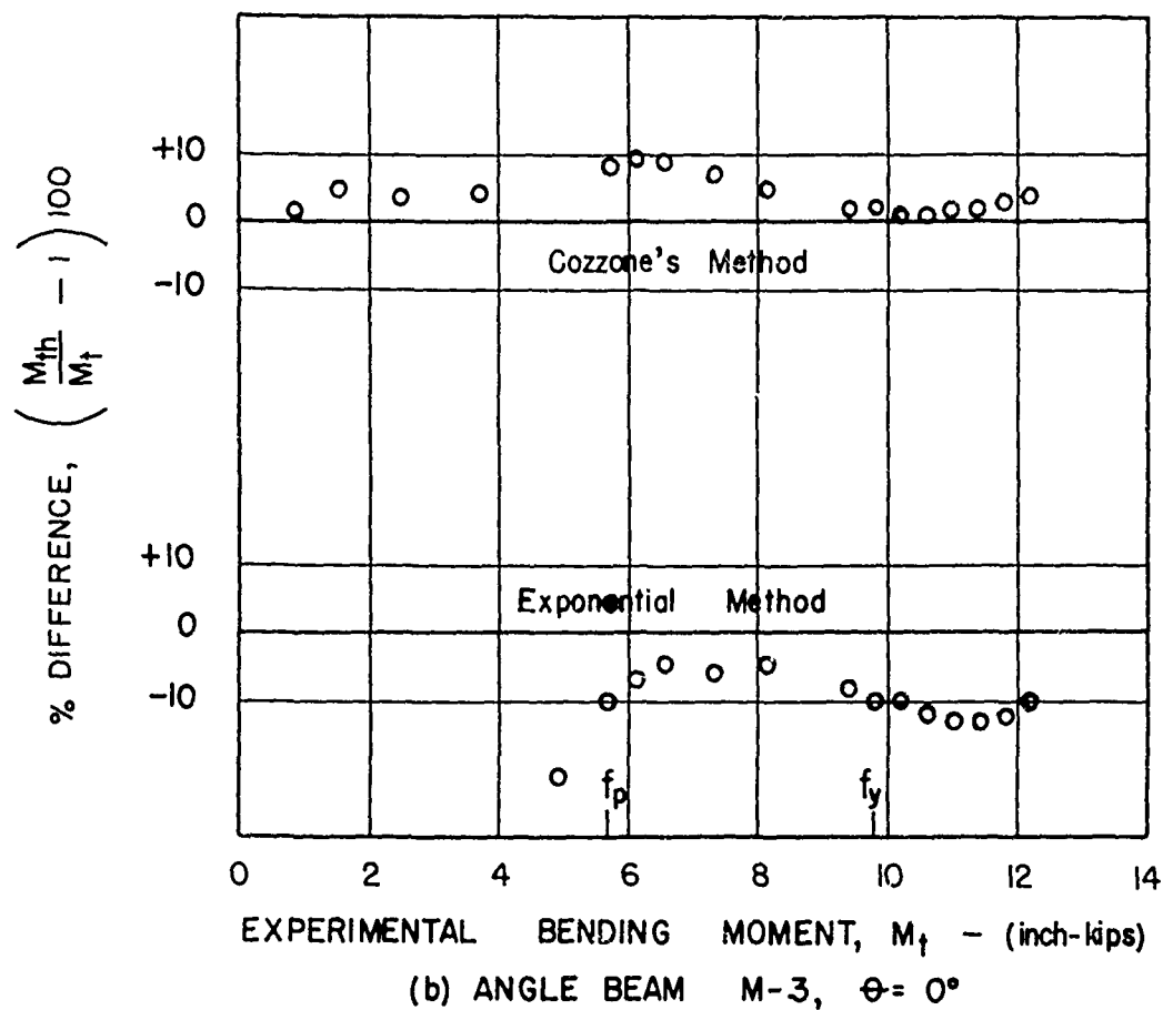
FIG. II -% DIFFERENCE BETWEEN EXPERIMENTAL AND COMPUTED BENDING MOMENTS FOR ANGLE BEAMS M-2 & M-3
