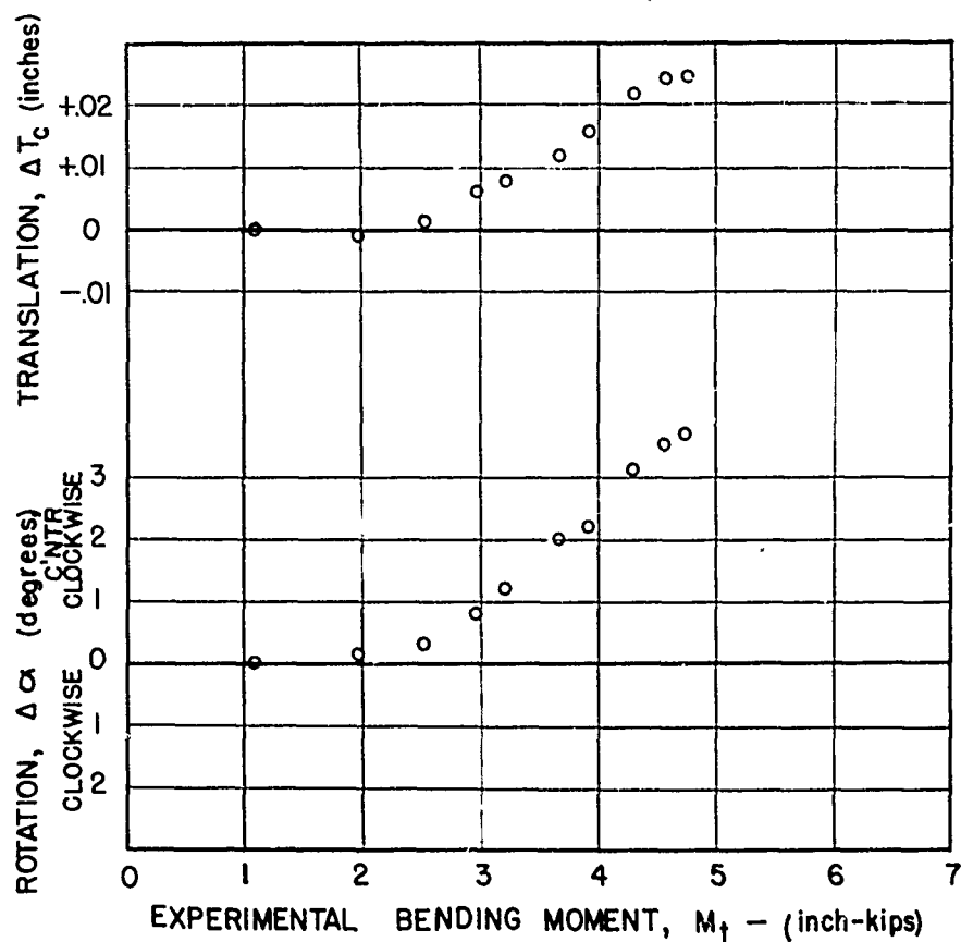
(b) ANGLE BEAM N-7, \theta = 76^\circ 07'
