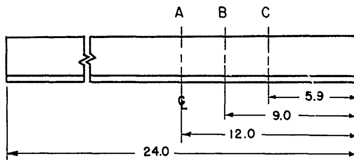
(a) LAYOUT, ANGLE BEAM M-5, \theta = 60^\circ
