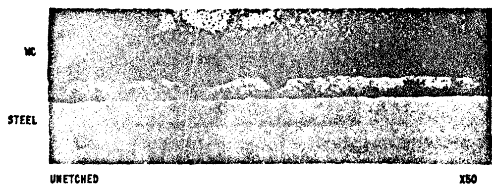
PHOTOMICROGRAPHS OF BRAZED JOINTS
