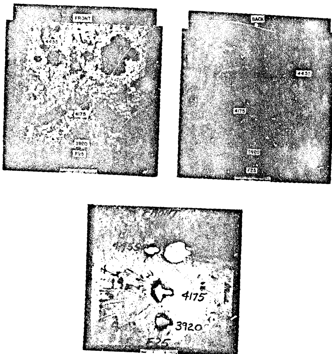
HADFIELD-MANGANESE SHEET TUNGSTEN CARBIDE COMPOSITE ARMOR PLATE ATTACKED BY CALIBER 0.40 M19B WC CORES AT 60° OBLIQUITY
