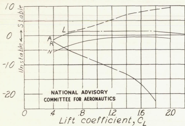
(b) \delta_f = 37^\circ .
