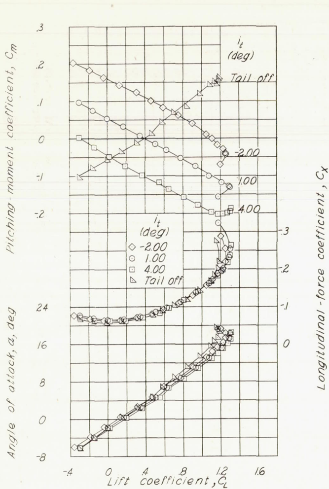
(a) \delta_f = 0^\circ ; windmilling propeller.
