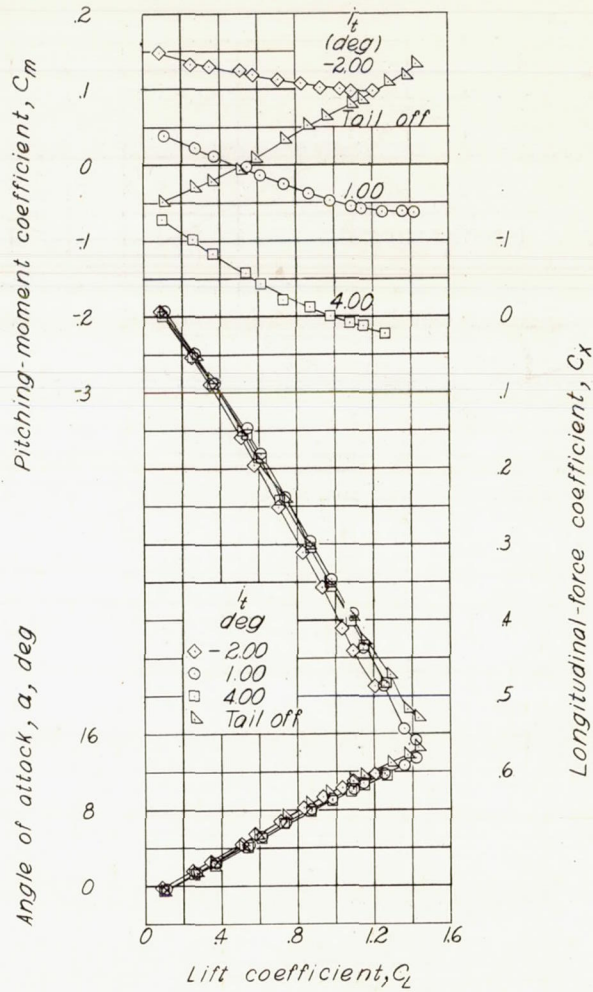
(b) \delta_f = 0^\circ ; power on.
