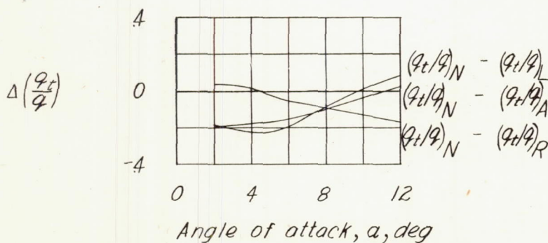
Figure 18.- Comparison of values of change in dynamic-pressure ratio \Delta \left( \frac{q_t}{q} \right) due to horizontal-tail arrangements of the single-engine airplane model. \delta_f = 0^\circ ; q = 16.37 pounds per square foot; power on; N, normal tail; L, left semispan of normal tail; R, right semispan of normal tail; A, asymmetric tail.
