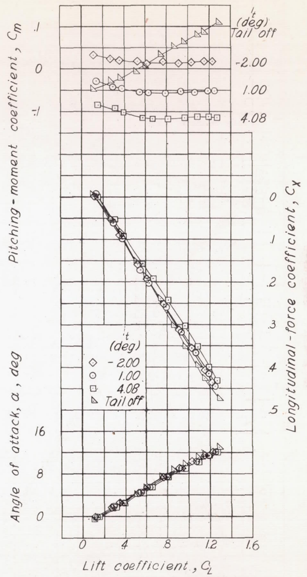
(b) \delta_F = 0^\circ ; power on.
