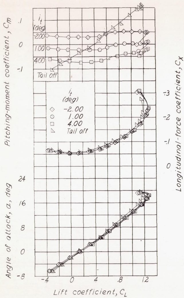
(a) \delta_F = 0^\circ ; windmilling propeller.
