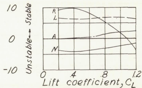
(b) Power on.
