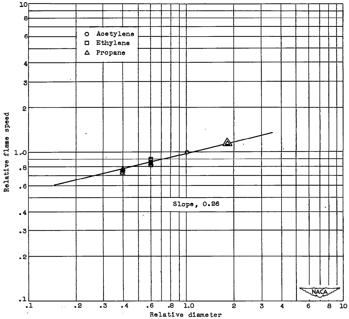
Figure 9. - Variation of relative flame speed with relative burner diameter, based on 5/8-inch burner.
