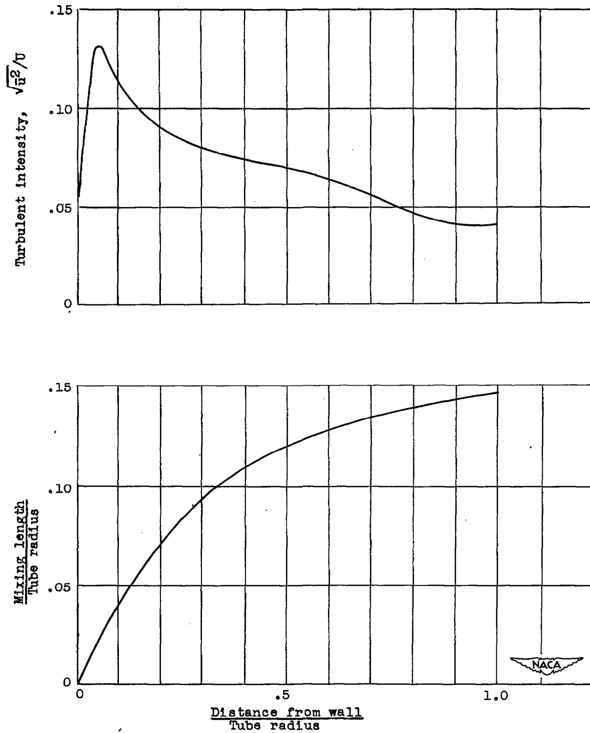
Figure 8. - Representative distribution across tube of turbulent intensity \sqrt{u^2}/U (reference 9) and mixing length l (reference 6).
