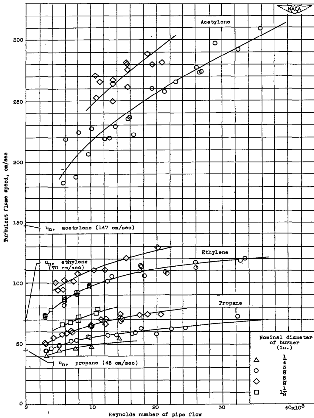
Figure 7. - Variation of flame speed with Reynolds number of flow. (Normal flame speed u_n from reference 4.)
