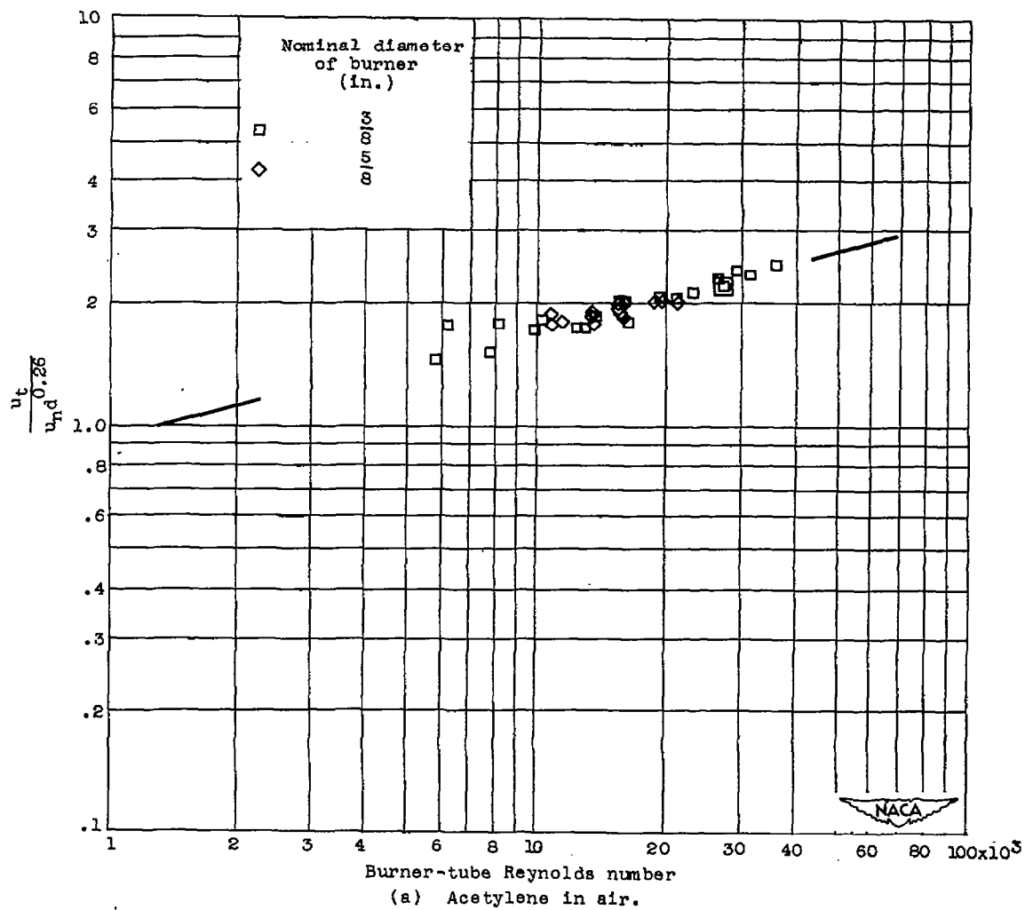
Figure 10. - \frac{u_t}{u_n d^{0.25}} as a function of burner-tube Reynolds number. Turbulent flame speed u_t , centimeters per second; normal flame speed u_n , centimeters per second; diameter d , centimeters.
