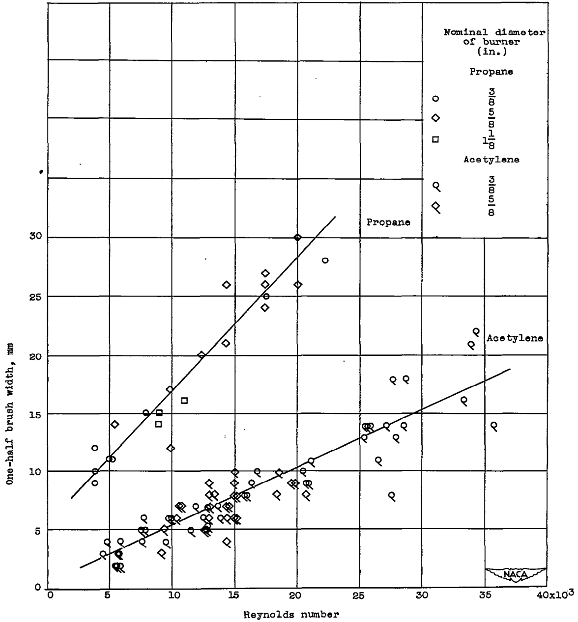
Figure 5. - Variation of flame-brush width with Reynolds number.
