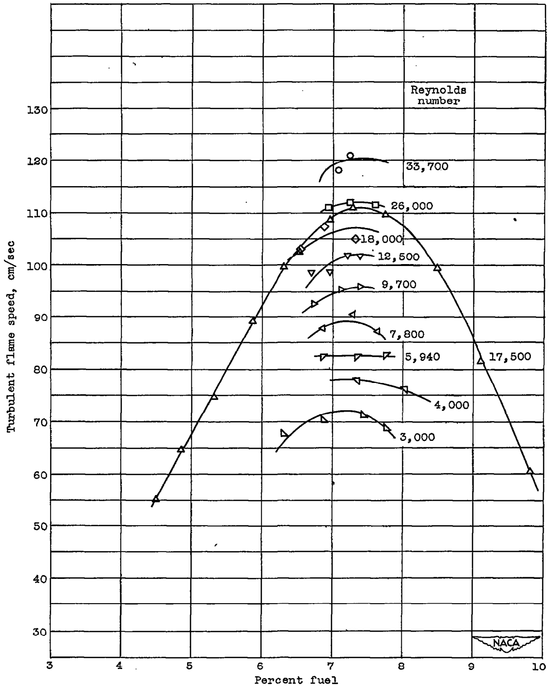
Figure 6. - Variation of flame speed with fuel concentration. Burner diameter, 3/8 inch; fuel, ethylene in air.
