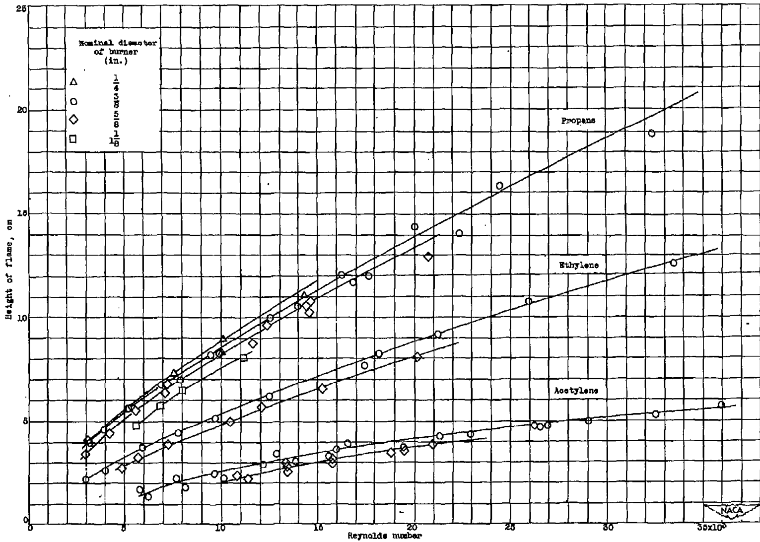
Figure 4. - Variation of mean flame height with Reynolds number.
