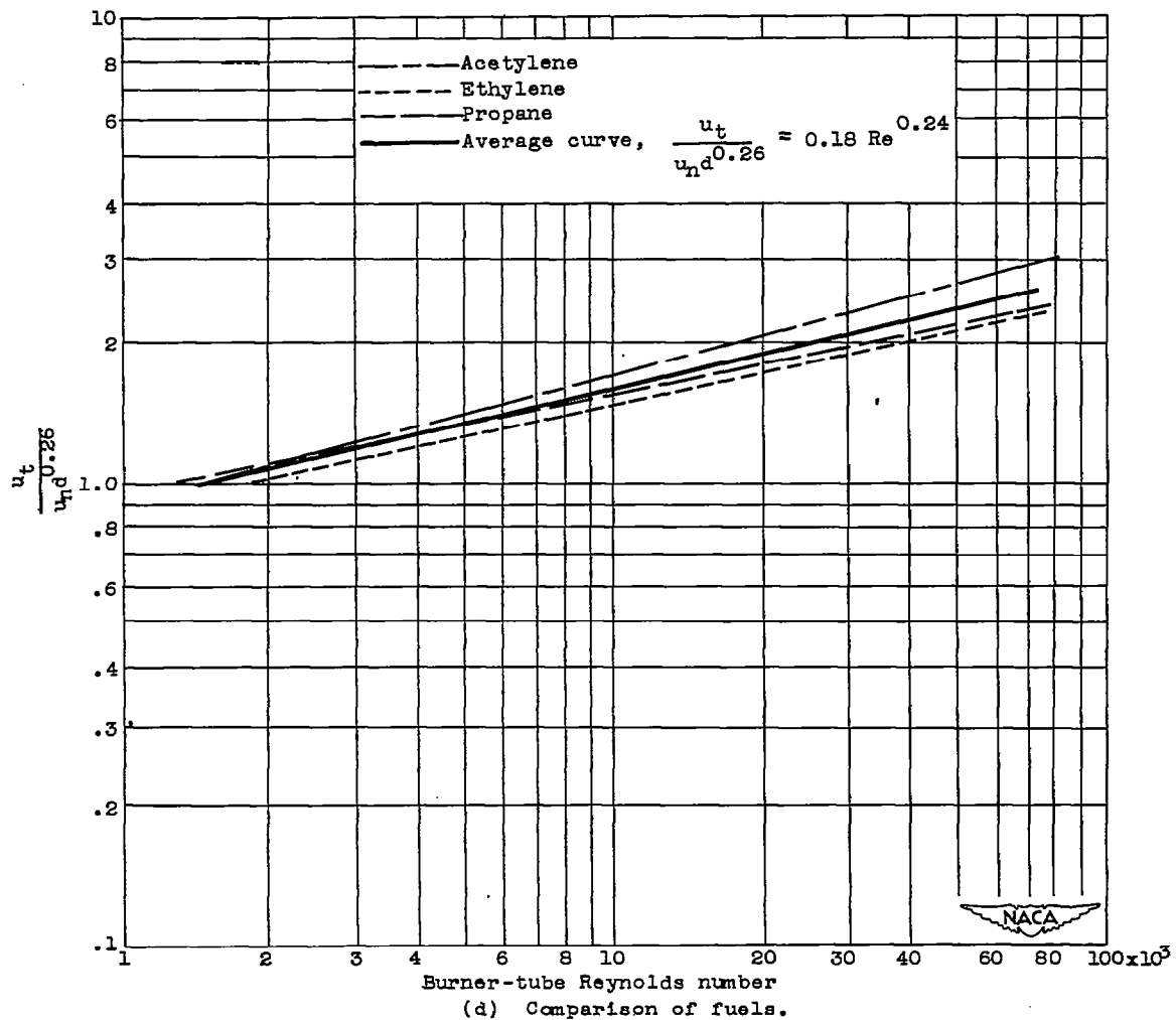
Figure 10. - Concluded. \frac{u_t}{u_n d^{0.26}} as a function of burner-tube Reynolds number.
