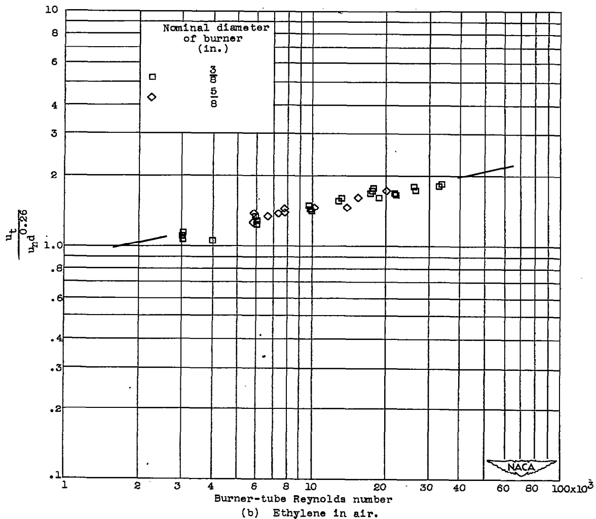
Figure 10. - Continued. \frac{u_t}{u_n d^{0.26}} as a function of burner-tube Reynolds number.
