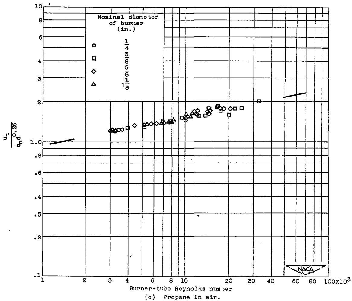
Figure 10. - Continued. \frac{u_t}{u_n d^{0.25}} as a function of burner-tube Reynolds number.
