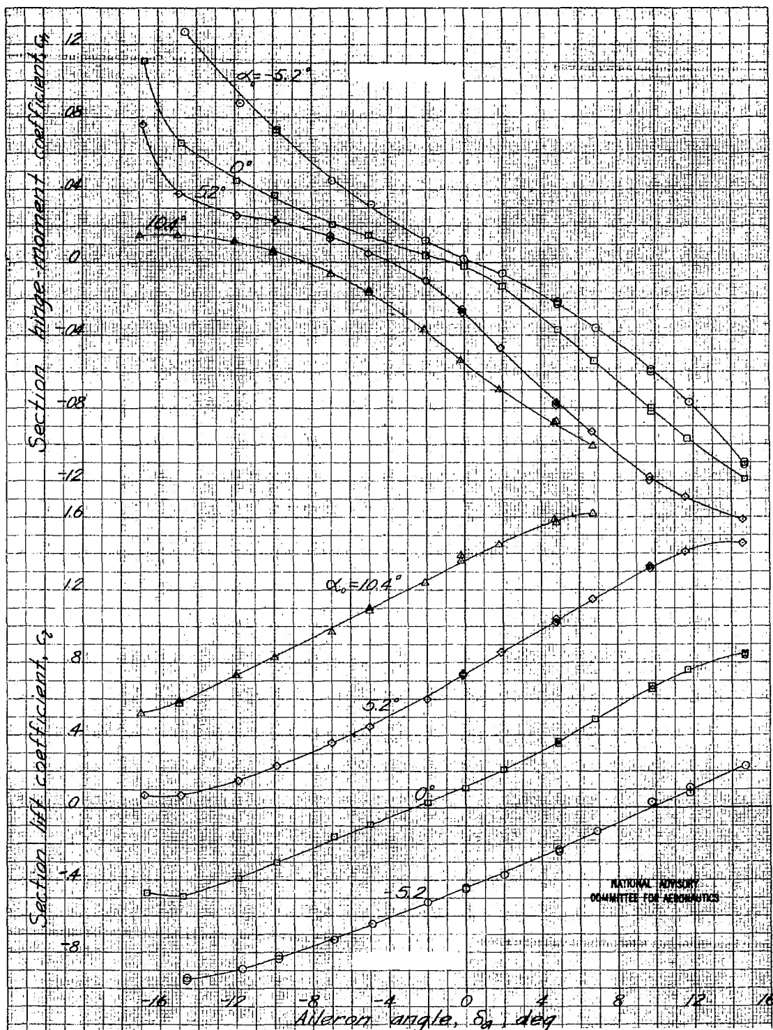
Figure 22. - Variation of section coefficients with aileron angle at various section angles of attack \alpha_s . Impact pressure q_0 of 240 pounds per square foot. Data from two-dimensional tests in the Langley Stability Tunnel.
