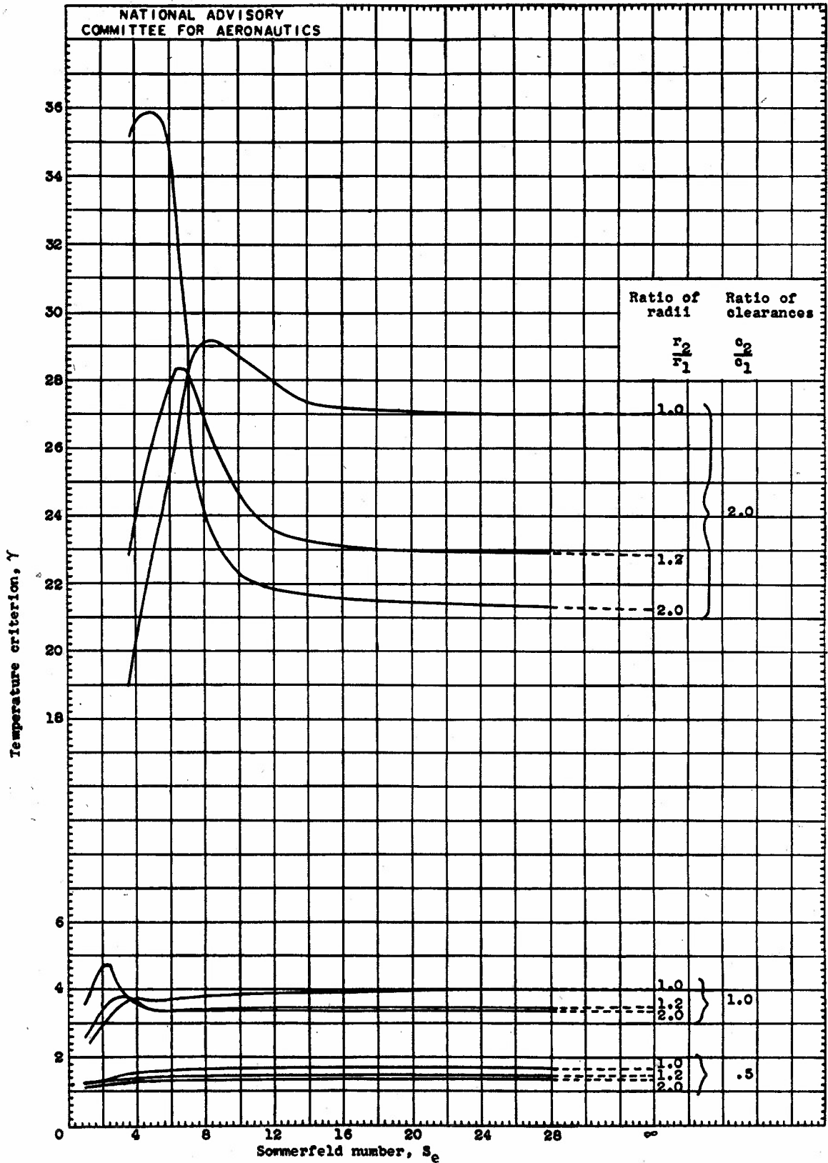
Figure 6. - Variation of temperature criterion with Sommerfeld number.
