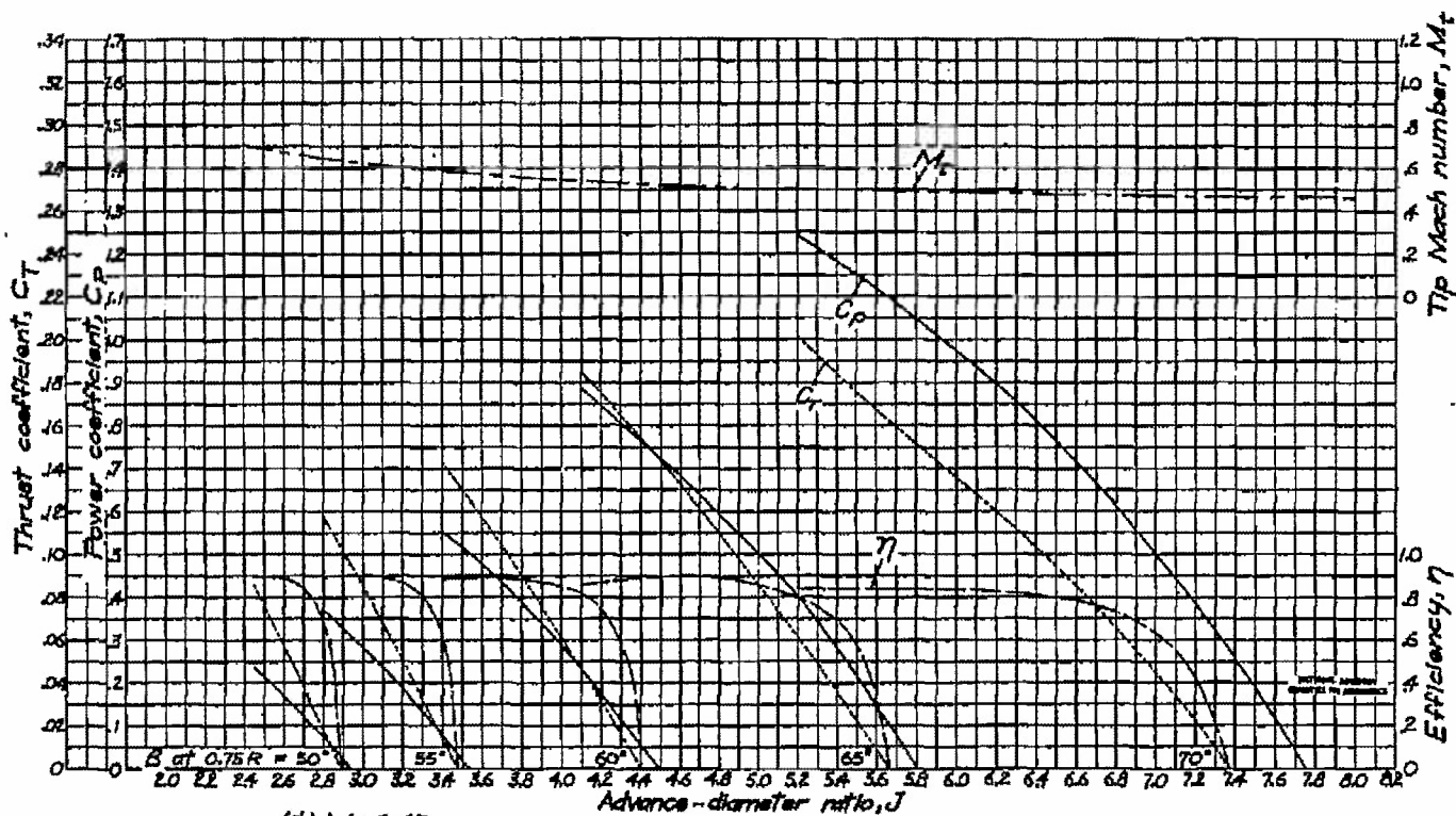
Figure 5-Continued. characteristics for the NACA 4306A-09 propeller.
