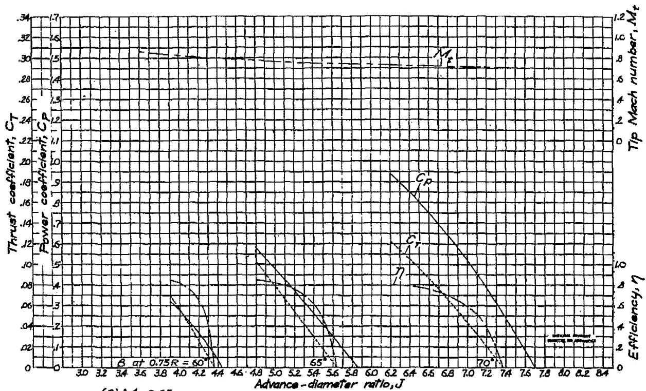
Figure 5-Continued. Characteristics for the NACA 4-3(06A)-09 propeller.
