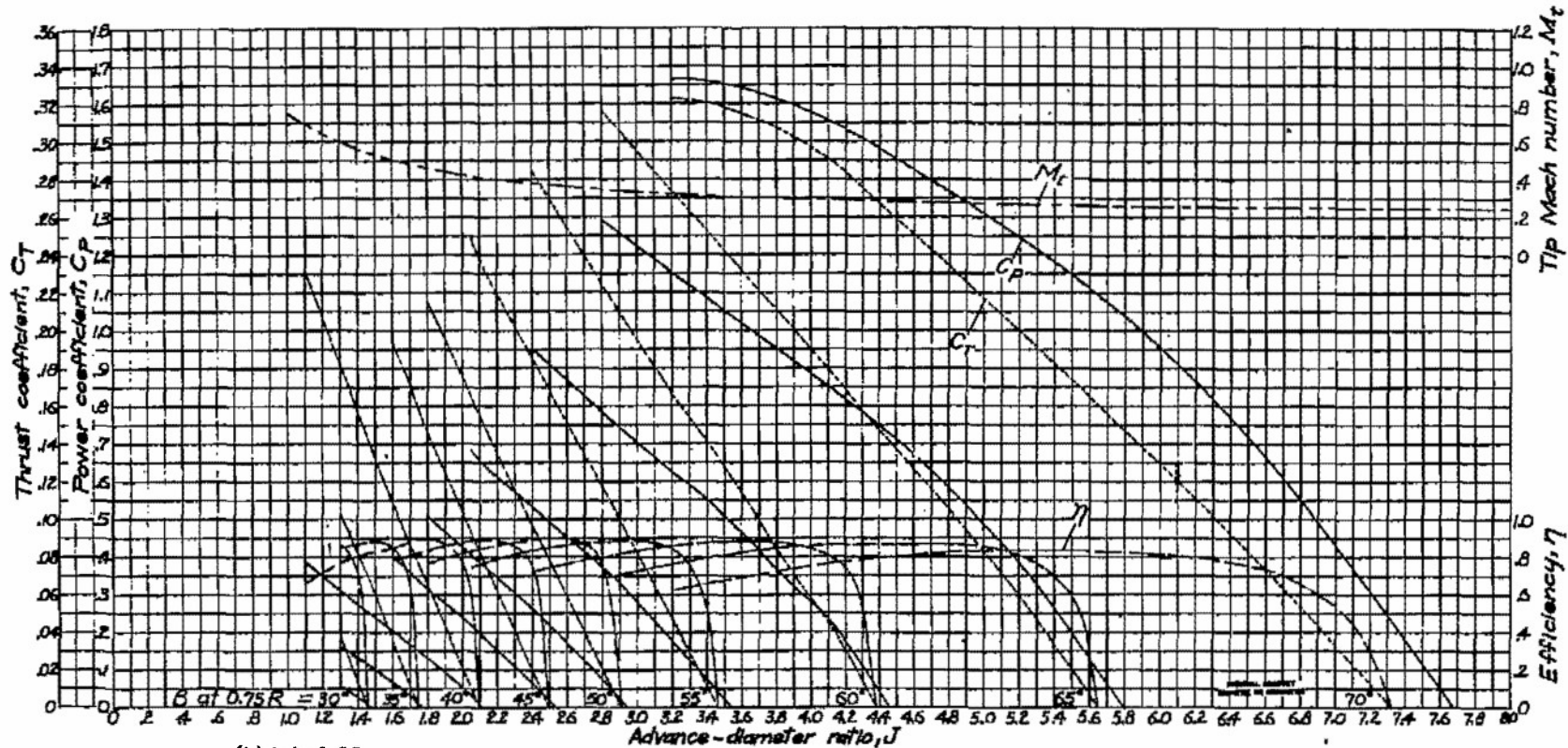
Figure 5.-Continued. Characteristics for the NACA 4(106A)-09 propeller.
