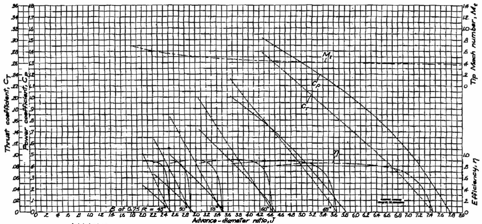
Figure 5.-Continued. Characteristics for the NACA 4(206A)-09 propeller.
