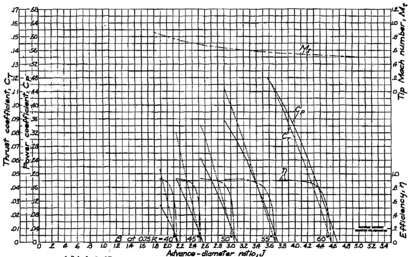
(d) M=0.43 . Figure 4.-Continued. Characteristics for the NACA 4-3(06.3)-06 propeller.
