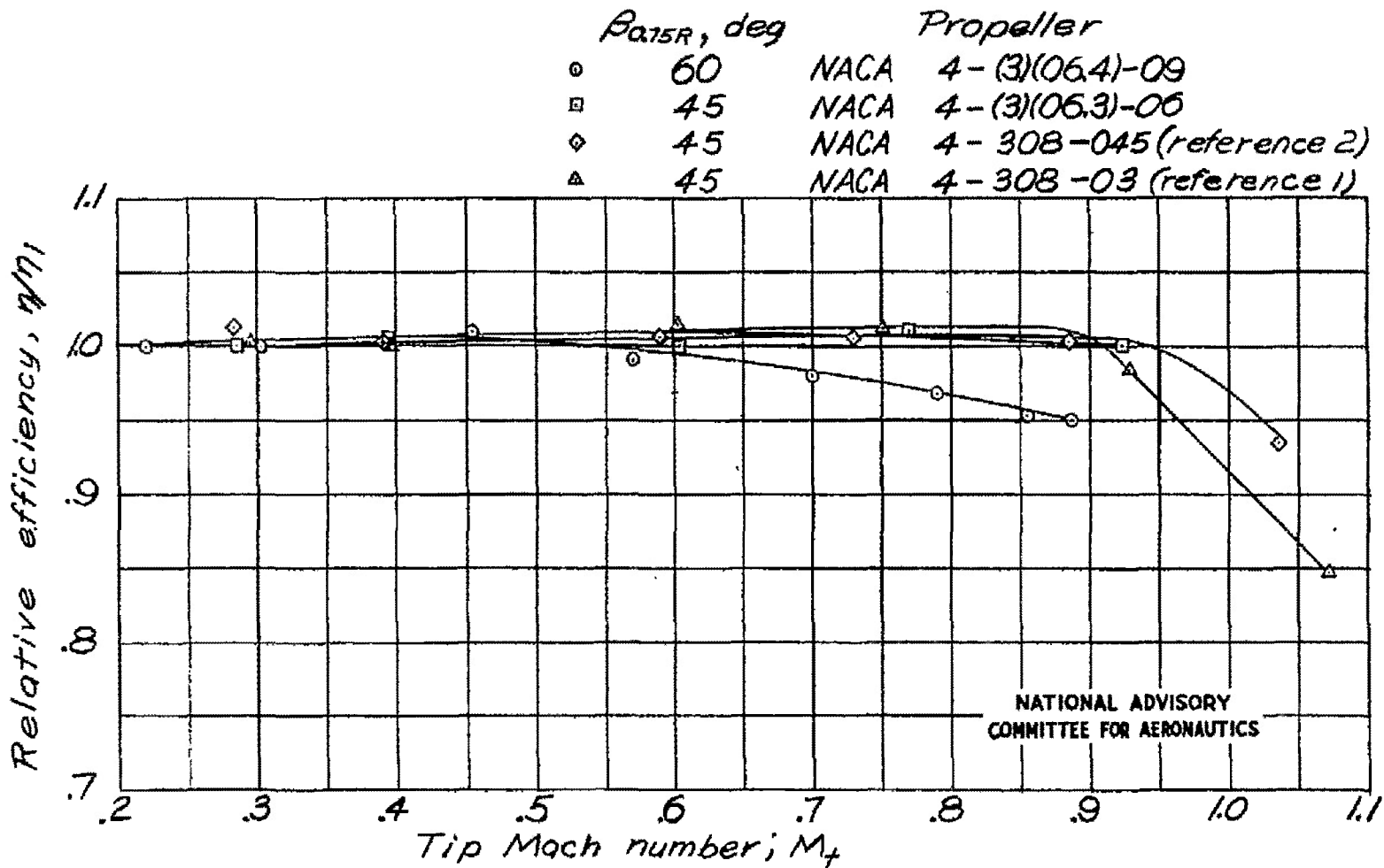
(a) Variation of \eta/\eta_1 with M_t
