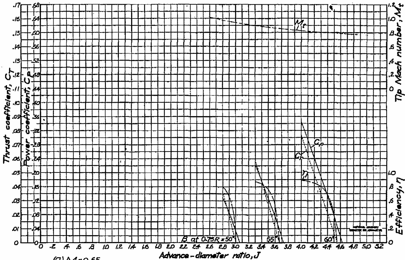
(9) M=0.65 . Figure 4.-Continued. Characteristics for the NACA 4(3)063-06 propeller.
