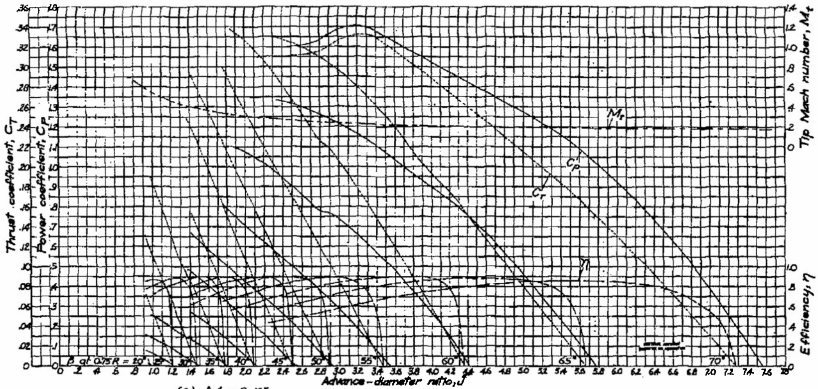
Figure 5.- Characteristics for the NACA 4(06A)-09 propeller.
