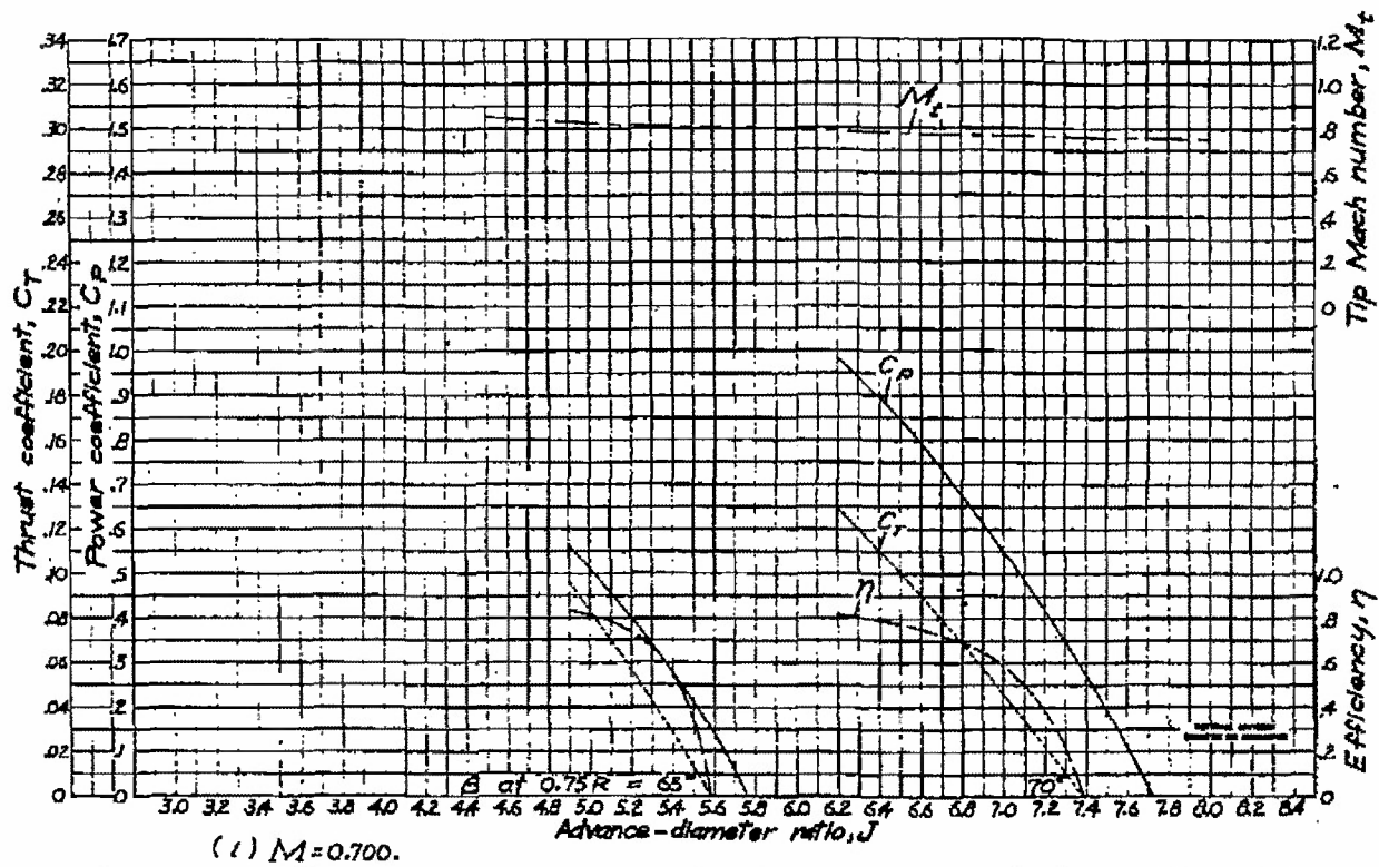
Figure 5-Continued. Characteristics for the NACA 4(06A)09 propeller.
