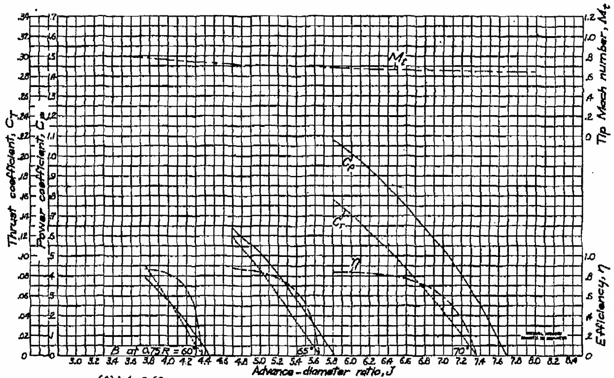
(f) M=0.60 . Figure 5-Continued. Characteristics for the NACA 40106A-09 propeller.
