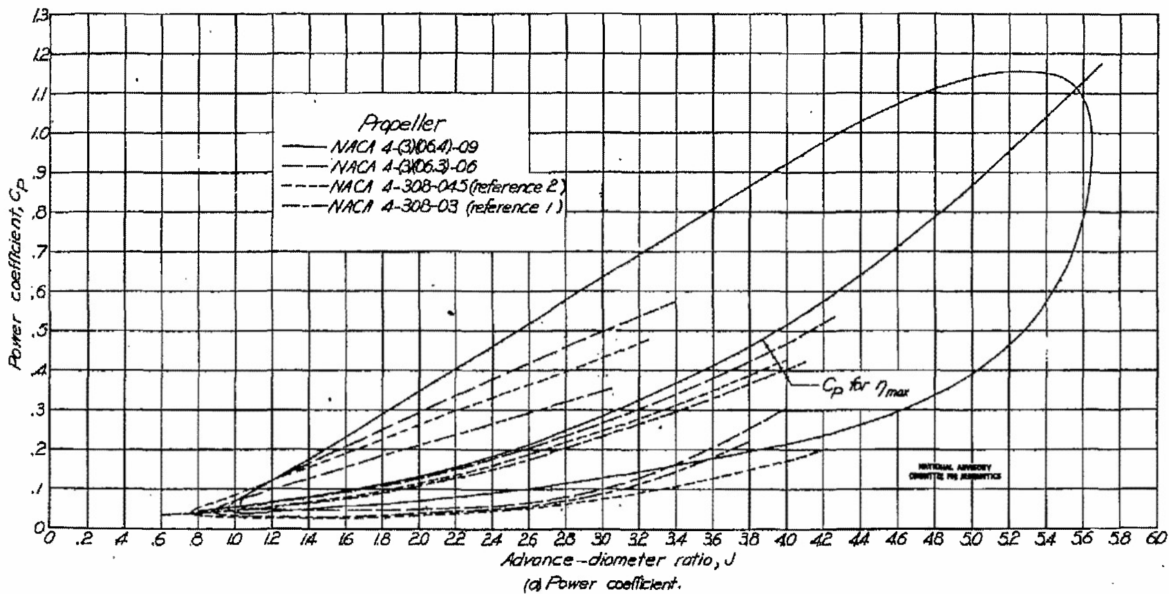
Figure 8.- Range of power coefficient and power coefficient-solidity ratio for efficiencies above 86 percent. M=0.165 .
