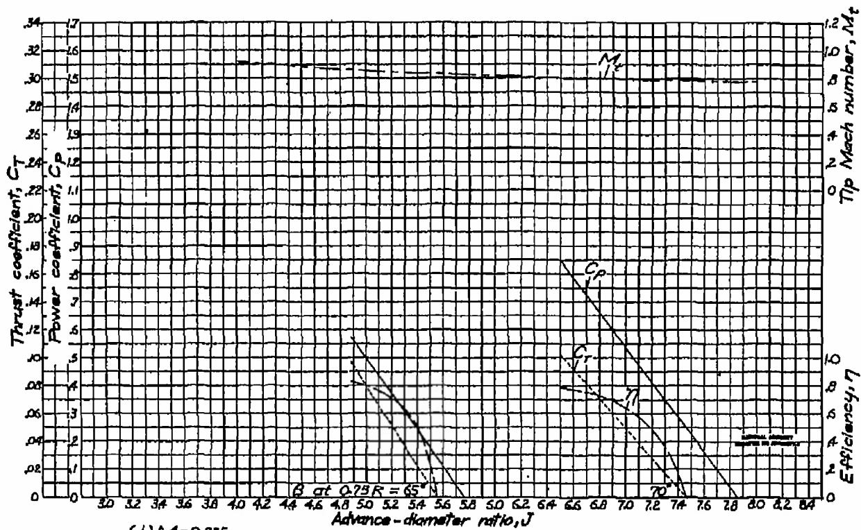
(J) M = 0.725 . Figure 5.-concluded. Characteristics for the NACA 4(3)(064)-09 propeller.
