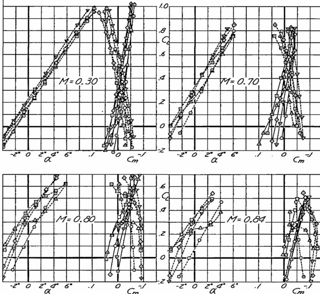
FIGURE 5.- EFFECT OF DIVE-RECOVERY FLAPS ON THE LIFT-MOMENT CHARACTERISTICS OF THE LOCKHEED YP-80A AIRPLANE MODEL.
