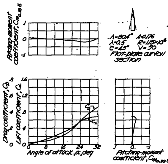
Figure 37.- Longitudinal stability characteristics of a 80° swept-back wing. Data from the Langley free-flight tunnel.
