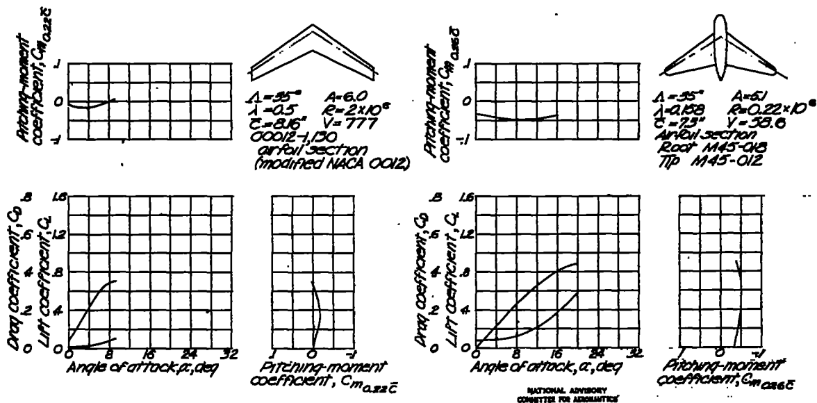
Figure 11.- Longitudinal stability characteristics of a 35° swept-back wing. Data from reference 5.
