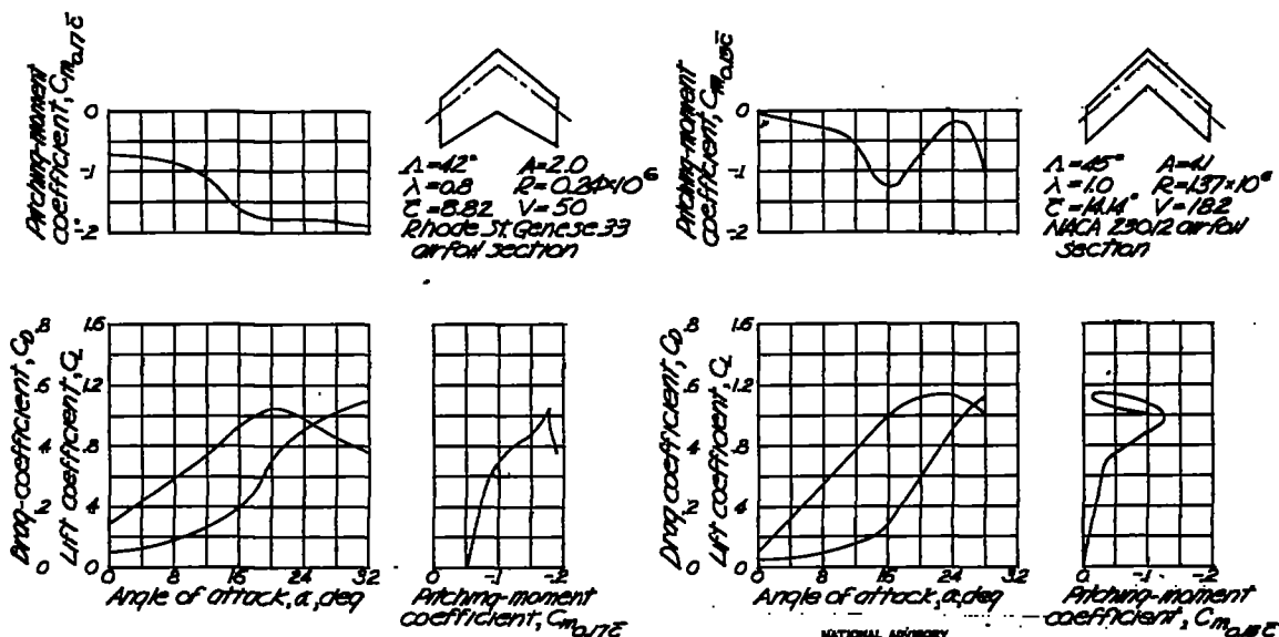
Figure 19.- Longitudinal stability characteristics of a 42° swept-back wing. Data from the Langley free-flight tunnel.
