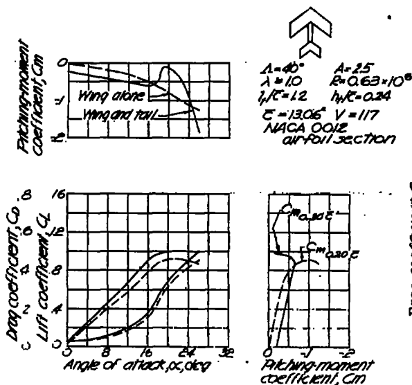
Figure 44.-Longitudinal stability characteristics of a 40° swept-back wing and horizontal tail combination. Data from the Langley 7 by 10 foot tunnel.
