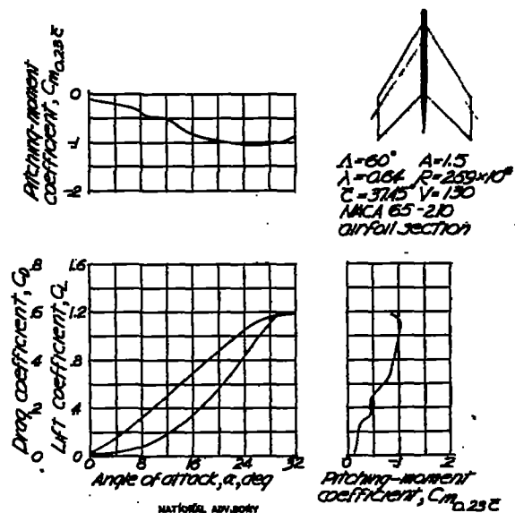
Figure 28.-Longitudinal stability characteristics of a 60° swept-back wing. Data from the Langley 300 MPH 7-by-10-foot tunnel.
