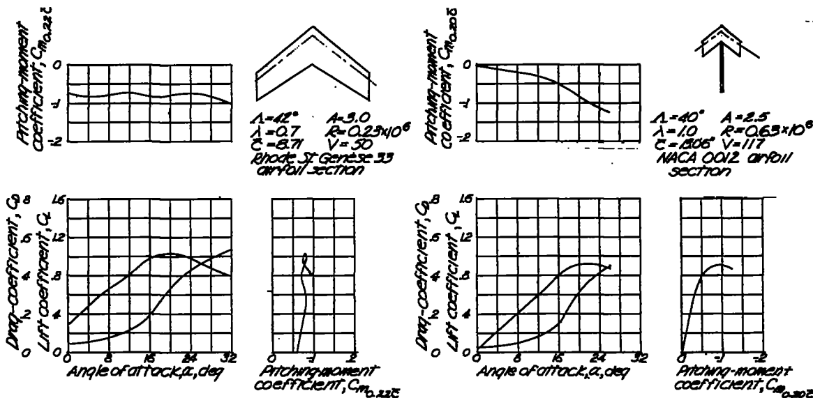
Figure 17.- Longitudinal stability characteristics of a 42° swept-back wing. Data from the Langley free-flight tunnel.
