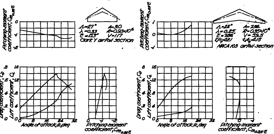
Figure 9.- Longitudinal stability characteristics of a 27° swept-back wing. Data from reference 3.
