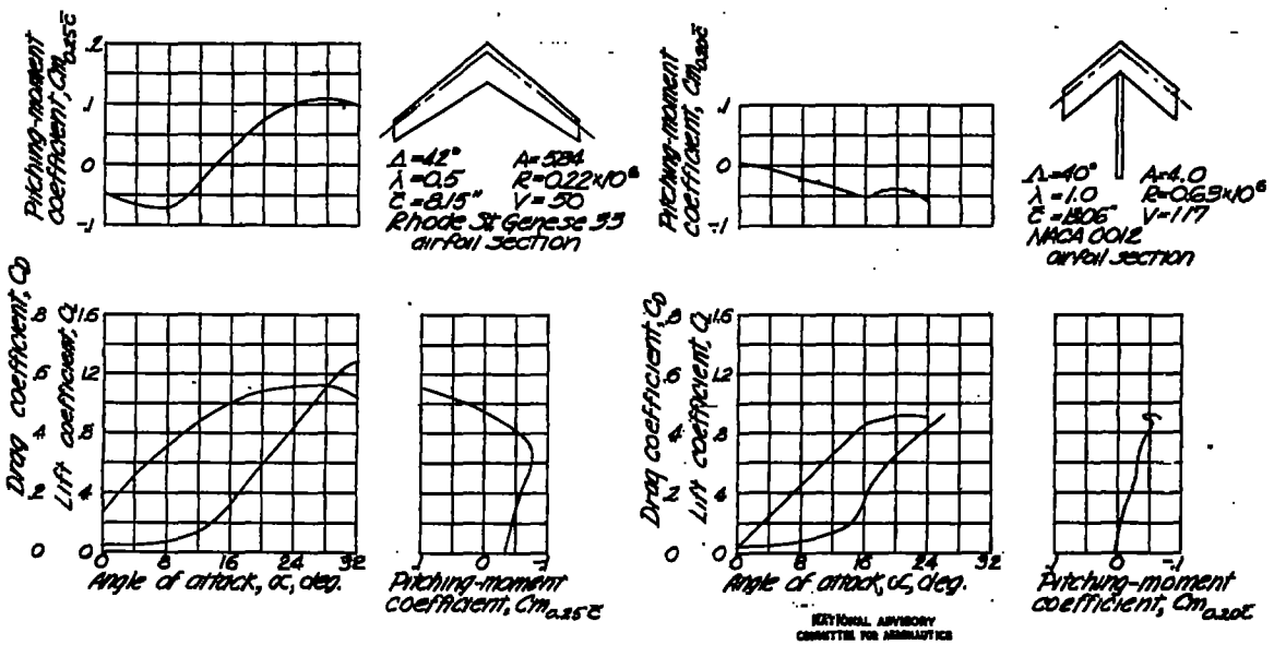
Figure 15.-Longitudinal stability characteristics of a 42° swept-back wing. Data from the Langley free-flight tunnel.
