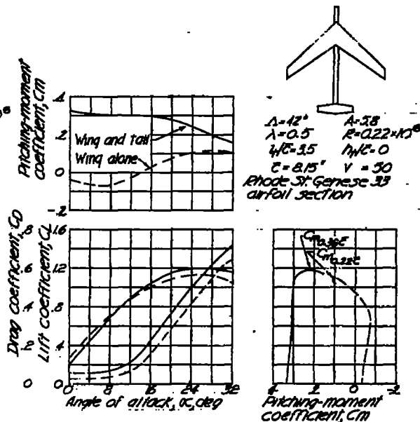
Figure 45.-Longitudinal stability characteristics of a 42° swept-back wing and horizontal tail combination. Data from the Langley free-flight tunnel.
