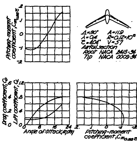
Figure 5.- Longitudinal stability characteristics of a 30° swept-back wing and fuselage combination. Data from Langley Free-flight tunnel.
