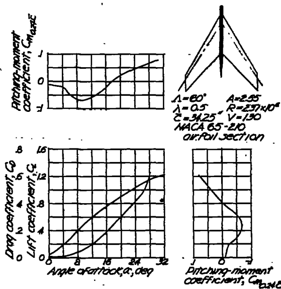
Figure 26.-Longitudinal stability characteristics of a 60° swept-back wing. Data from the Langley 300 MPH 7-by-10-foot tunnel.
