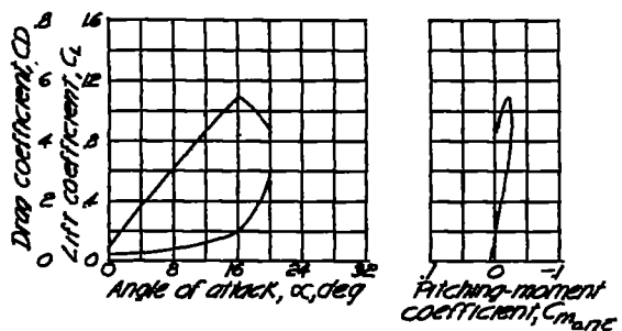
Figure 35.-Longitudinal stability characteristics of a 22.5° swept-back wing and fuselage combination. Data from the Langley full-scale tunnel.
