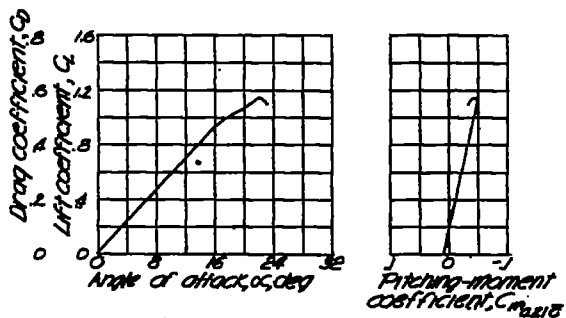
Figure 33.-Longitudinal stability characteristics of a 24° swept-back wing. Data from the Langley Full-scale Tunnel.
