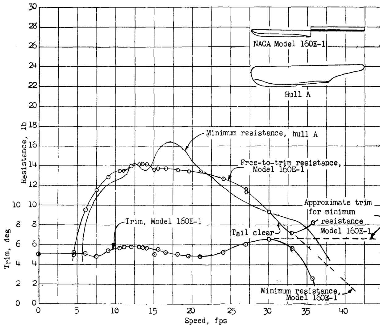
Figure 9.- Comparison of resistance of NACA Model 160E-1 with that of a conventional flying-boat hull.
