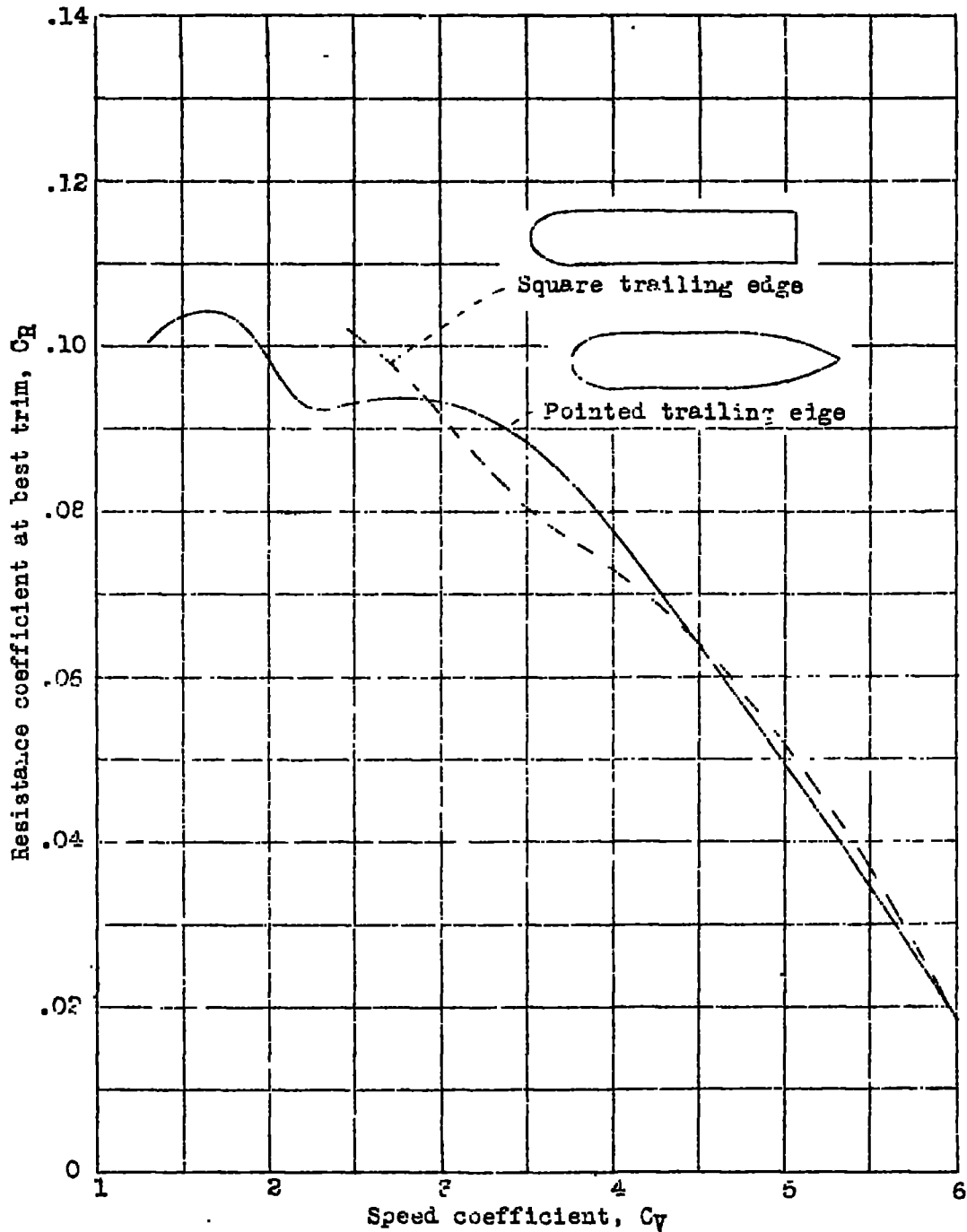
Figure 11.- Comparison of resistance coefficients of planing surfaces with square and pointed trailing edges. Angle of dead rise, 22\text{-}1/2 degrees.
