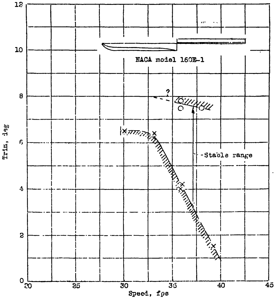
Figure 13.- Longitudinal stability limits of NACA model 16OE-1.
