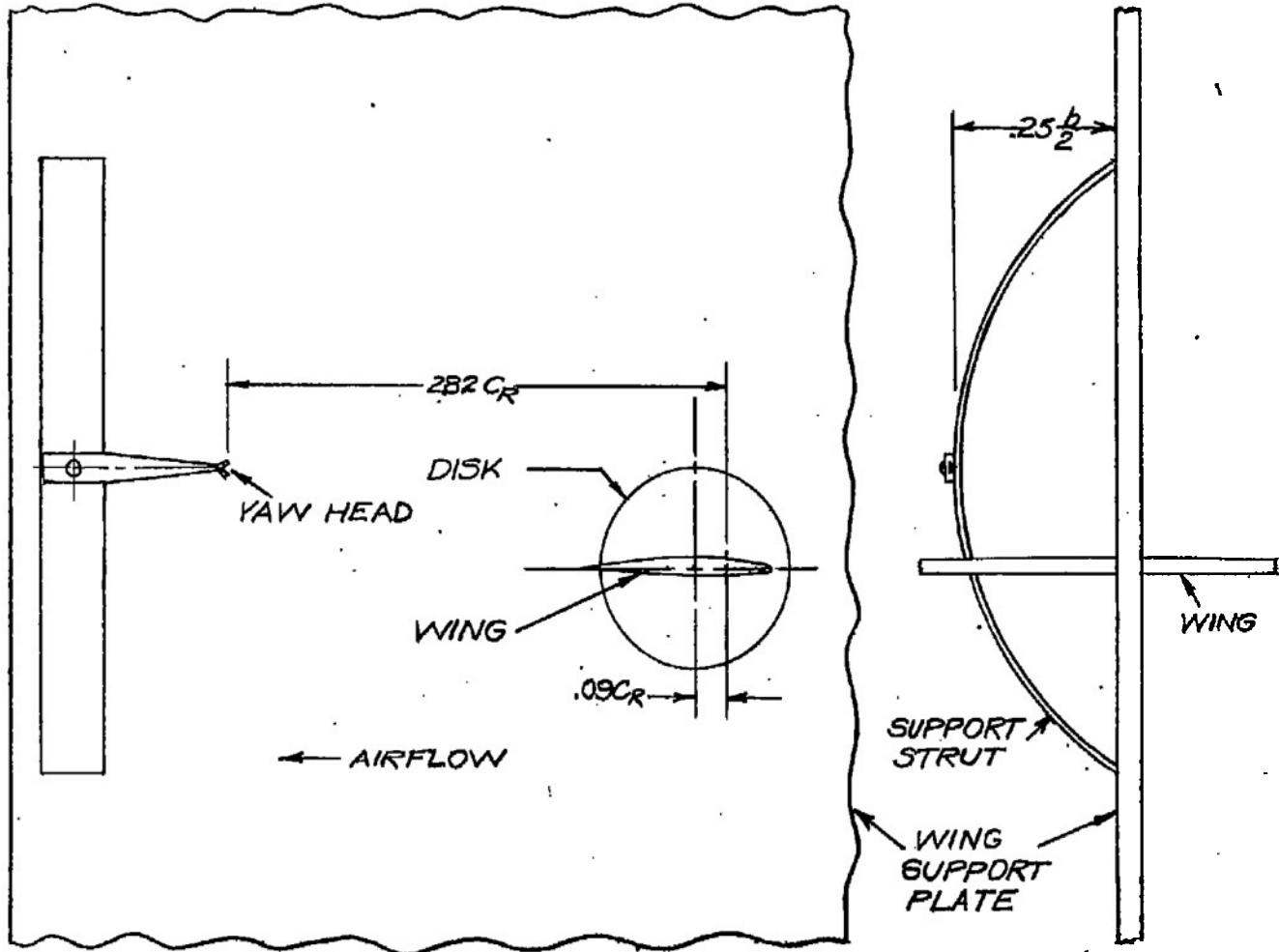
SIDE VIEW FIGURE 1.-TEST APPARATUS.
