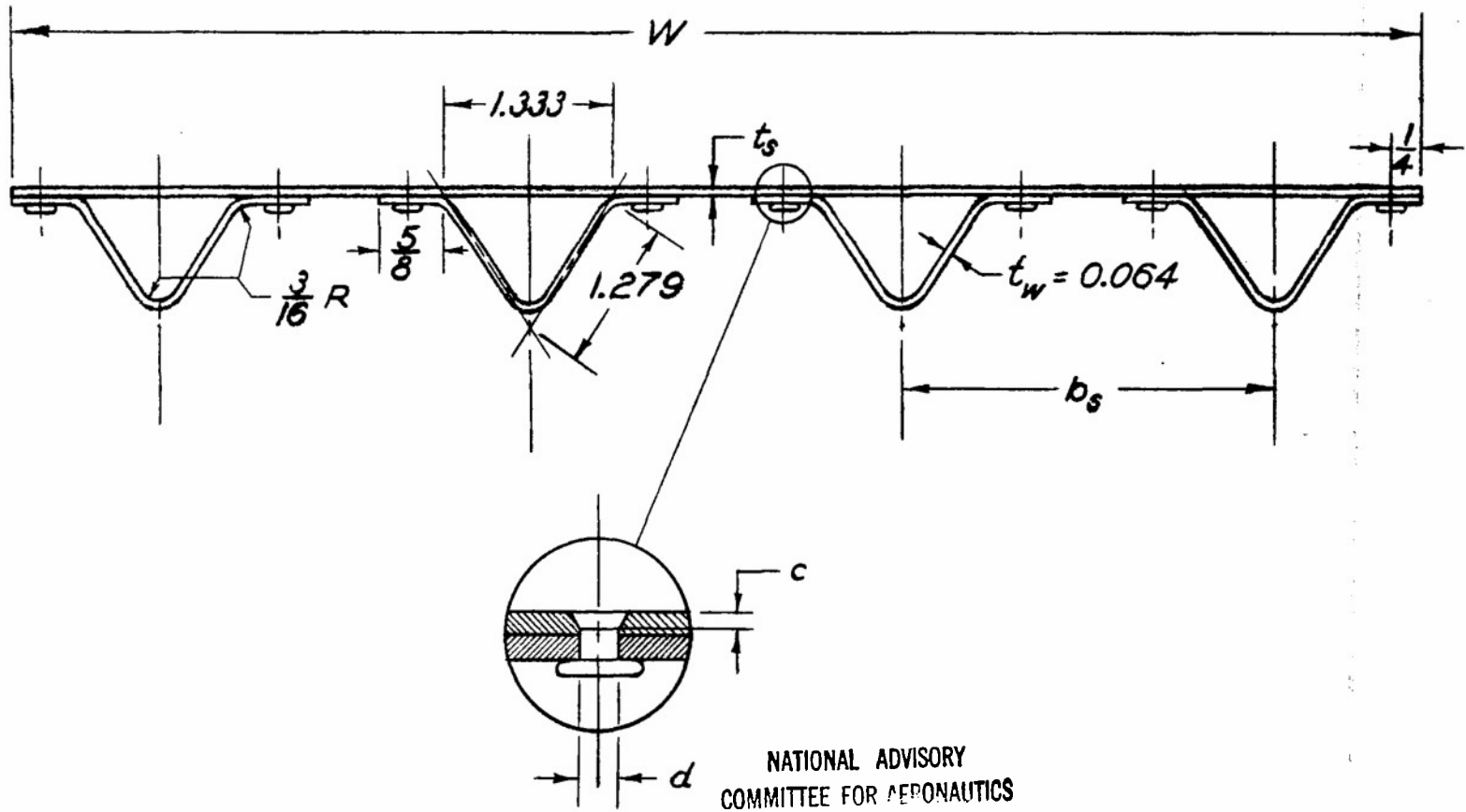
Figure 1. - Test specimens.
