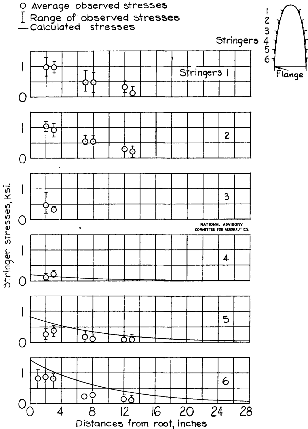
Figure 4 - Spanwise distribution of stringer stresses in D-section box, T=42.8 kip-inches.
