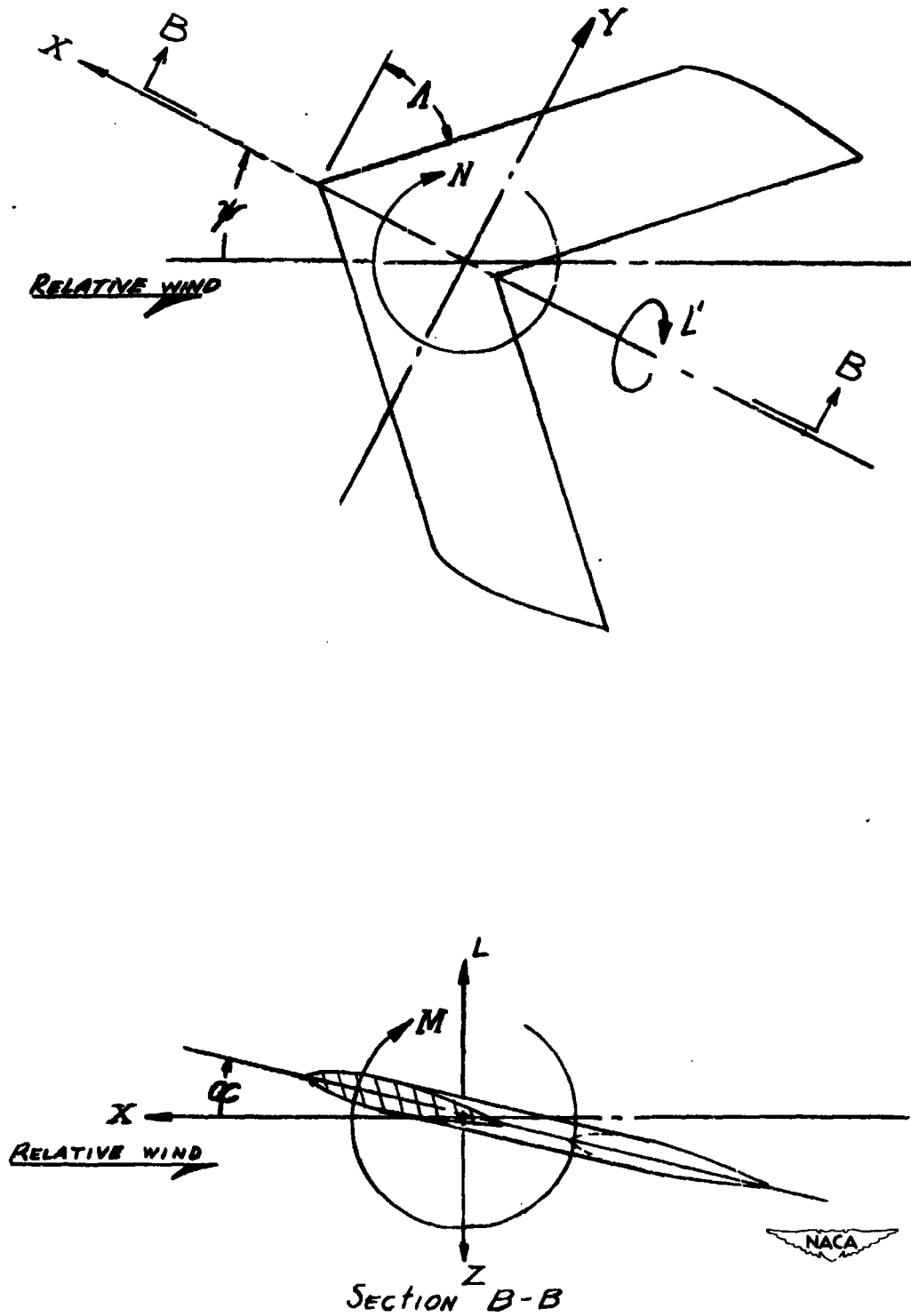
Figure 1.- System of axes used. Positive directions of forces, moments, and angles are indicated.
