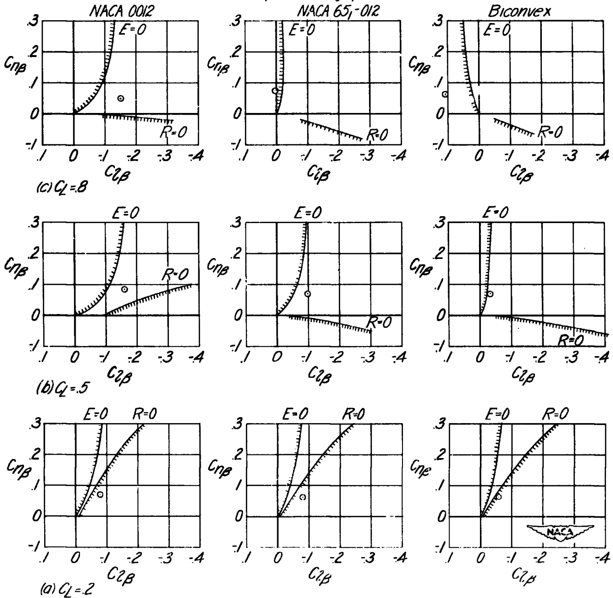
Figure 10.— Lateral stability boundaries for the three hypothetical transonic airplanes showing position of the airplanes with respect to the boundaries.
