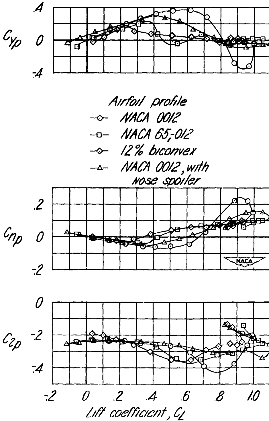
Figure 6.— Variations of C_{yp} , C_{np} , and C_{zp} with lift coefficient for the wings tested.
