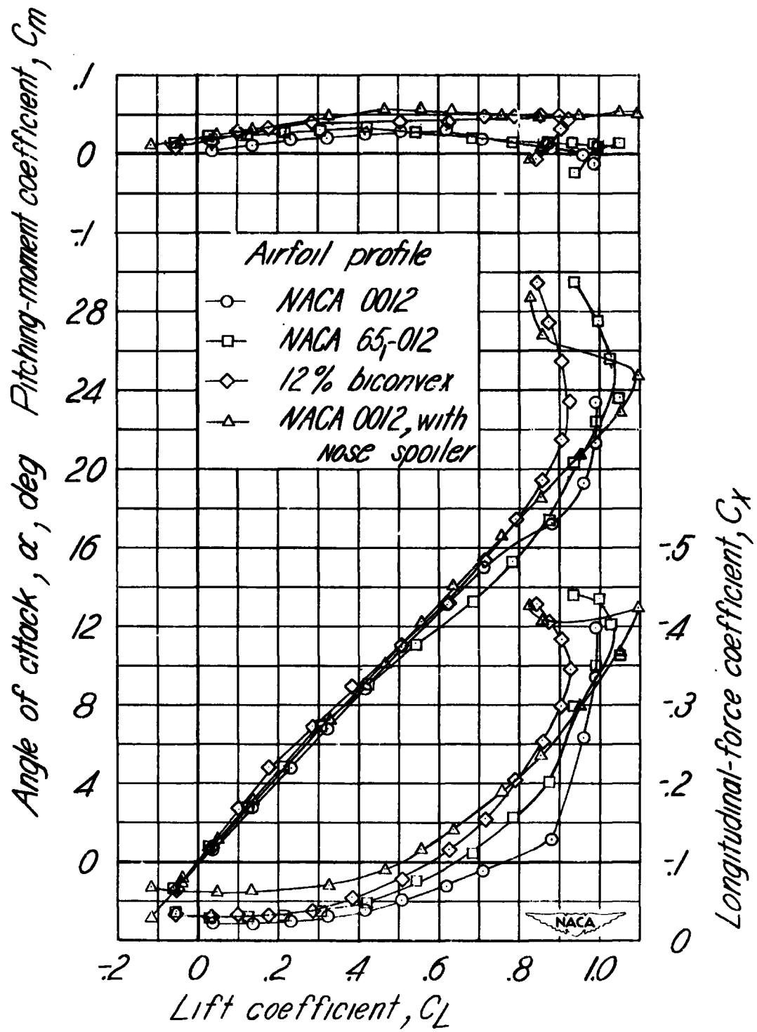
Figure 5.-- Variation of C_m , C_x , and \alpha with lift coefficient for the wings tested.
