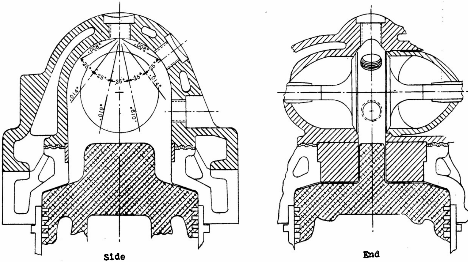
Figure 1.- Combustion chamber in the water-cooled cylinder.
