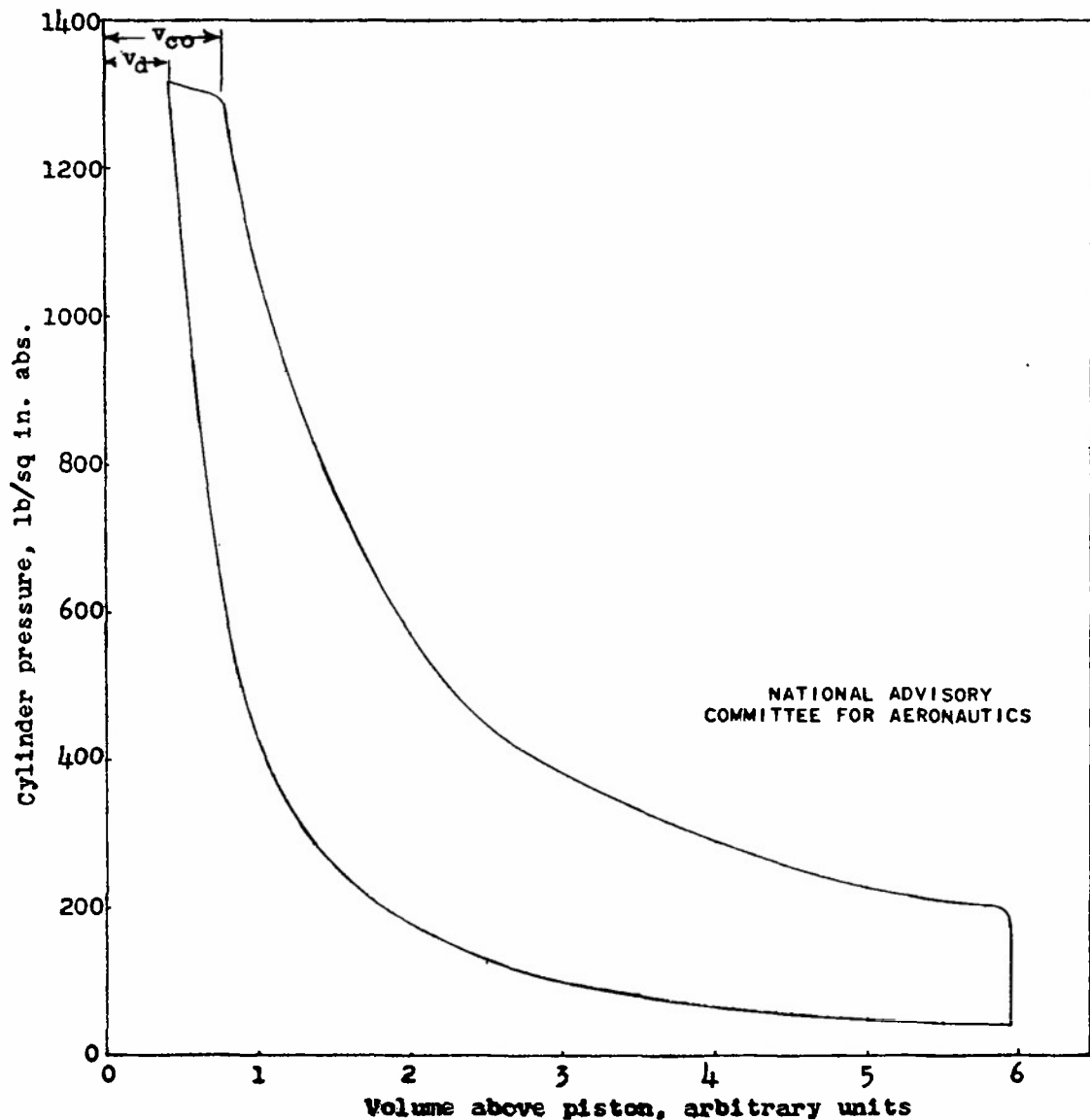
Figure 10. - High-pressure diagram obtained with Farnboro indicator and translated to pressure-volume card. Compression ratio, 13.1; engine speed, 2200 rpm; inlet-air pressure, 80 inches mercury absolute; inlet-air temperature, 95° F; measured indicated mean effective pressure, 335 pounds per square inch; area of card, 8.74 square inches; equivalent mean effective pressure, 318 pounds per square inch.
