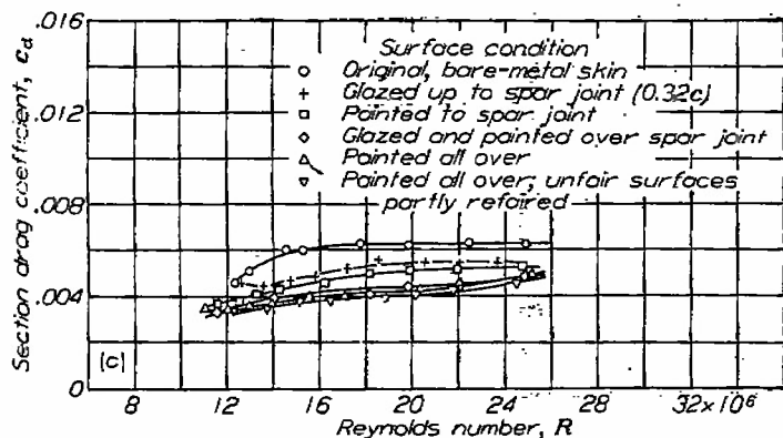
(c) Model 3, NACA 66(215)-116 airfoil section. c_l=0.18 .
