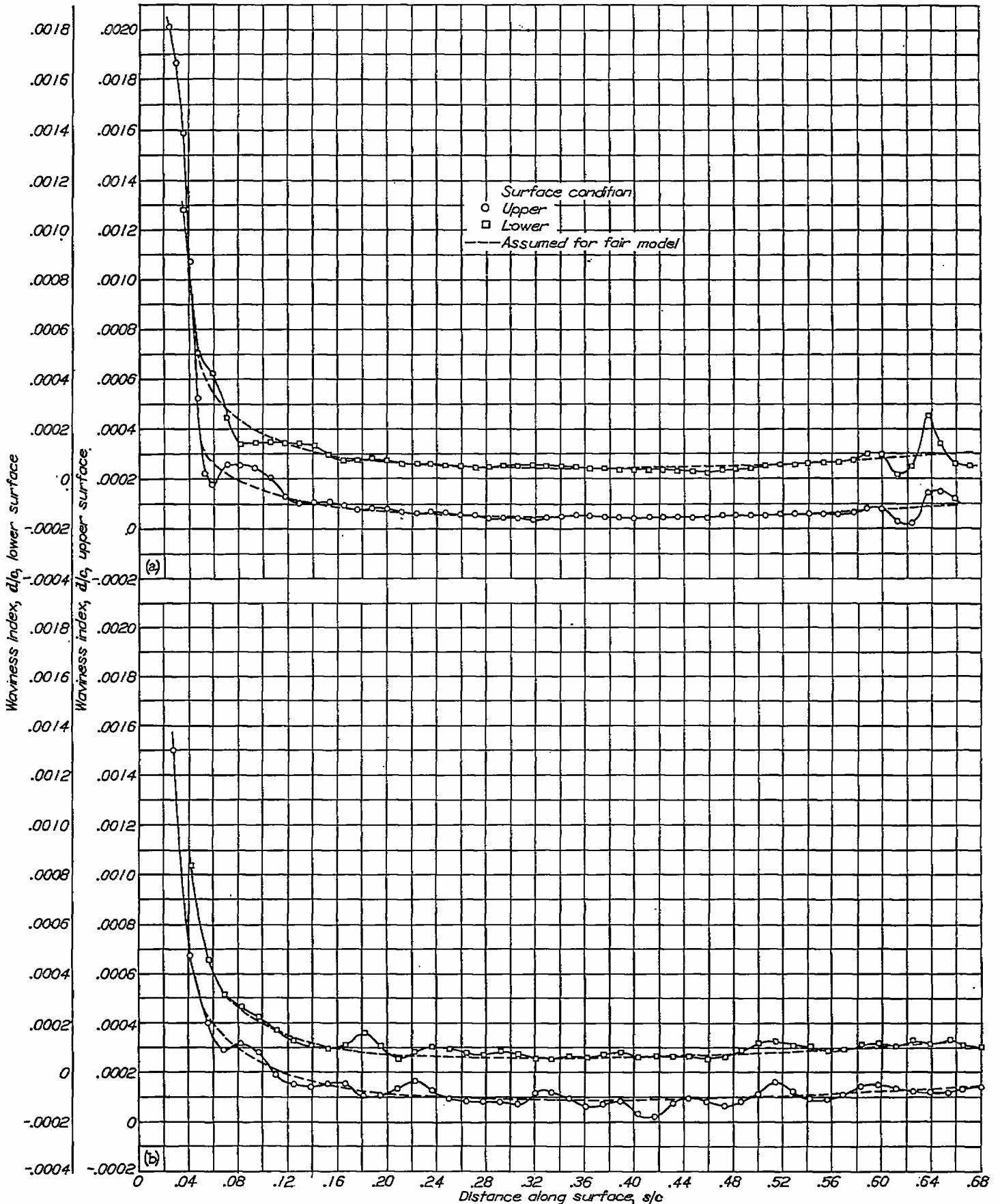
(a) Surface waviness of NACA 66(215)-116 \left\{ \begin{matrix} \alpha=1.0, c_{t_1}=0.2 \\ \alpha=0.8, c_{t_1}=-0.1 \end{matrix} \right\} practical-construction airfoil section. Model 5. (b) Surface waviness of NACA 66(215)-(1.25)16 practical-construction airfoil section. Model 9. FIGURE 17.—Waviness characteristics of some smooth NACA 6-series practical-construction airfoil sections.
