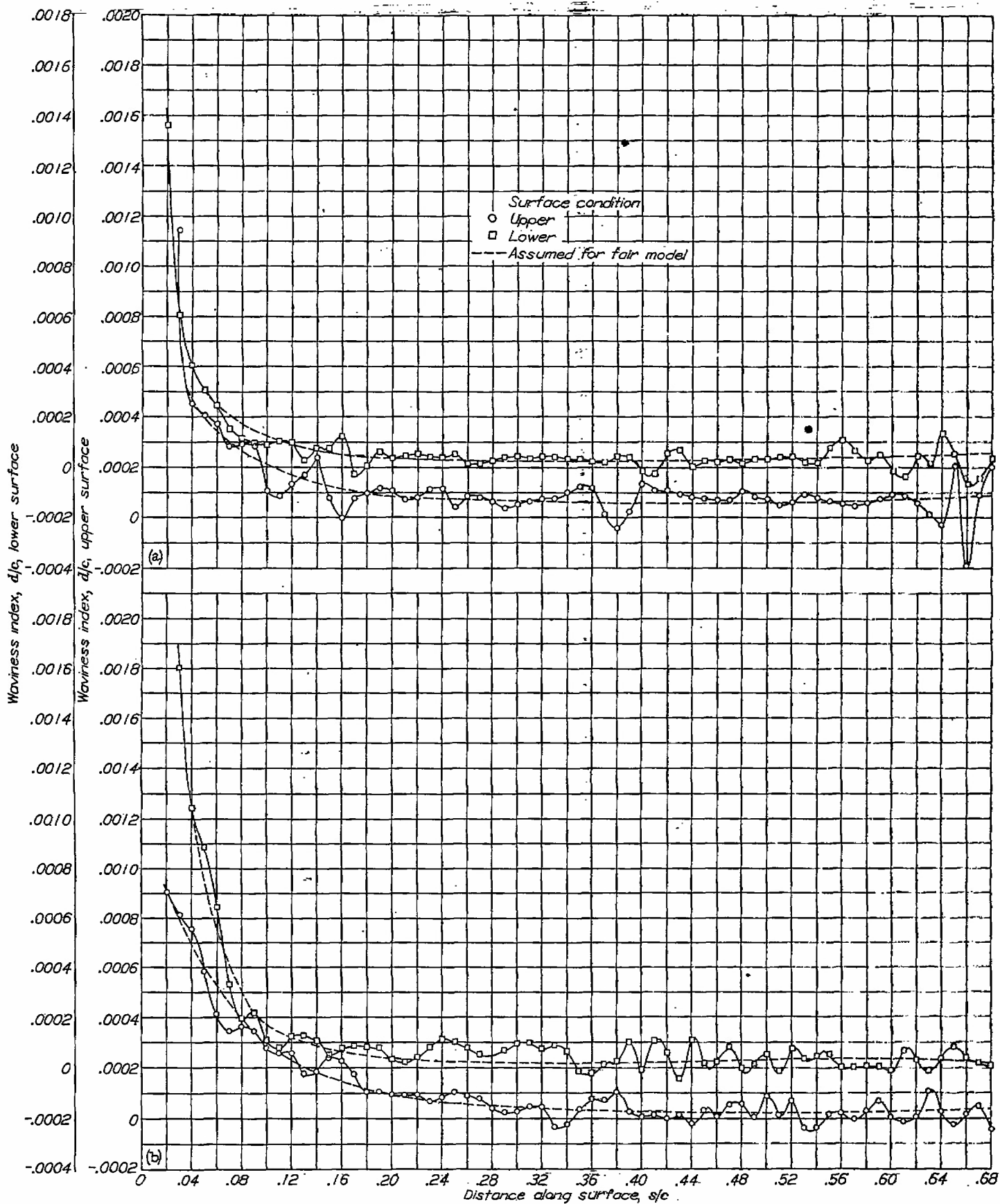
(a) Surface waviness of NACA 23015 (approx.) practical-construction airfoil section, Model 12.
