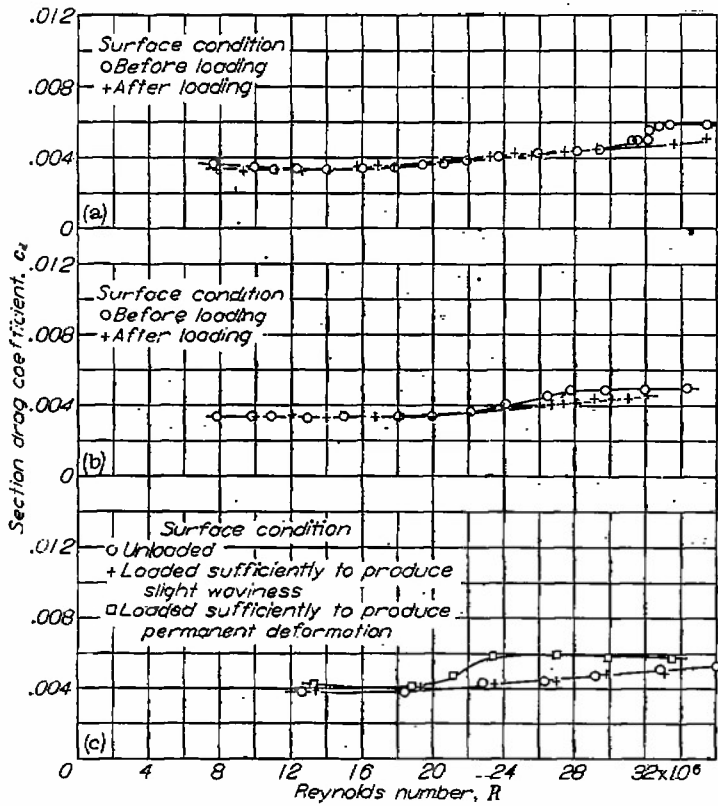
(a) NACA 66(215)-(1.25)16 airfoil section with chordwise hat-section stiffeners spaced 8 inches on centers. c_1=0.14 . Model 9. (b) NACA 66(215)-(1.25)16 airfoil section with chordwise hat-section stiffeners spaced 6 inches on centers. c_1=0.16 . Model 14. (c) NACA 65(216)-215 (approx.) airfoil section. c_1=0.3 . Model 15. FIGURE 28.—Effect of compressive load on drag characteristics of airfoils.
