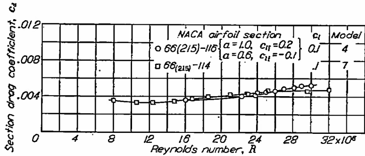
FIGURE 22.—Drag of NACA 66(215)-116 practical-construction airfoil section, surfaces painted and glazed, compared with drag of faired NACA 66(215)-114 practical-construction airfoil section.
