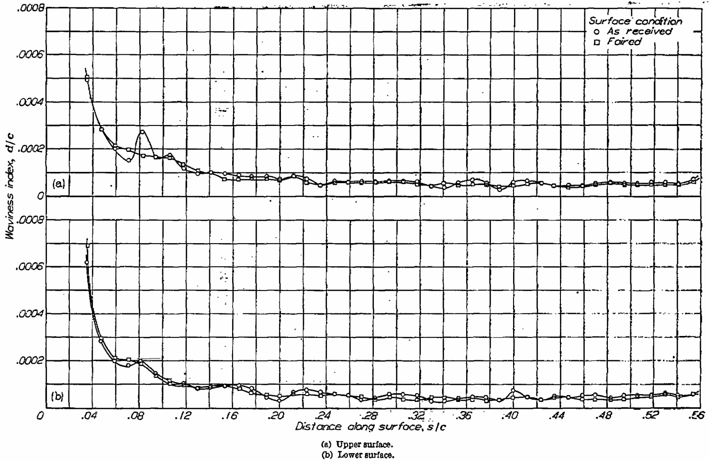
FIGURE 11.—Waviness characteristics of NACA 66(2x15)-114 practical-construction airfoil section in as-received condition and in faired condition. Model 7.
