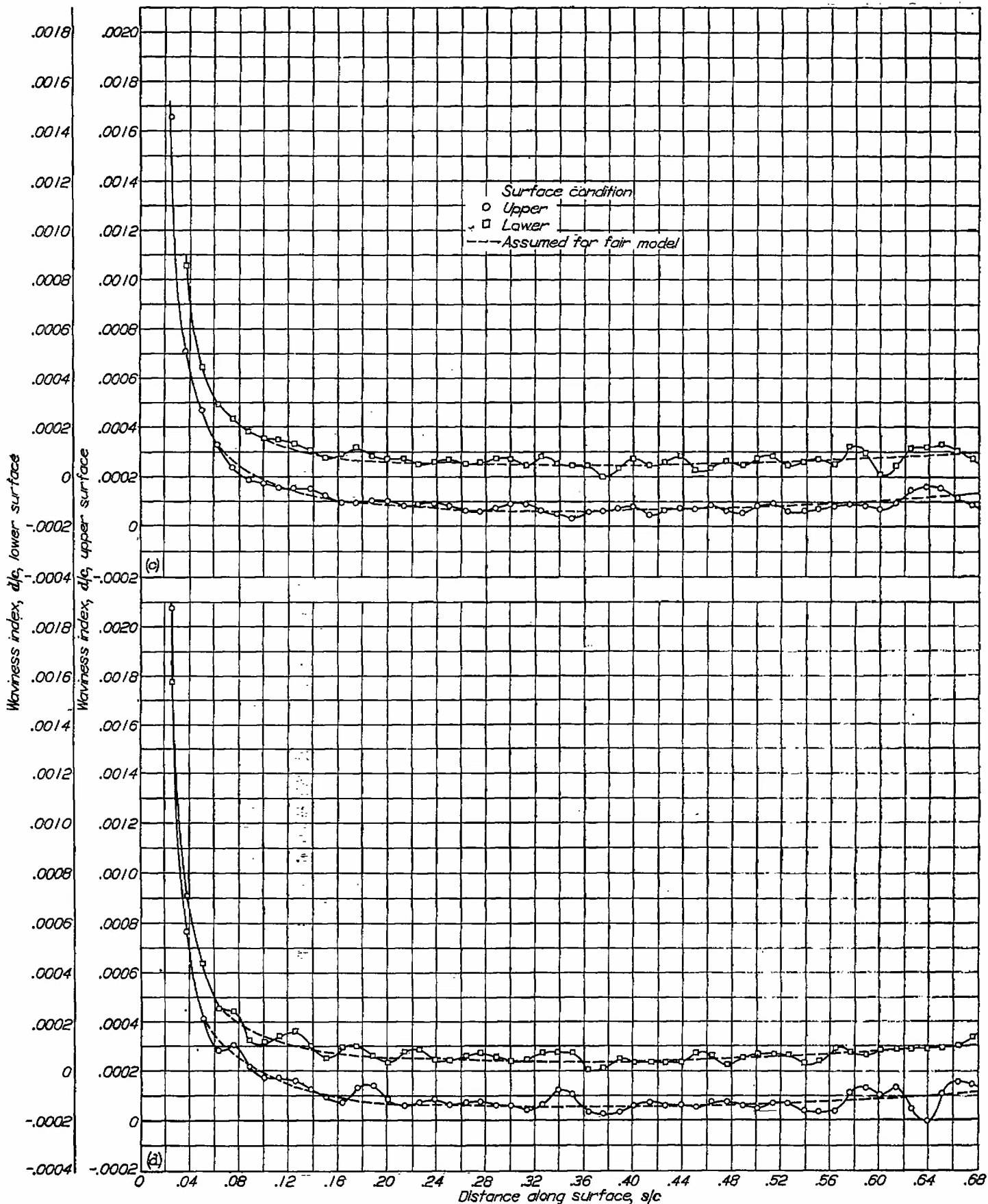
(c) Surface waviness of NACA 66,2-115 practical-construction airfoil section. Model 10.
