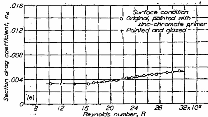
(e) Model 5, NACA 66(215)-116 \left\{ \begin{matrix} \alpha=1.0, c_l=0.2 \\ \alpha=0.6, c_l=-0.1 \end{matrix} \right\} airfoil section. c_l=0.1 .
