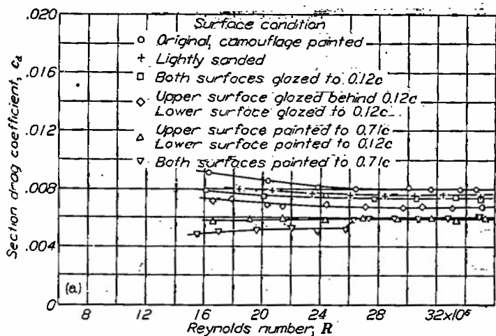
(a) Model 1, NACA 65(216)-3(18.5) (approx.) airfoil section. c_l=0.2 .
