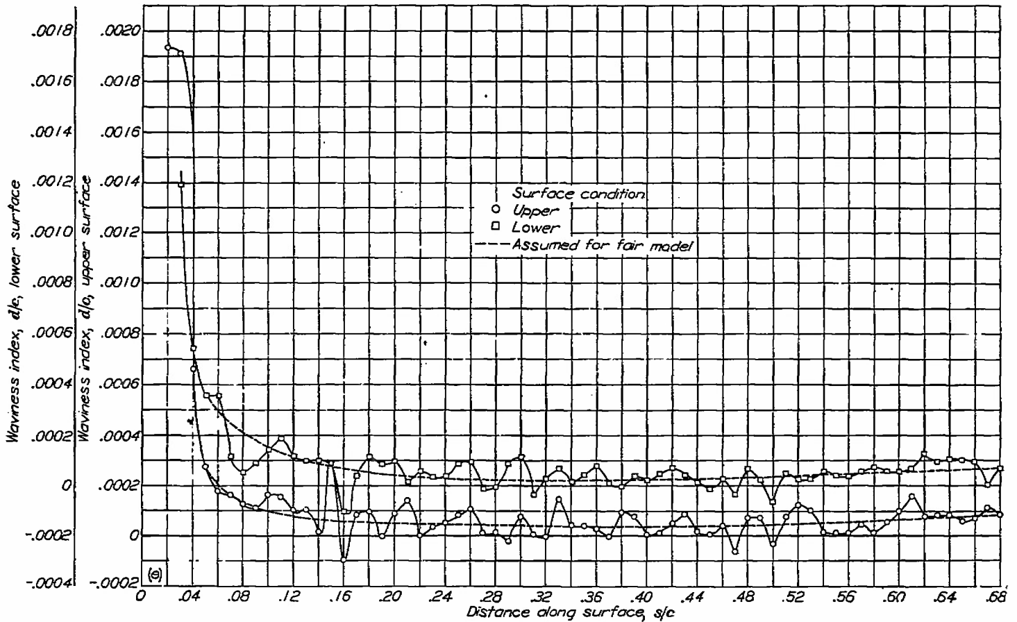
(e) Surface waviness of NACA 65(215)-116 practical-construction airfoil section Model 6. FIGURE 17.—Concluded.
