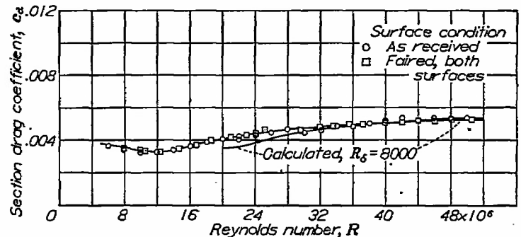
FIGURE 10.—Experimental and calculated section drag characteristics for NACA 66 (215) -114 practical-construction airfoil section. c_l=0.1 (approx.). Model 7.
