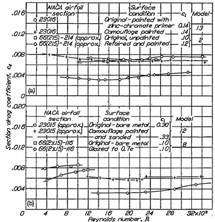
(a) NACA 23016 and 66(215)-214 (approx.) airfoil sections. (b) NACA 23015 (approx.) and 66(2x15)-116 airfoil sections.
