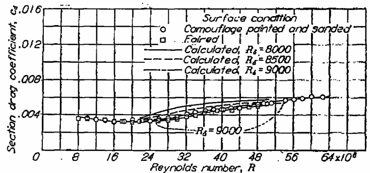
FIGURE 13.—Comparison of experimental and calculated drag-scale-effect curves for NACA 66(2x15)-116 practical-construction airfoil section. c_r=0.1 . Model 8.
