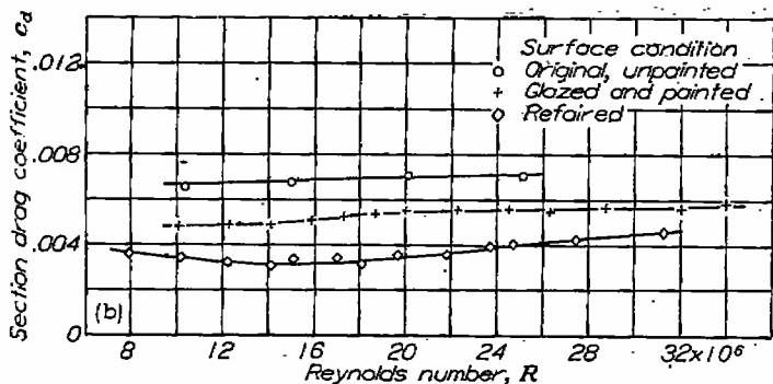
(b) Model 2, NACA 66(215)-214 (approx.) airfoil section. c_l=0.13 .
