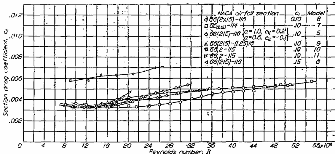
FIGURE 18.—Drag characteristics of some smooth NACA 6-series practical-construction airfoil sections.
