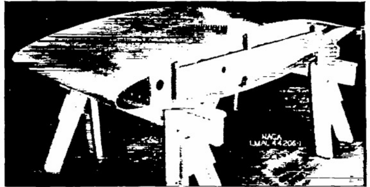
FIGURE 9.—Three-quarter front view of upper surface of NACA 66 (215) -114 airfoil section in as-received condition. Model 7
