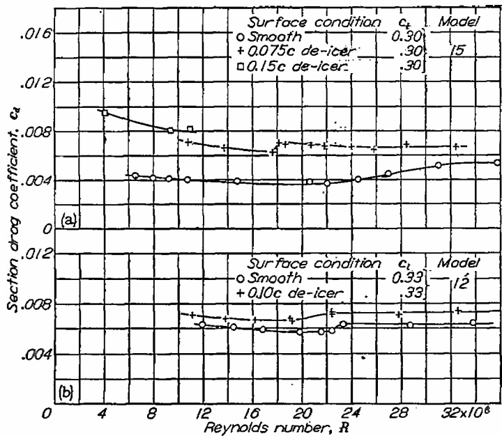
(a) 0.075c and 0.15c de-icer boots on NACA 65(216)-215 (approx.) airfoil section. (b) 0.10c de-icer boot on NACA 23015 (approx.) airfoil section. FIGURE 29.—Effect of de-icer boots on drag characteristics of airfoil sections.
