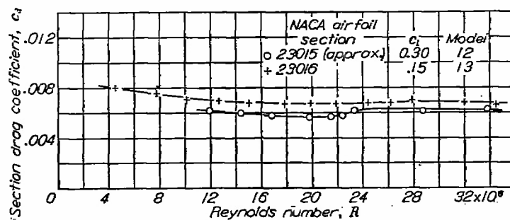
FIGURE 20.—Drag characteristics of some smooth 230-series practical-construction airfoil sections with some surface waviness.
