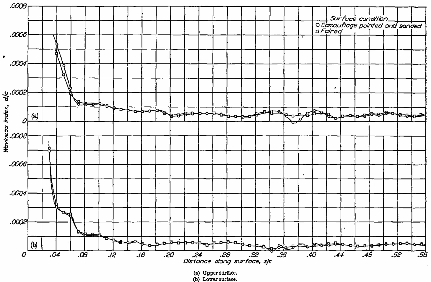
FIGURE 14.—Waviness characteristics of NACA 66(2x15)-116 practical-construction airfoil section before and after fairing process. Model 8.
