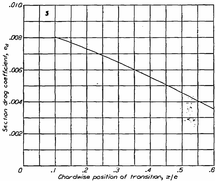
FIGURE 1.—Calculated variation of section drag coefficient with position of transition on NACA 66(na)-116 airfoil section. c_l=0.1 ; R=20 \times 10^6 .
