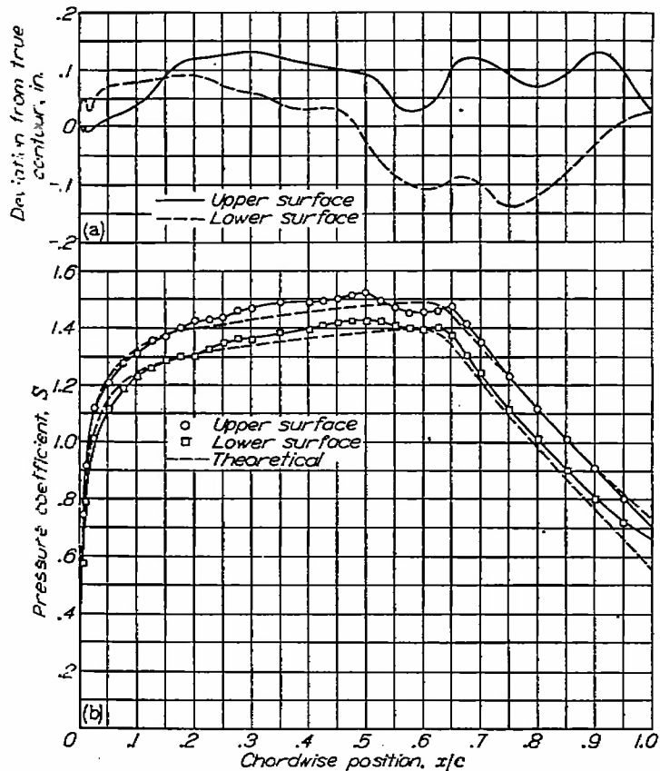
(a) Surface unfairness, painted and glazed condition. (b) Pressure distribution, c_f \approx 0.1 .
