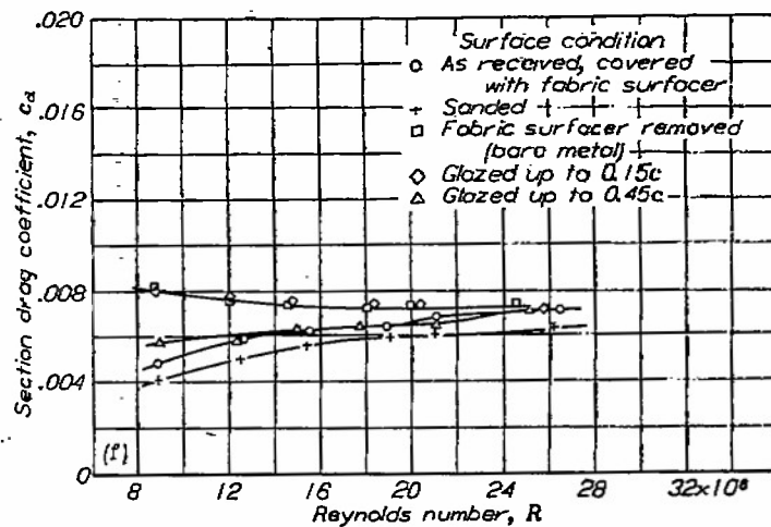
(f) Model 6, NACA 66(215)-116 practical-construction airfoil section. c_l=0.15 (approx.).
