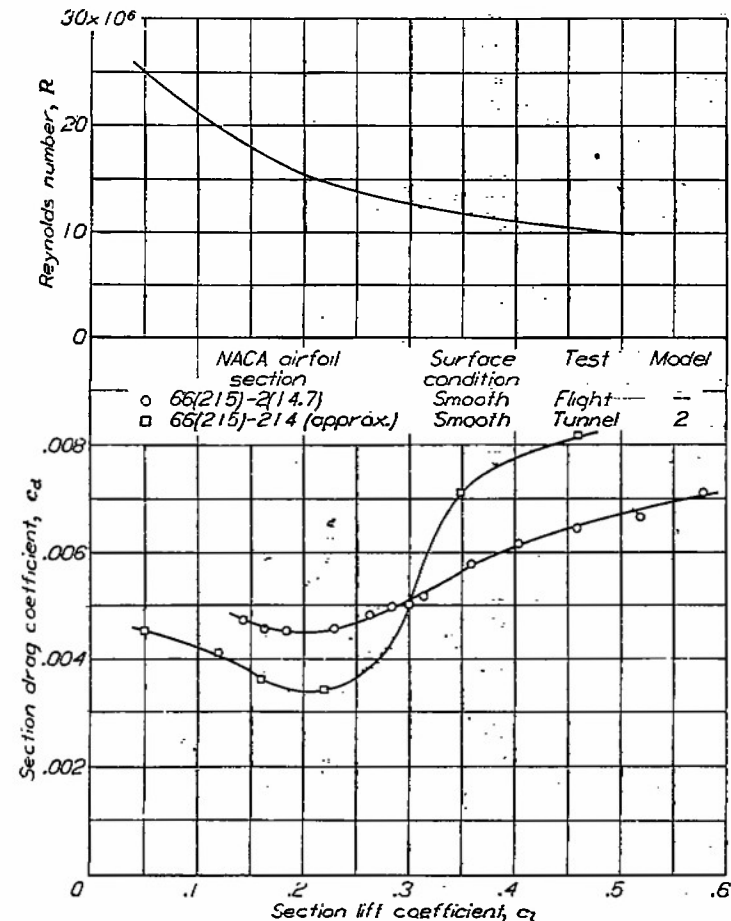
FIGURE 25.—Comparison of drag characteristics of smooth test panel of airplane wing with that of smooth practical-construction wing model.
