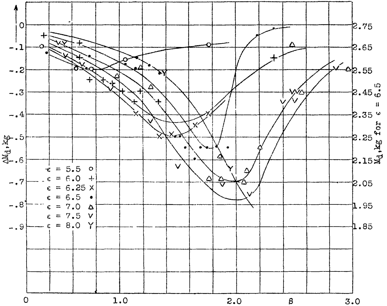
Figure 24.- Free torque curves ( \Delta M_d ) against \beta , for Fig. 5. Fuel No. 3. (octane rating 87)
