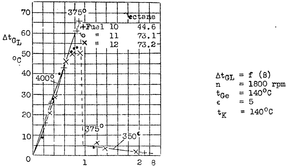
Figure 13.- Behaviour of Fuel No. 10 (44-6 octane rating, I.G. standard reference petrol): and Fuel No.10 with the addition of tetraethyl lead (Fuel No.11, 73.1 octane, and No.12, 73.2 octane).
