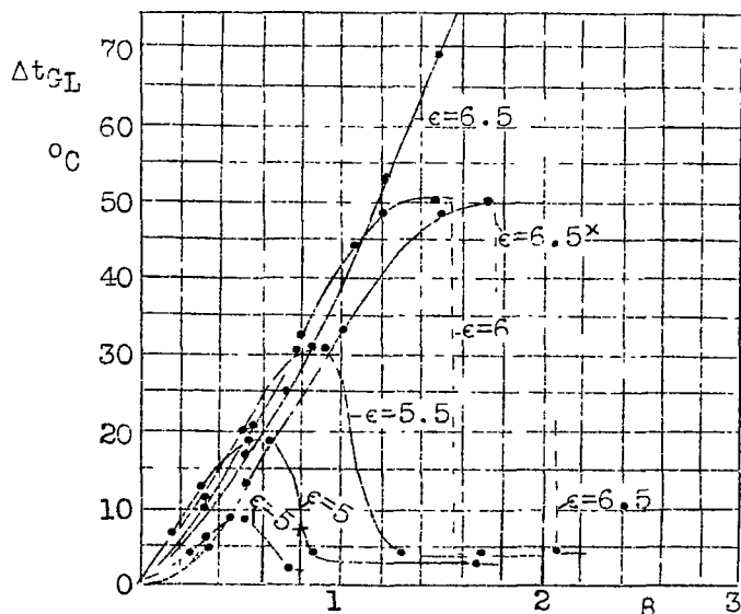
Figure 12.- Behaviour of Fuel 2. (72-octane rating), for \epsilon = 6.5^x and \epsilon = 5^x - Fuel No.13 (87.8 - octane rating) prepared from Fuel No.2 by the addition of 1.3 \text{ cm}^2 ethyl fluid per litre.
