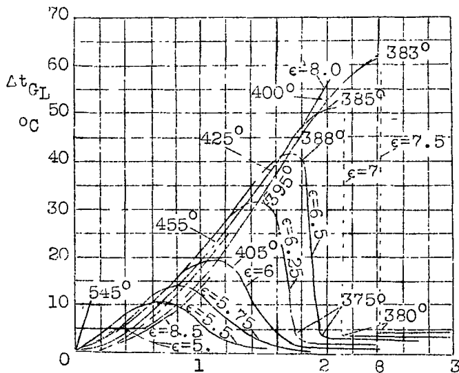
Figure 5.- Behaviour of Fuel No.3 (Aviation Spirit, rated 87-octane). (octane rating 87)
