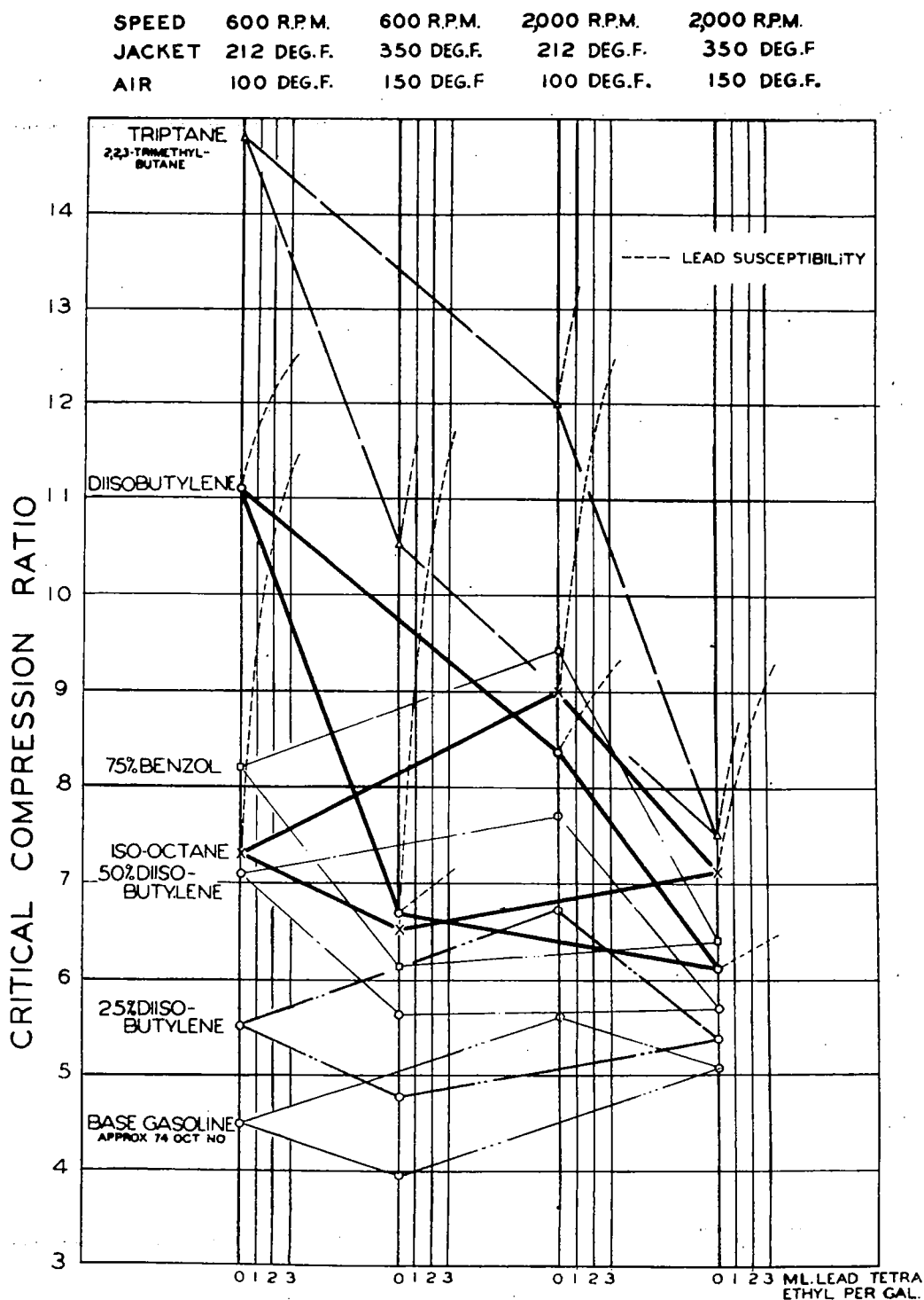
Fig. 31.-Variation in critical compression ratio of six fuels for four standard test conditions (reference 14 ).
