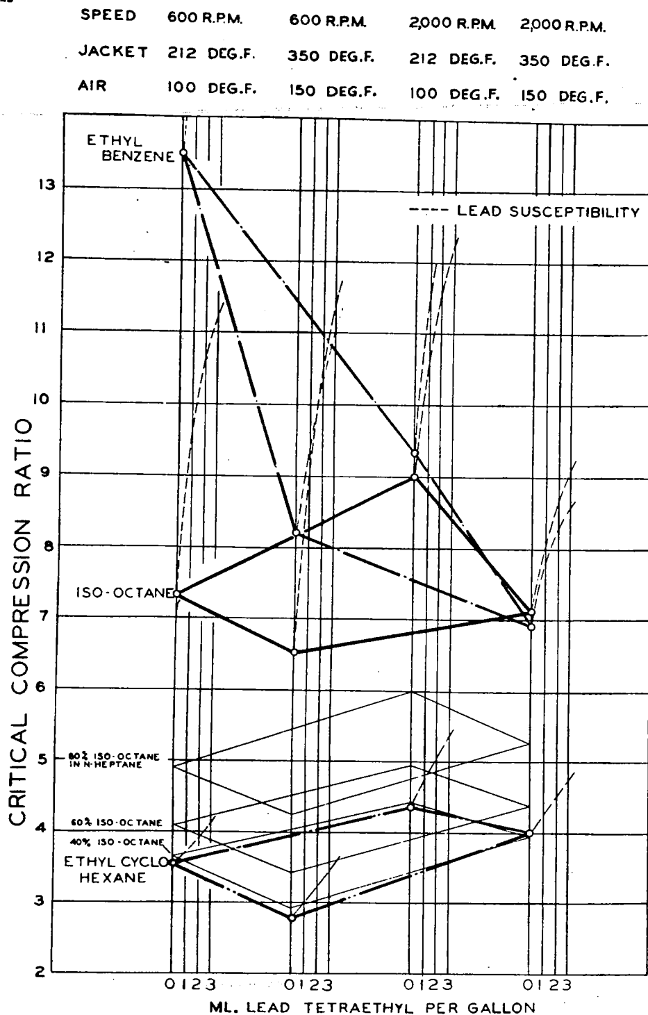
Fig. 32.-Variation in critical compression ratio for four standard test conditions, for ethyl benzene, ethyl cyclohexane, and iso-octane (2, 3, 4-trimethylpentane) (reference 14).
