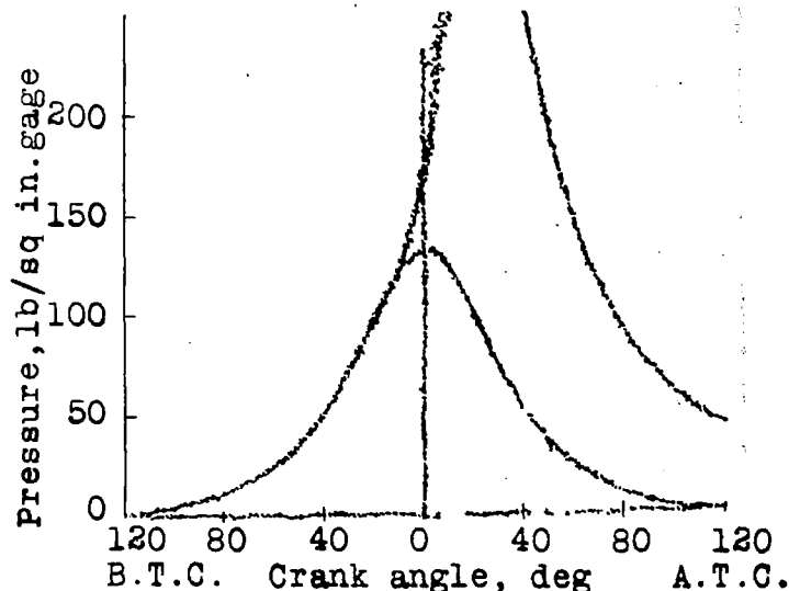
Figure 14.- Composite indicator diagram for run 73.
