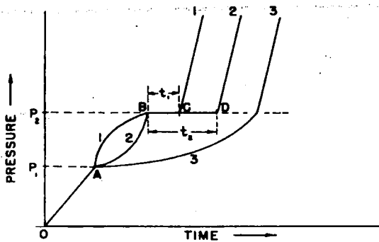
Figure 26. - Effect of path of compression on the value of apparent delay at a given pressure.
