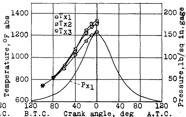
Figure 24.- Temperature and pressure of the unburned charge at various crank angles, run 80. See table XII.
