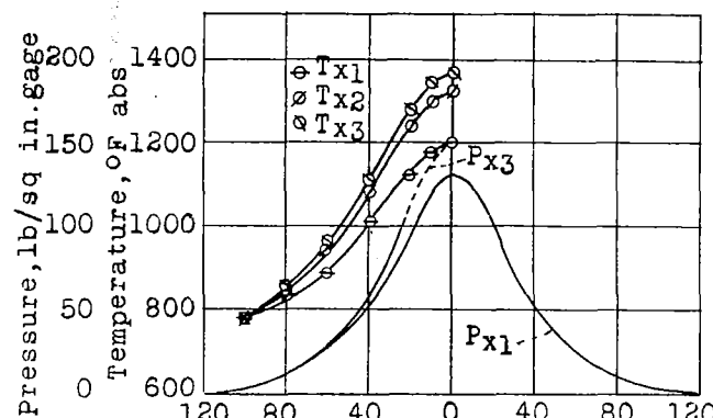
Figure 17.- Temperature and pressure of the unburned charge at various crank angles, computed from 100° B.T.C., run 76. See table V.
