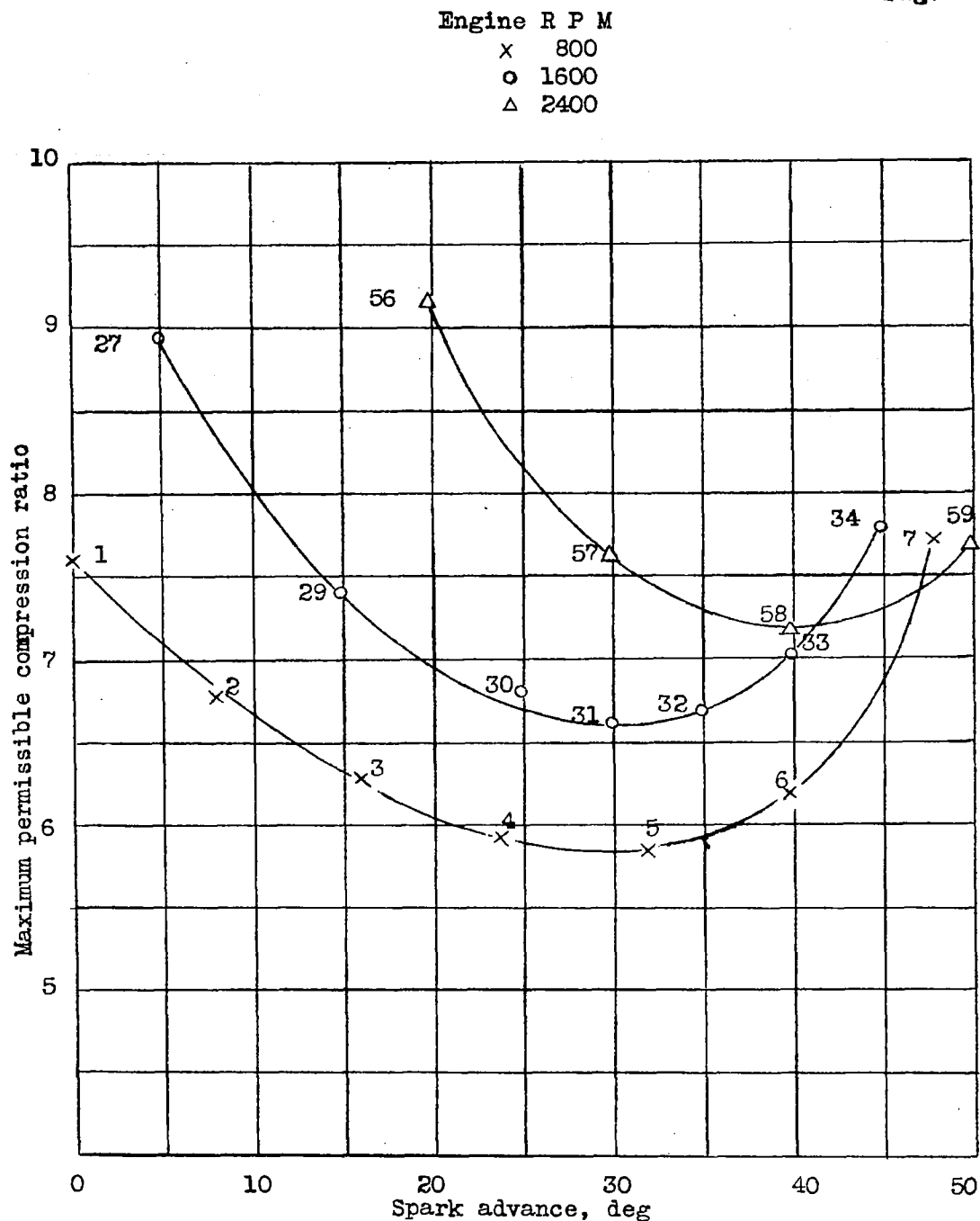
Figure 7- Effect of spark advance and engine speed on maximum permissible compression ratio. C.F.R. engine; inlet mixture temperature, 120°F; fuel 78.9 octane. Numbers on points correspond to runs listed in table 1.
