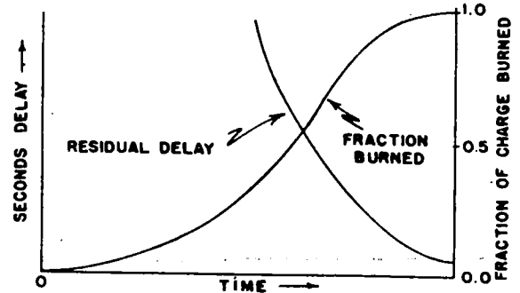
Figure 30. - Effect of flame propagation on residual delay in a non-detonating engine.
