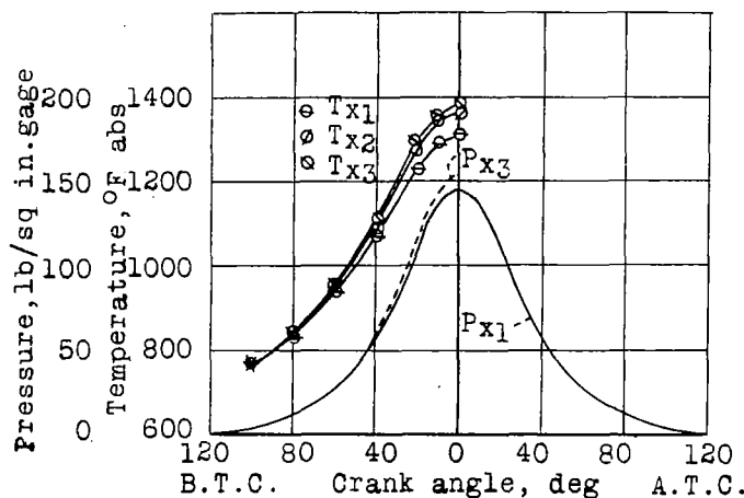
Figure 19.- Temperature and pressure of the unburned charge at various crank angles, run 77a. See table IX.
