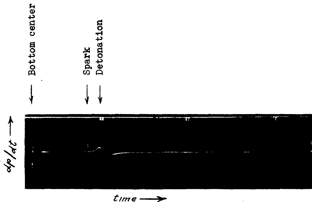
Figure 12. - Specimen \frac{dp}{dt} record for moderate detonation.
