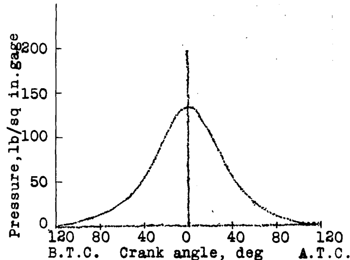
Figure 16.- Indicator diagram for run 76. See table V.
