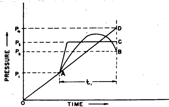
Figure 27. - Effect of path of compression as self-ignition pressure for a constant value of total delay.
