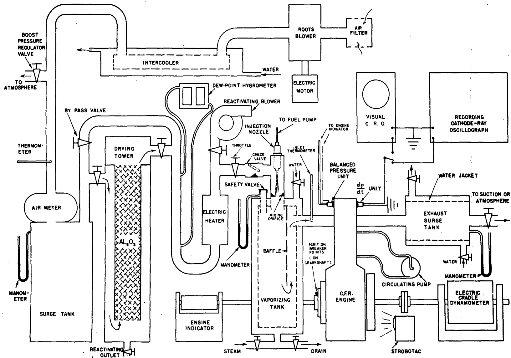
Figure 2. - Schematic diagram of apparatus.
