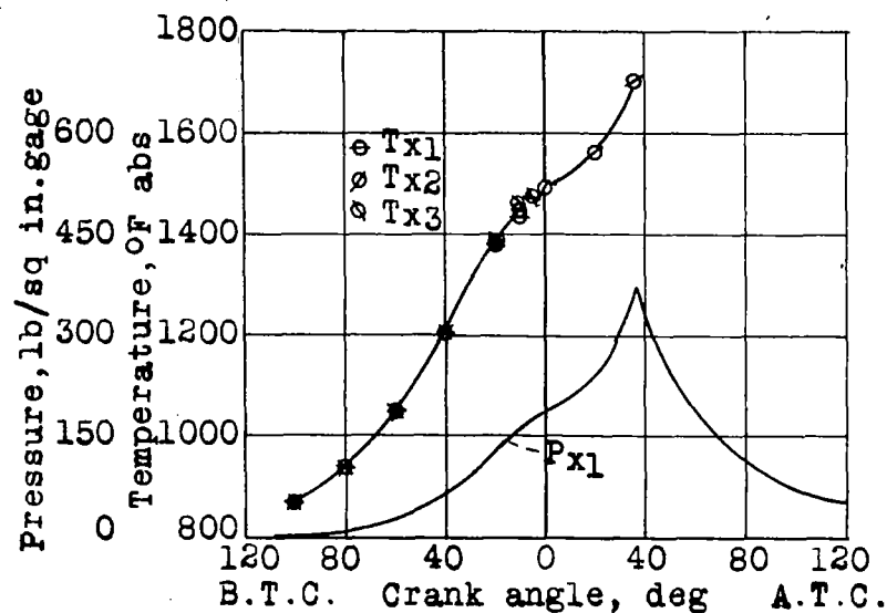
Figure 13.- Temperature of the unburned charge and cylinder pressures at various crank angles, run 27. See table III.
