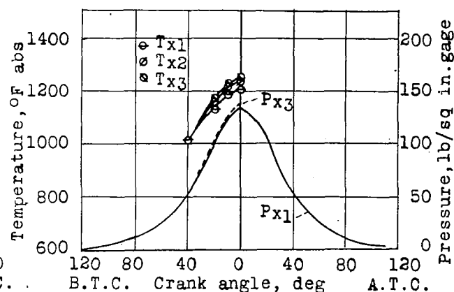
Figure 18.- Temperature and pressure of the unburned charge at various crank angles, computed from 40° B.T.C., run 76. See table V.
