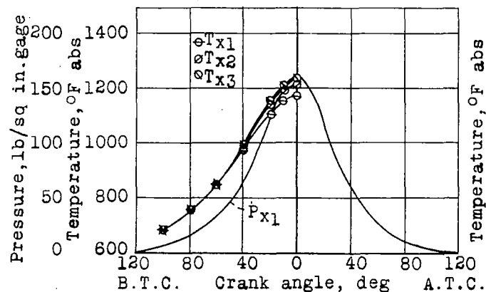
Figure 23.- Temperature and pressure of the unburned charge at various crank angles, run 79. See table XI.
