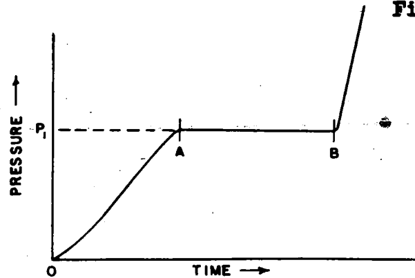
Figure 8. - Pressure-time curve for sudden compression of fuel-air mixture showing apparent delay.
