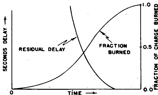
Figure 29. - Effect of flame propagation on residual delay in a detonating engine.
