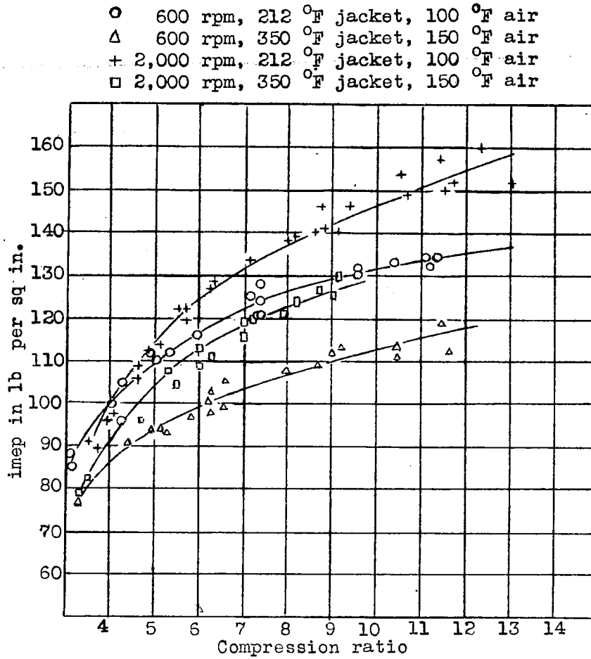
Figure 33.- Indicated mean effective pressure vs. compression ratio for four standard conditions (reference 14).
