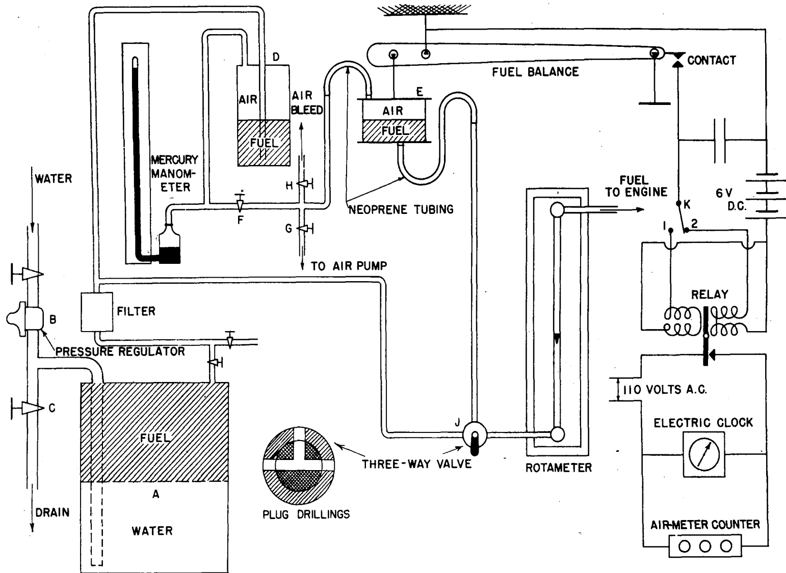
Figure 3. - Schematic diagram of fuel system.
