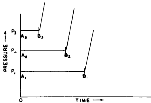
Figure 28. - Pressure-time curves for instantaneous compression of fuel-air mixture showing how absolute delay varies with pressure.
