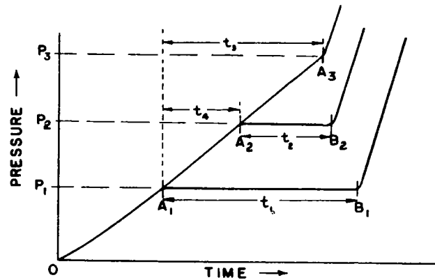
Figure 9. - Pressure-time curves for sudden compression of fuel-air mixture showing how delay varies with pressure.
