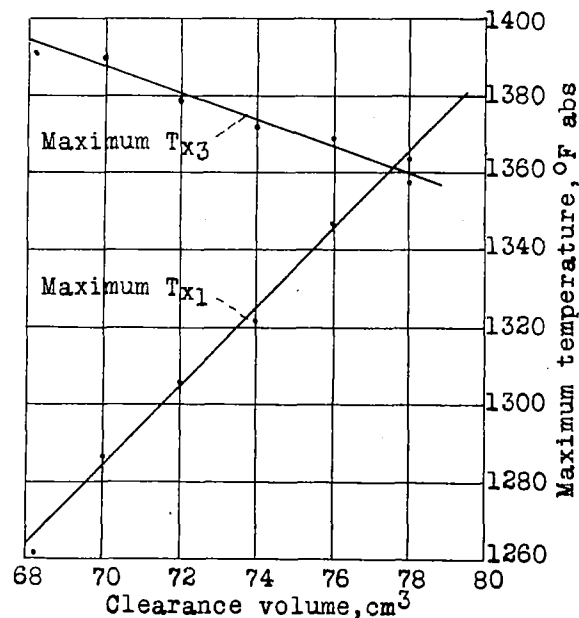
Figure 21.- Effect of clearance-volume errors on maximum values of indicated and adiabatic temperatures, run 77a.
