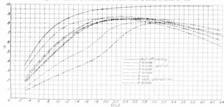
Figure 22.- Comparison of efficiencies for different methods of increasing thrust. C_p = 0.6 .
