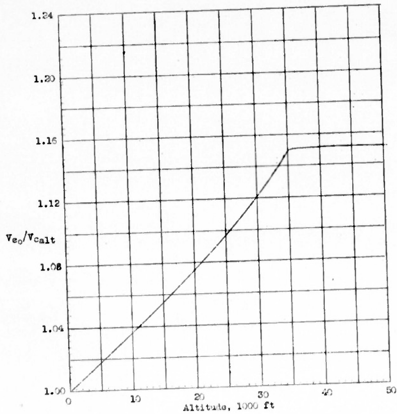
Figure 7.- Variation of ratio \frac{\text{speed of sound at sea level}}{\text{speed of sound at altitude}} with altitude.
