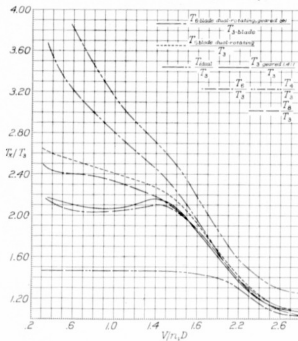
Figure 25.- Comparison of methods for increasing thrust. C_{p1} = 0.6 .
