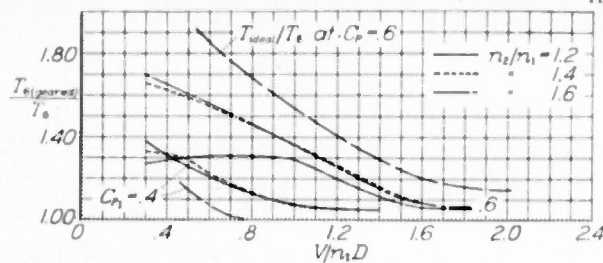
Figure 18.- Effect of two-speed gearing on thrust at low speeds. Six-blade propeller.
