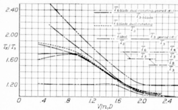
Figure 24.- Comparison of methods for increasing thrust. C_{p1} = 0.4 .
