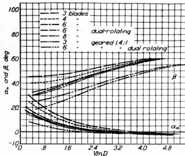
Figure 26.- Variation of \alpha_\infty and \beta with V/nD for several propellers at C_p = 0.4 .
