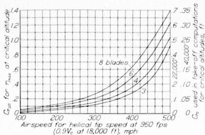
Figure 6.- Variation of C_p for \eta_{max} with airspeed for different propeller efficiencies.
