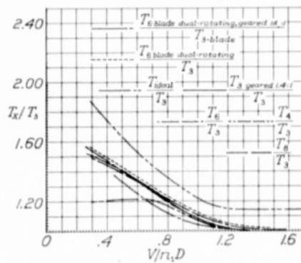
Figure 23.- Comparison of methods for increasing thrust. C_p = 0.2 .
