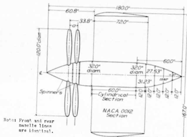
Figure 4.- Plan view showing dimensional details of wing and nacelle. Dimension a for four-blade propeller = 9.7" and for six and eight blade propeller = 10.0".
