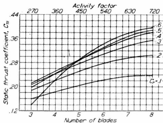
Figure 27.- Variation of static thrust with solidity.
