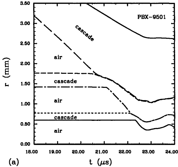
Fig. 3. Cascade radii (a) and velocity (b) for PBX-9501 simulations using the mixed EOS. Calculated field (MG) is overlaid in (b).
