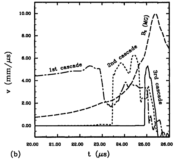
Fig. 2. Cascade radii (a) and velocity (b) for Comp-B simulations using the mixed EOS. Calculated field is overlaid in (b).
