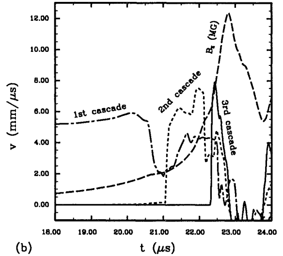
Fig. 3. Cascade radii (a) and velocity (b) for PBX-9501 simulations using the mixed EOS. Calculated field (MG) is overlaid in (b).
