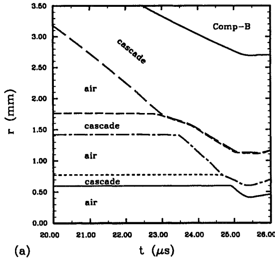
Fig. 2. Cascade radii (a) and velocity (b) for Comp-B simulations using the mixed EOS. Calculated field is overlaid in (b).
