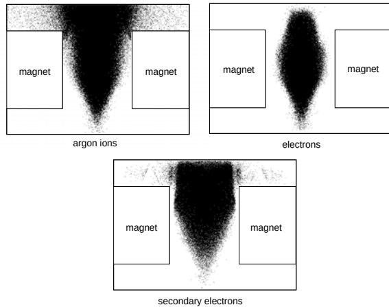
Figure 6. Particle distributions in z-r space for a) argon ions; b) electrons from the ionization of argon neutrals by secondary electrons; c) secondary electrons emitted from the three ground conducting surfaces.
