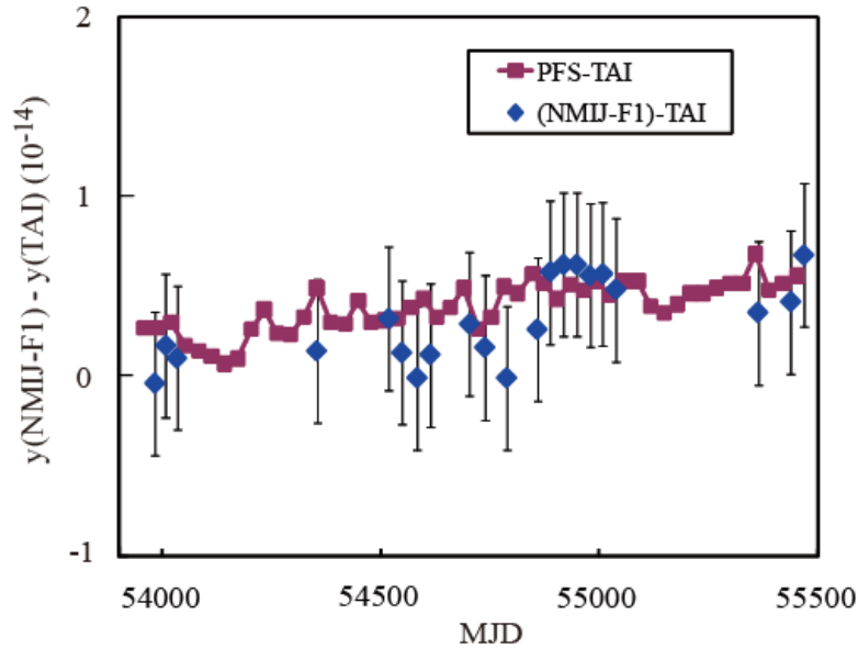
Figure 2. The long-term data of NMIJ-F1 reported to BIPM.
