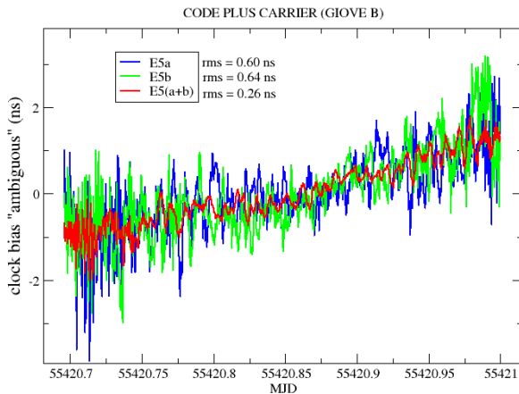
Figure 6. Comparison between the CPC clock solutions for station GNOR, obtained with 30-second data and with E5a, E5b or E5(a+b).
