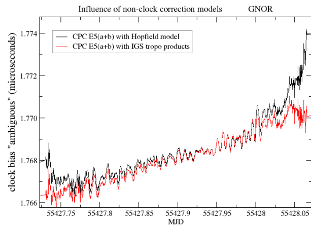
Figure 7. Comparison between the CPC clock solutions obtained with tropospheric corrections from the Hopfield model or with the IGS troposphere products.
